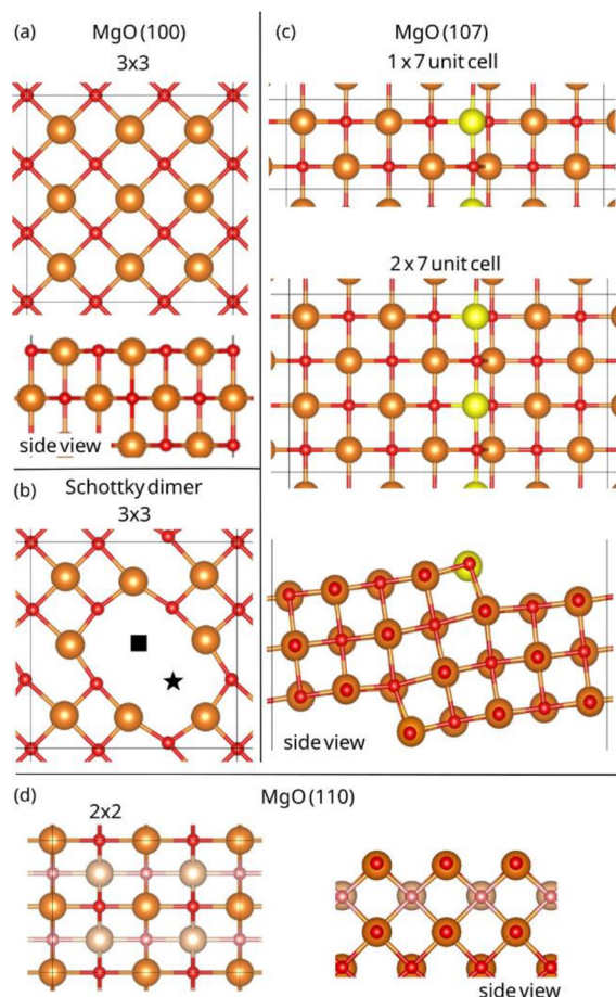
FIGURE 3 | Surface models employed in the DFT calculations. (a) Pristine MgO(100) terrace represented by a slab model using a (3 × 3) supercell (top and side views). (b) MgO(100) slab with (3 × 3) surface periodicity containing a Schottky dimer defect, consisting of adjacent Mg and O vacancies (top view). (c) Stoichiometric MgO(107) stepped slabs exposing monoatomic step edges, shown for (1 × 7) and (2 × 7) surface supercells (top views). (d) Stoichiometric MgO(110) surface (top and side views). For clarity, the top views in (a) and (d) display only the outermost surface layer of the slab. Color code: fivefold-coordinated surface Mg ( \text{Mg}_{5c}^{2+} ) in orange, fourfold-coordinated Mg ( \text{Mg}_{4c}^{2+} , characteristic of step-edge sites) in yellow, and O in red. For the MgO(110) model in (d), Mg and O atoms in the second layer are displayed in lighter shades to distinguish them from the outermost surface layer. Mg vacancies are indicated by black squares and O vacancies by black stars. This color scheme is used consistently throughout all figures in this paper.
