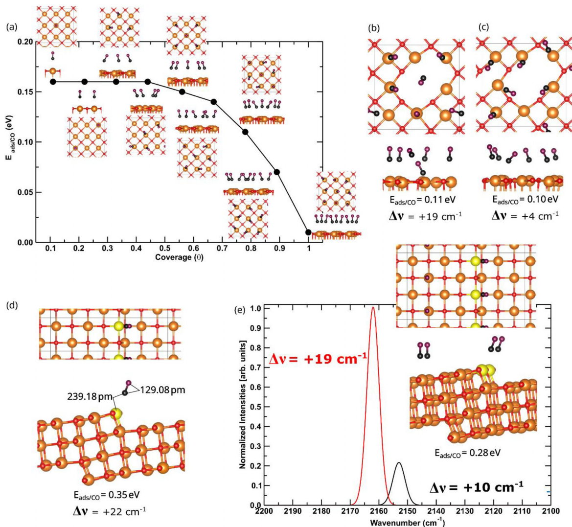
FIGURE 4 | (a) Coverage dependence of the average adsorption energy per CO molecule, |E_{\text{ads/CO}}| , on MgO(100) computed at the PBE level; optimized structures corresponding to selected coverages are shown as insets ( 3 \times 3 cell). (b,c) Top and side views of representative ordered CO adlayers on a Schottky dimer model at \Theta = 2/3 ML, together with the computed adsorption energies ( E_{\text{ads/CO}} ) and C–O stretching-frequency shifts, \Delta\nu , relative to gas-phase CO. (d) Optimized geometry of a strongly bound CO species at an MgO step site, highlighting the Mg–C and C–O bond lengths and the corresponding E_{\text{ads/CO}} and \Delta\nu ( 1 \times 7 cell). (e) Simulated IR spectra for CO at step-edge (red) and terrace sites (black), illustrating the characteristic positive frequency shifts associated with step-edge and terrace adsorption configurations ( 2 \times 7 cell). Adsorption energies and vibrational frequency shifts shown in panels (b–e) are computed at the HSE06 level. Color code: C atoms of CO are shown in black and O atoms of CO in violet.
