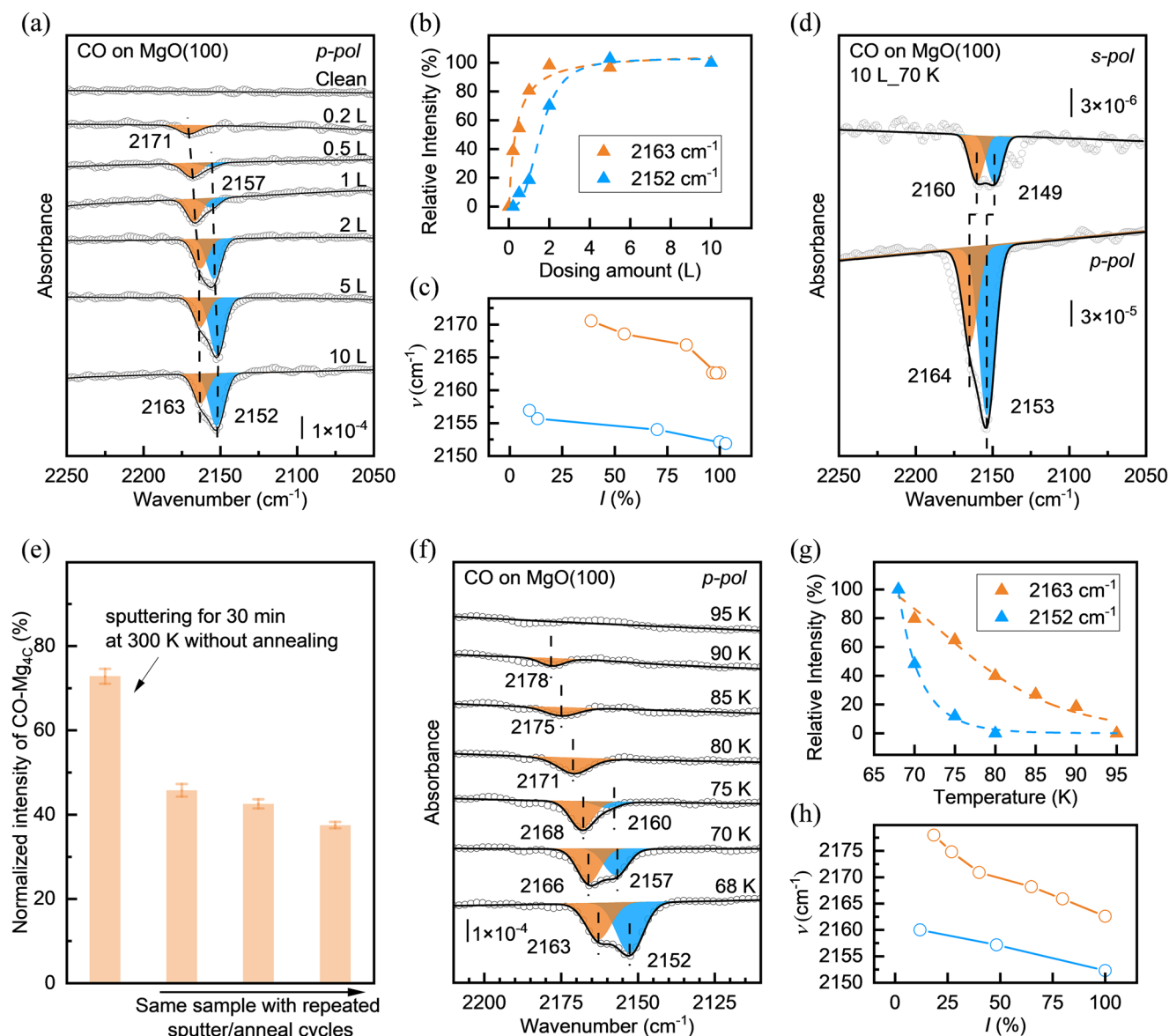
FIGURE 1 | Polarization-resolved IRRAS data for CO adsorption on MgO(100) single crystal surfaces. (a) Deconvoluted coverage-dependent IRRAS spectra recorded with p -polarized light at 67 K. (b) Integrated intensities of the CO bands as a function of CO dose. (c) Vibrational frequency shifts of the two CO bands as a function of relative band intensity. (d) Deconvoluted p - and s -polarized IRRAS spectra acquired after CO exposure (10 L) on MgO(100) at 70 K. (e) Relative intensity of the defect-related high-frequency CO band ( \sim 2165\text{ cm}^{-1} ), defined as the ratio of the peak area of the 2165\text{ cm}^{-1} band to the total peak area of both CO bands, as a function of surface preparation by successive sputtering (10 min at 300 K) and annealing (15 min at 850 K in 1 \times 10^{-6} mbar \text{O}_2 ) cycles. (f–h) Temperature-dependent IRRAS data for CO desorption from MgO(100): (f) Deconvoluted p -polarized IRRAS data recorded after CO adsorption (10 L) at 68 K and subsequent annealing to the indicated temperatures. (g) Integrated intensities of the CO bands associated with \text{Mg}_{\text{sc}}^{2+} terrace sites and \text{Mg}_{4\text{c}}^{2+} defect sites as a function of sample temperature, used for Redhead-type analysis of adsorption energies. (h) Vibrational frequency shifts of the CO bands as a function of relative band intensity during the desorption process. All spectra were measured at a grazing incidence angle of 80^\circ under UHV conditions (base pressure 8 \times 10^{-11} mbar).
