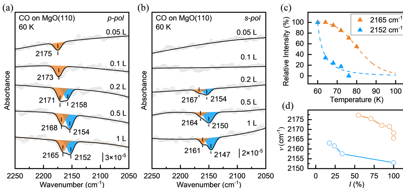
FIGURE 2 | (a,b) Deconvoluted polarization-resolved IRRAS data for CO adsorption on MgO(110) at 60 K as a function of CO dose: (a) p -polarized IRRAS spectra; (b) s -polarized IRRAS spectra. (c,d) Temperature-dependent IRRAS data for CO desorption from MgO(110) recorded after CO adsorption (1 L) at 60 K and subsequent annealing to the indicated temperatures. (c) Integrated intensities of the distinct CO bands as a function of sample temperature, used for Redhead-type analysis of adsorption energies. (d) Vibrational frequency shifts of the CO bands as a function of relative band intensity during the desorption process. All spectra were collected at a grazing incidence angle of 80° along the [001] azimuth. The small frequency offset ( \sim 4 cm -1 ) between s - and p -polarized spectra arises from the dielectric response of the substrate and is intrinsic to IRRAS on insulating surfaces [58].
