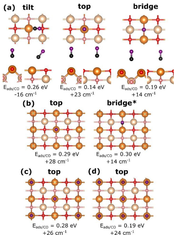
FIGURE 5 | Optimized adsorption geometries (top and side views) for the stable local minima obtained at different coverages \theta on MgO(110). (a) At \theta = 1.0 ML, three adsorption motifs are identified: tilt, top, and bridge configurations. (b) At \theta = 0.25 ML, only on-top and a slightly tilted bridge* minimum remain stable. (c,d) At intermediate coverages \theta = 0.50 ML (c) and \theta = 0.75 ML (d), the calculations converge to a single stable on-top configuration.
