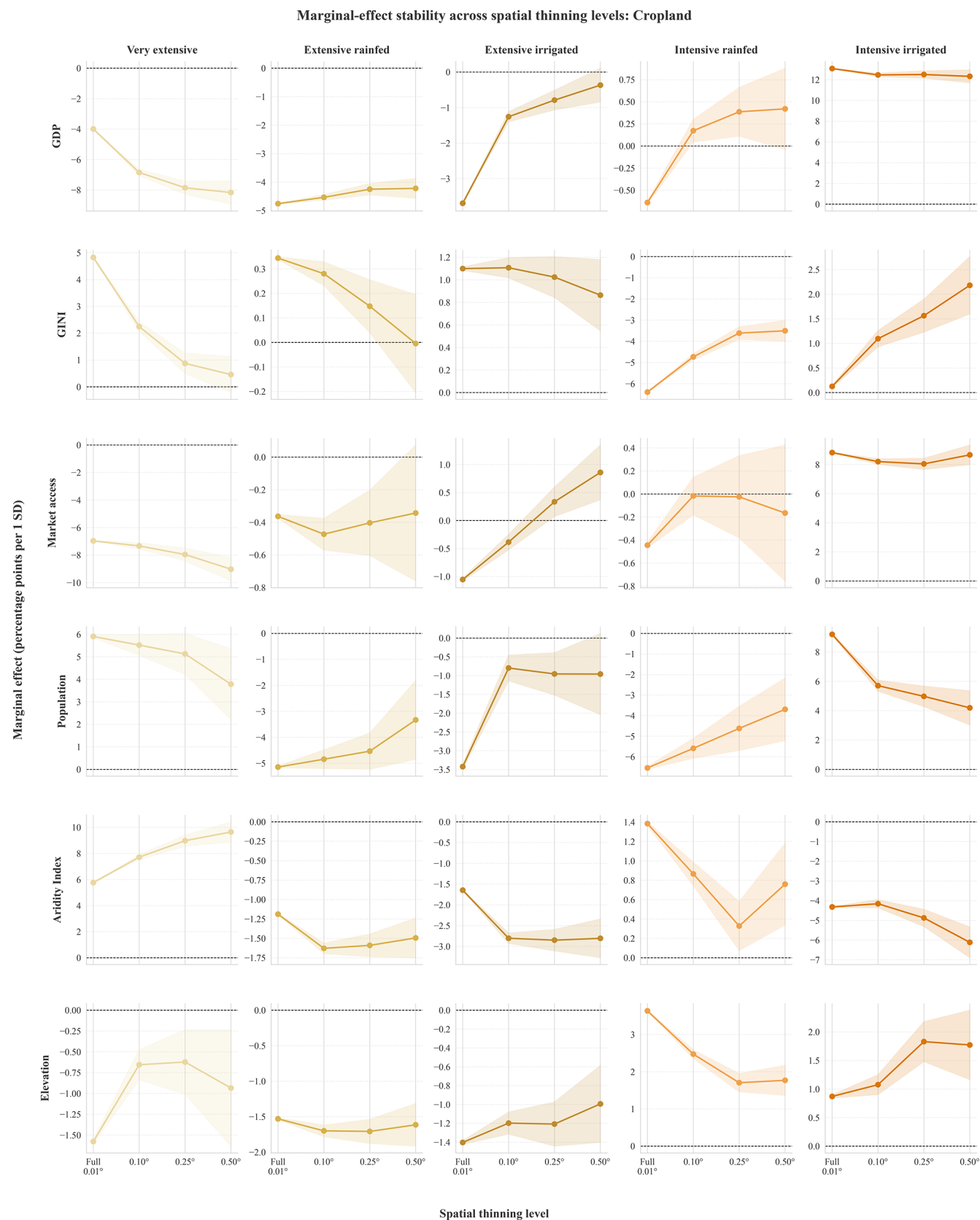
Figure A10. Spatial thinning robustness analysis of marginal effects for cropland management intensity classes. Marginal effects were recalculated using progressively coarser spatial samples (0.10, 0.25, and 0.50°). Lines show marginal effects for each thinning level relative to the full-resolution model (0.01°), while shaded areas indicate confidence intervals.
