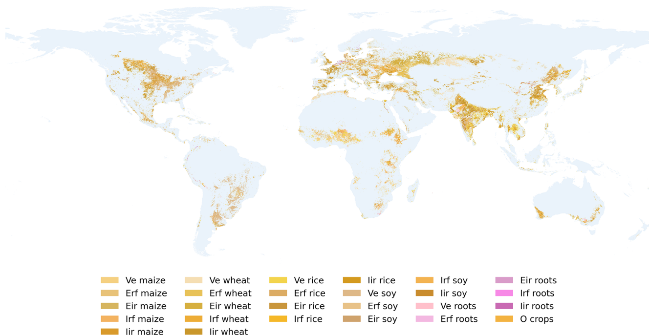
Figure A2. Global cropland management intensity. Cropland management categories included very extensive (Ve), extensive rainfed (Erf), extensive irrigated (Eir), intensive rainfed (Irf), intensive irrigated (Iir). Roots include tubers and potatoes, and “O” refers to “other crops”.
