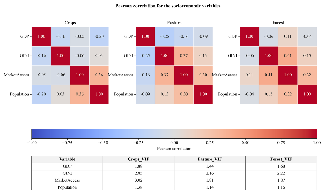
Figure A6. Multicollinearity check using pair-wise regression analysis and the variance inflation factor (VIF) methods for the socioeconomic variables.
