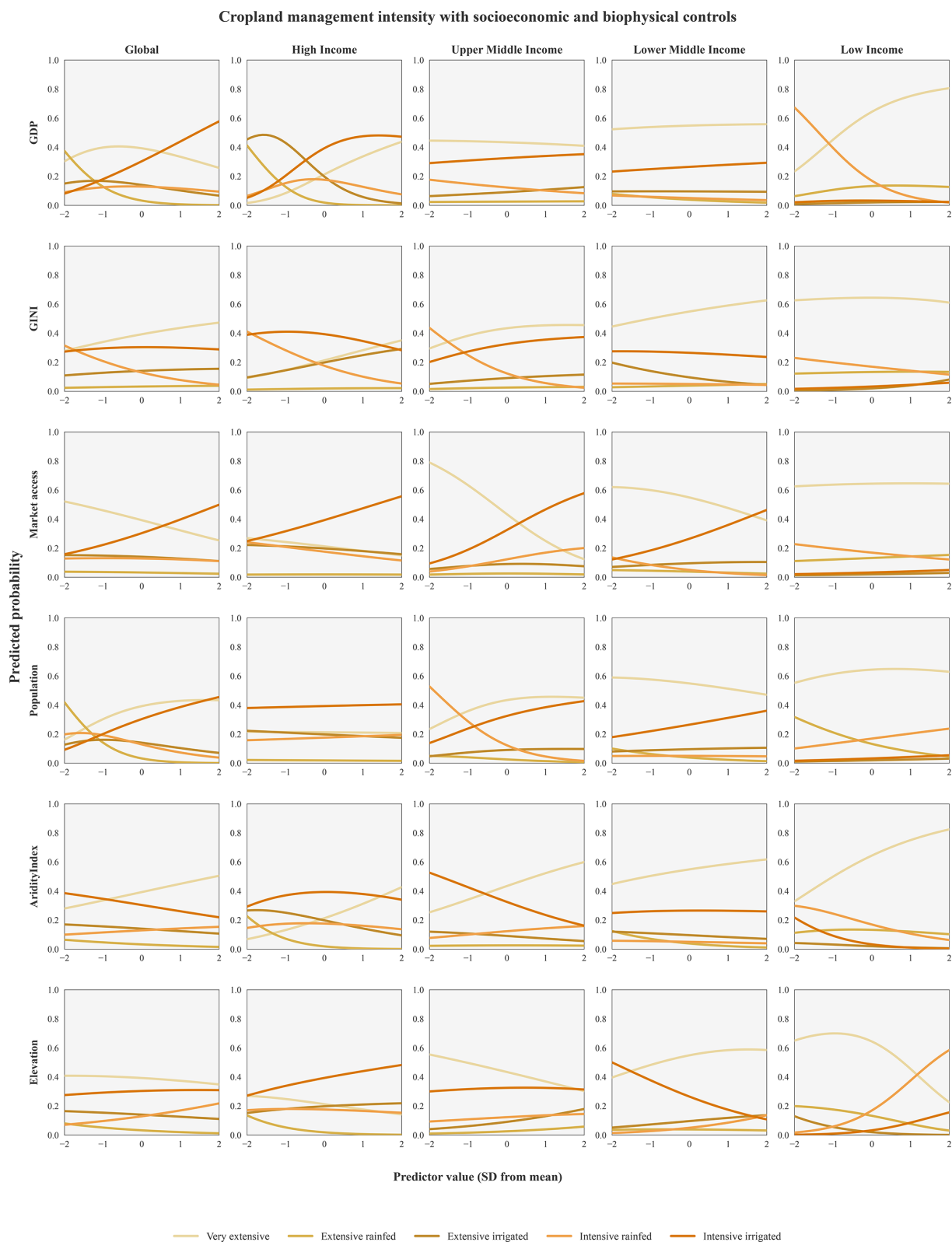
Figure A7. Predicted relationships between crop management intensity and socioeconomic drivers across global income groups. The x -axes of each plot show the standardised predictor value ( z -score) for various variables (GDP, GINI, market access, and population), and the y -axes indicates the predicted probability of each management intensity (very extensive, extensive, and intensive).
