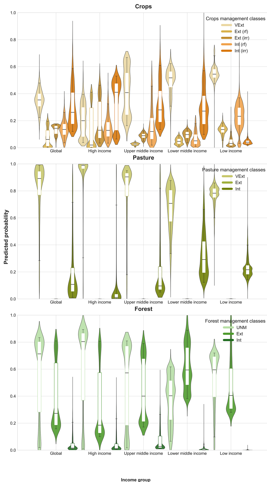
Figure A13. Distribution of predicted probabilities for land management intensity. The distributions for predicted probabilities are shown for cropland, pasture and forest systems across global and world income groups. Violins represent full distribution across grid cells, while embedded boxplots indicate the interquartile range (25th–75th percentiles), median, and dispersion within each group.
