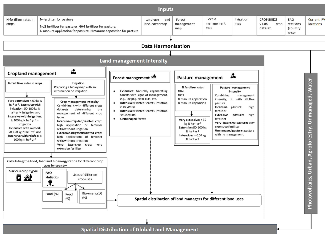
Figure 1. Methodology for land management dataset creation.
