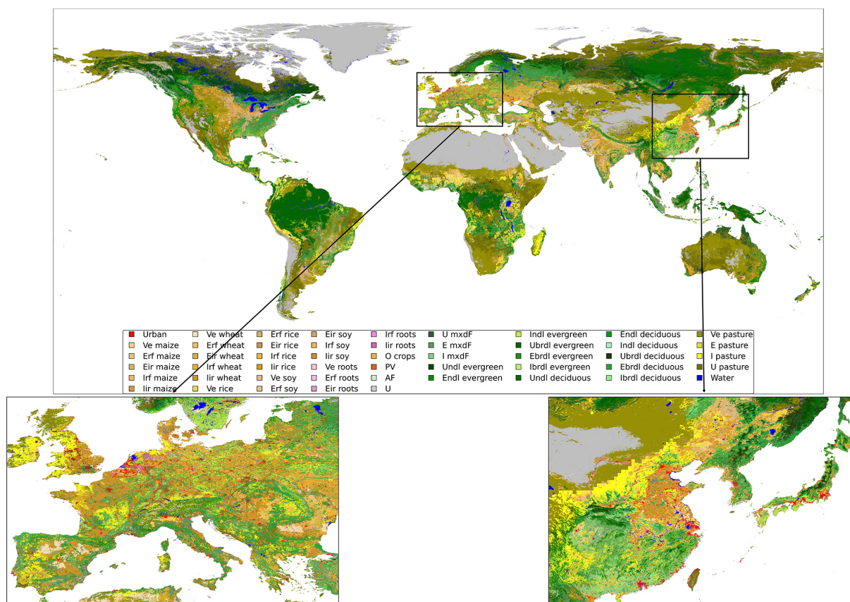
Figure 2. Global land management intensity distribution in 2020 at 0.01° spatial resolution. Here, I – intensive, E – extensive, Ve – very extensive ir – irrigated, rf – rainfed, ndl – needleleaf, bdl – broadleaf, mxdf – mixed forest, PV – photovoltaics, AF – Agroforestry, U – unmanaged, and O – other. Enlarged panels show example regions of Europe and East Asia with dense and heterogeneous land management patterns.
