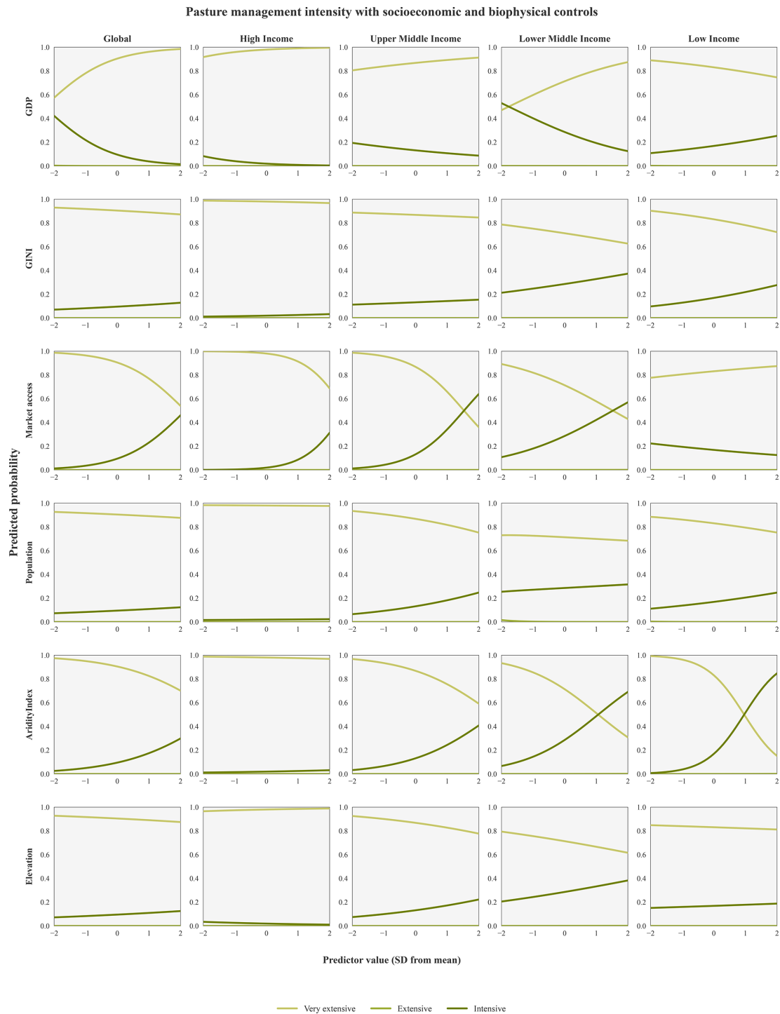
Figure A8. Predicted relationships between pasture management intensity and socioeconomic drivers across global income groups. The x -axes of each plot show the standardised predictor value ( z -score) for various variables (GDP, GINI, market access, and population), and the y -axis indicates the predicted probability of each management intensity (very extensive, extensive, and intensive).
