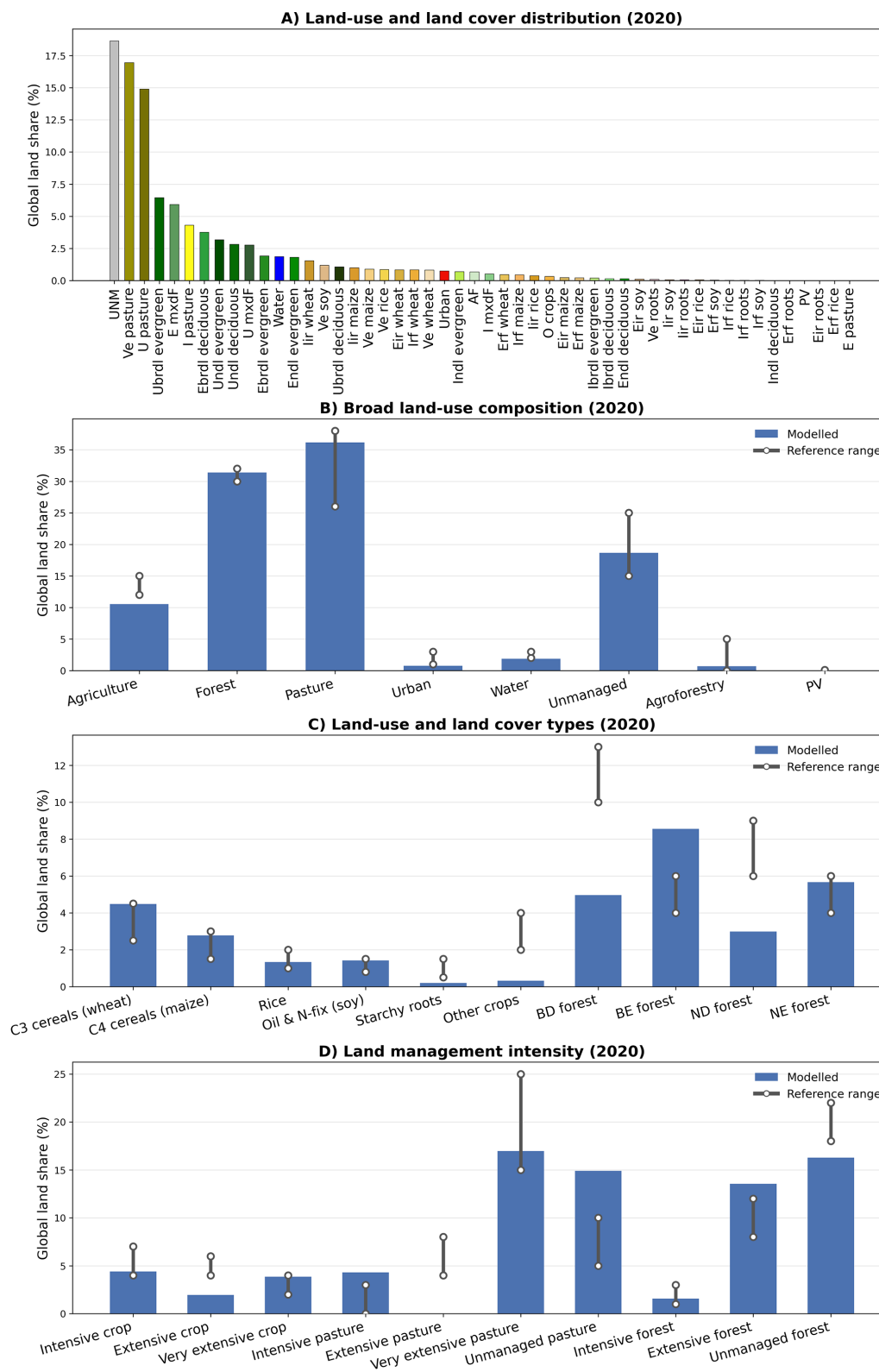
Figure A5. (a) Land-use and land cover distribution and a comparison of modelled and reference global land-use shares. Land-use distribution by (b) groups, (c) types, and (d) management intensities. Land-use groups are the broader land-use and cover sectors, Land-use types are finer land-use types, while Land-use management intensity is further classification of the land-use types in various management intensities. Blue bars denote modelled estimates from this study, and red bars indicate reference data.
