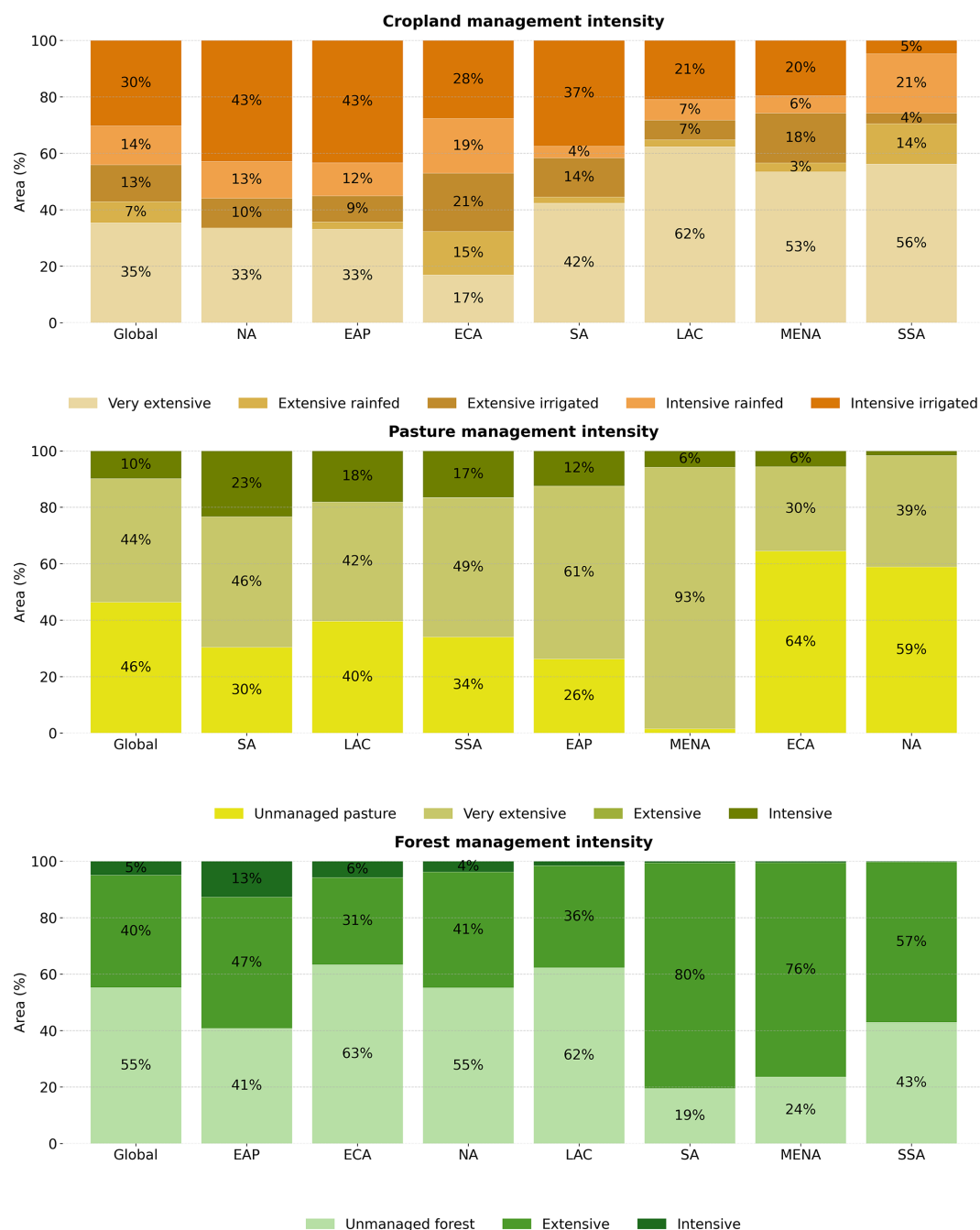
Figure A1. Proportion of cropland, pasture, and forest area under different management intensities by World Bank regions in 2020. Cropland management categories included very extensive, extensive rainfed, extensive irrigated, intensive rainfed, intensive irrigated. Pasture management included unmanaged, very extensive, extensive and intensive pasture. Forest management included unmanaged, extensive and intensive forest. Regions include: EAP – East Asia & Pacific, ECA – Europe & Central Asia, LAC – Latin America & Caribbean, MENA – Middle East & North Africa, NA – North America, SA – South Asia, SSA – Sub-Saharan Africa.
