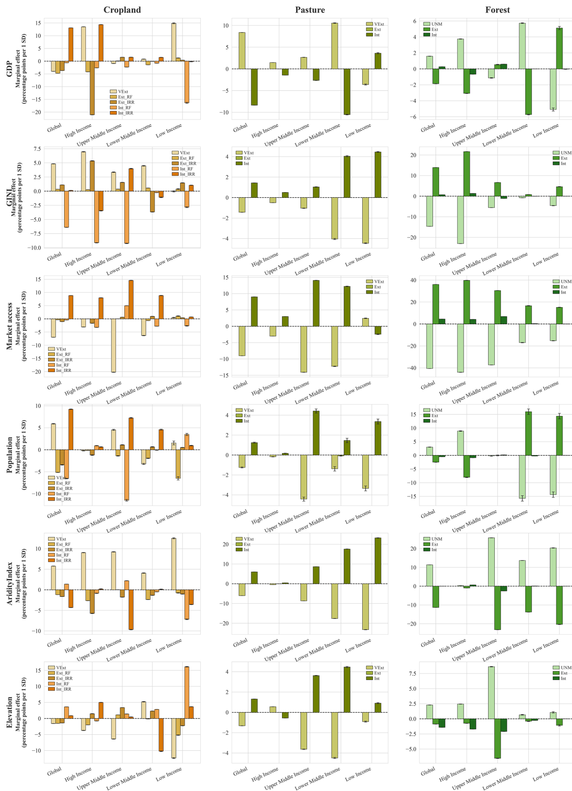
Figure 6. Marginal effects of socioeconomic variables on land management intensities. Individual plot shows an average marginal effect of socioeconomic variables on the predicted probability of land management intensity (very extensive, extensive, and intensive) for cropland, pasture and forest across global and world economic group. Bars represent average marginal effects calculated from multinomial logistic regression method with 95 % confidence interval. Positive (negative) values indicate an increase (decrease) in the probability of a given management intensity class associated with a one standard deviation change in the corresponding socioeconomic variable.
