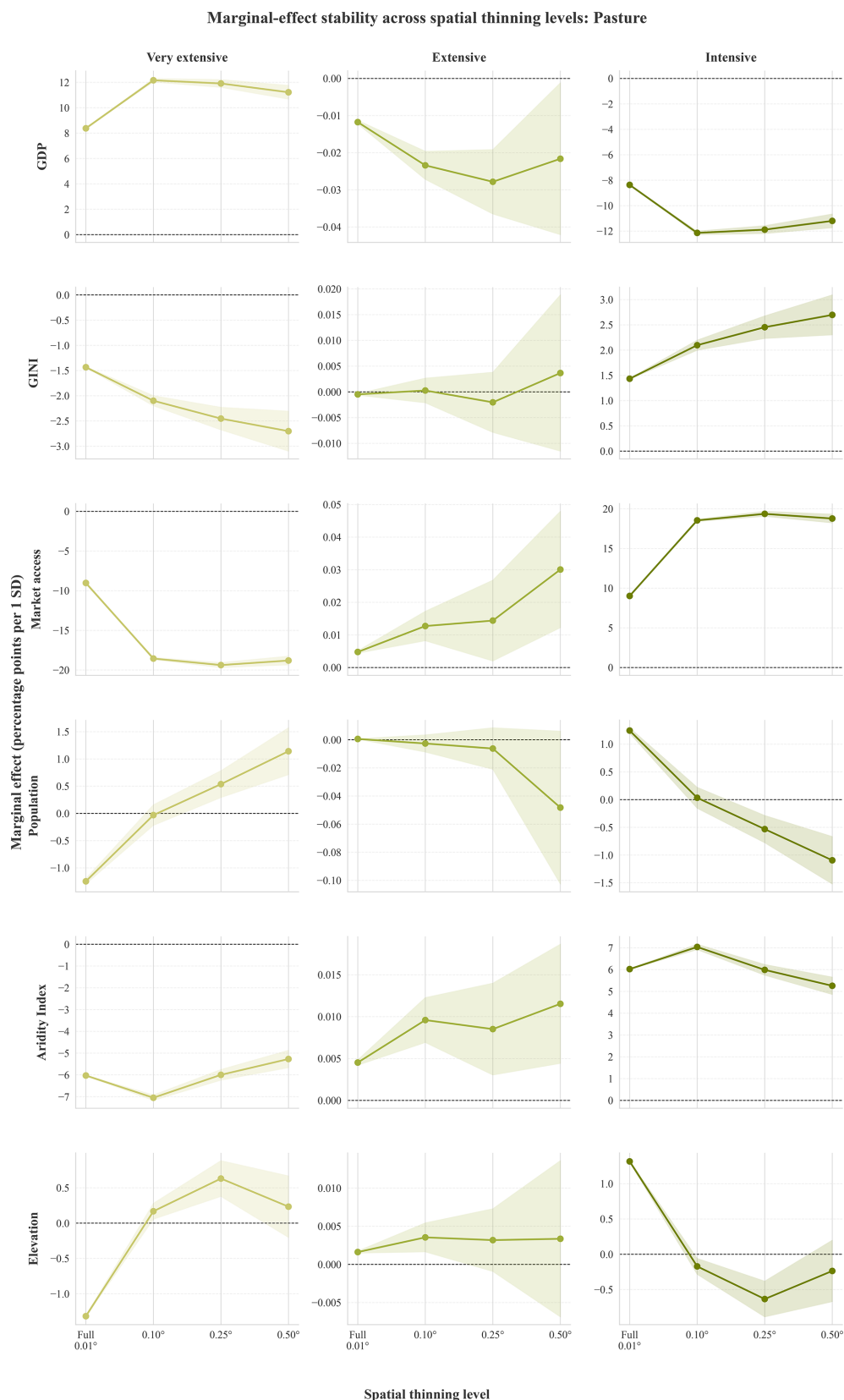
Figure A11. Spatial thinning robustness analysis of marginal effects for pasture management intensity classes. Marginal effects were recalculated using progressively coarser spatial samples (0.10, 0.25, and 0.50°). Lines show marginal effects for each thinning level relative to the full-resolution model (0.01°), while shaded areas indicate confidence intervals.
