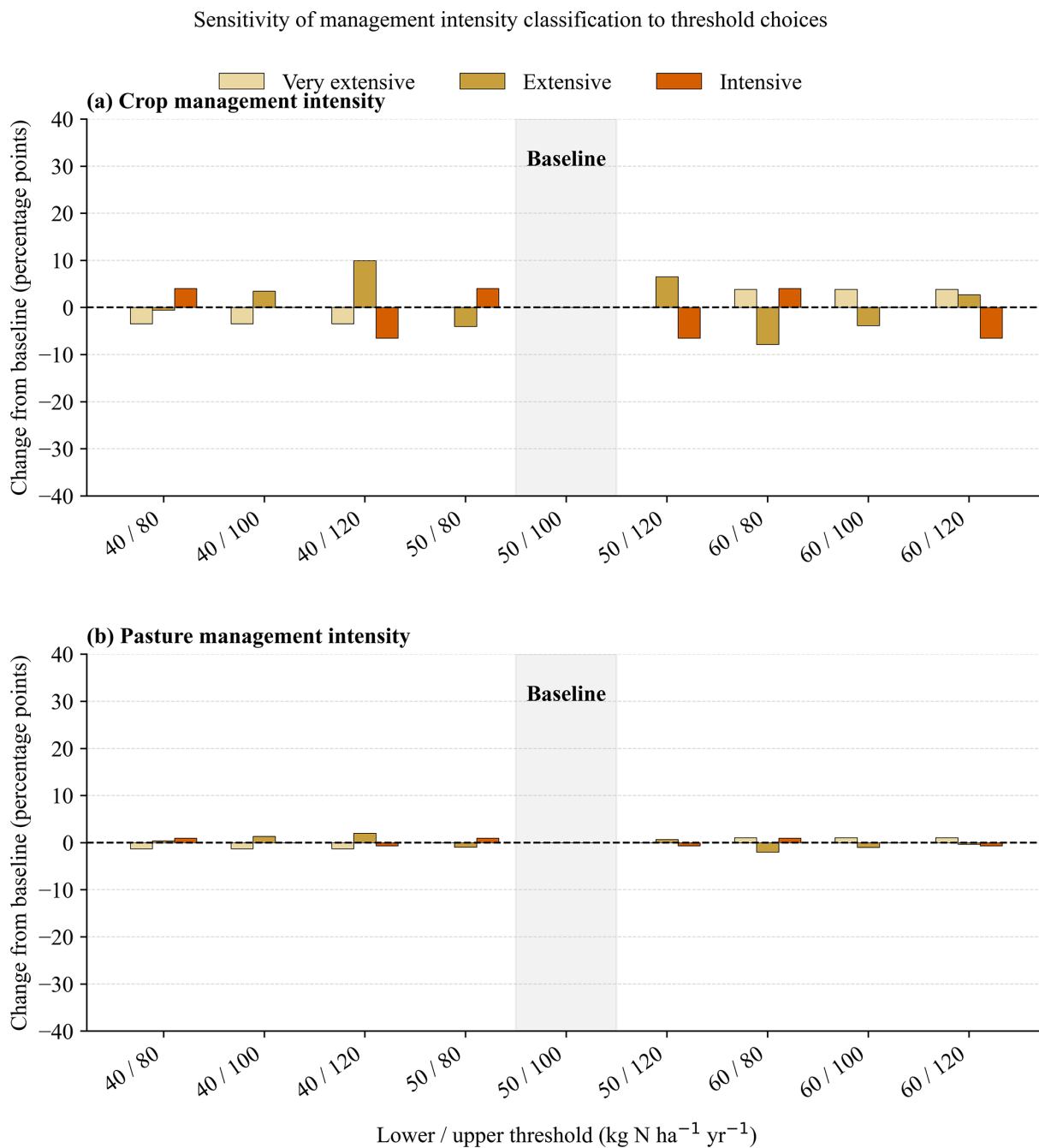
Figure A4. Sensitivity analysis of cropland and pasture management intensity classifications to different thresholds values. The x -axis represents the lower and upper thresholds used for the management intensity classes, while the y -axis indicates changes in the spatial agreement with respect to the baseline in percentage points.
