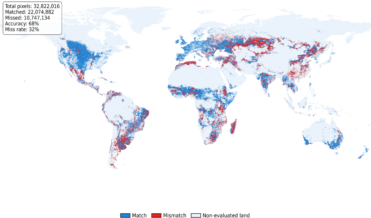
Figure 7. Comparing land management intensities and land-use decision-making types (given by Malek and Verburg, 2020) showing spatial consistency between the decision-making types and management intensities.
