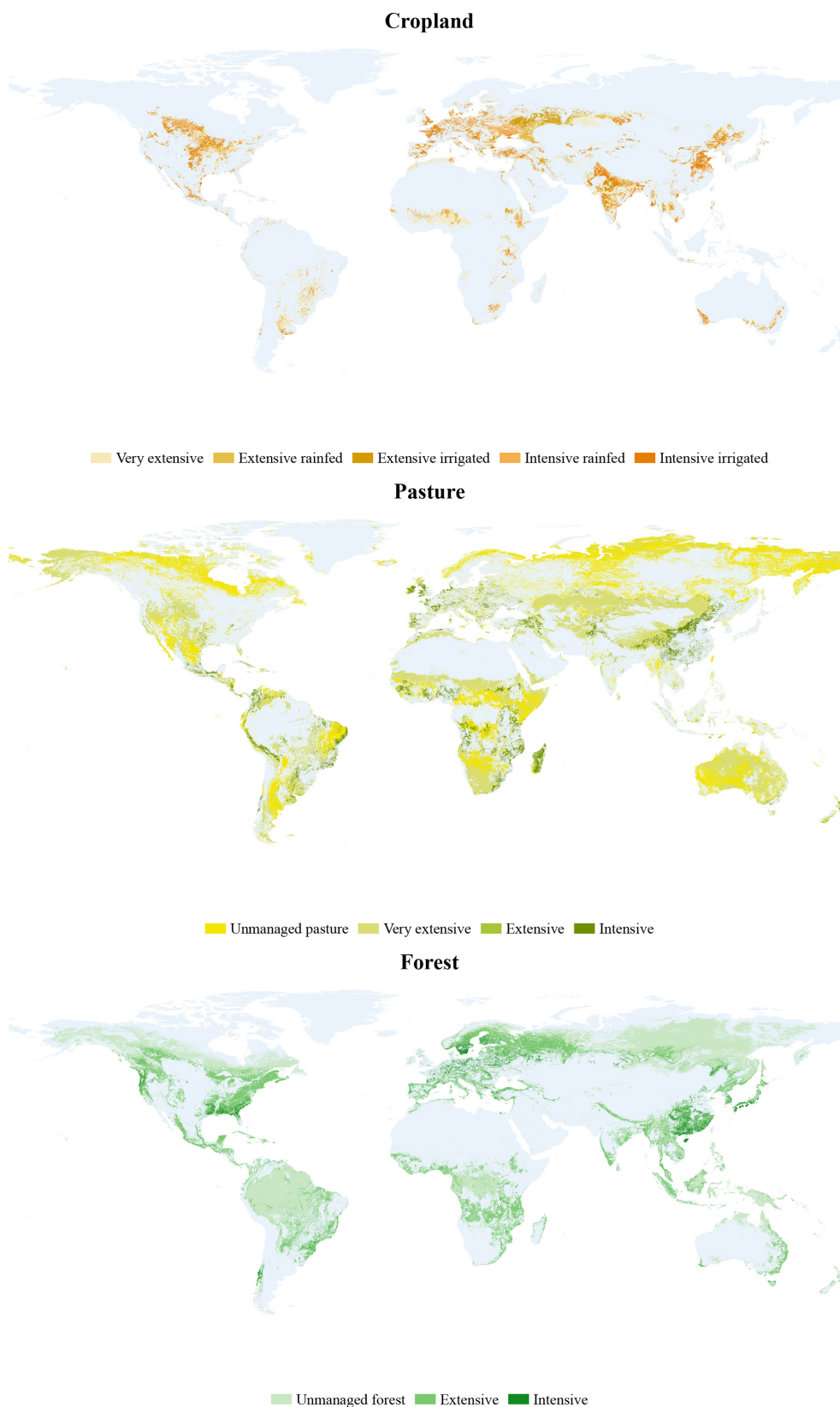
Figure 3. Spatial distribution of land management intensity in cropland, pasture, and forest, categorised into very extensive, extensive, intensive, unmanaged forest, and pasture.
