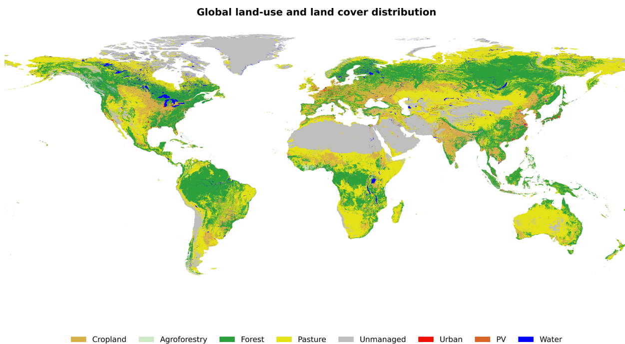
Figure A3. Global Land-use and land cover distribution. The map shows broader land-use and land cover classes.
