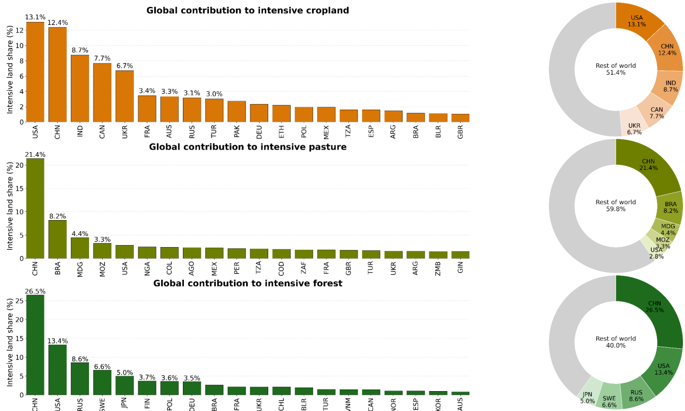
Figure 5. Intensively managed land in cropland, pasture, and forest systems. Bars show the percentage distribution of intensive management class for the top twenty countries, while pie donuts show the contribution of top five countries and the rest of world. Countries are arranged by decreasing share of intensive management.
