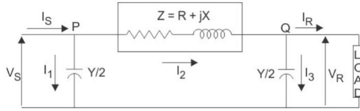
Figure 2.7.: Pi-equivalent circuit: Circuit diagram to approximate the distributed electrical behavior of transmission lines. Figure from Hagenmeyer (2024).
