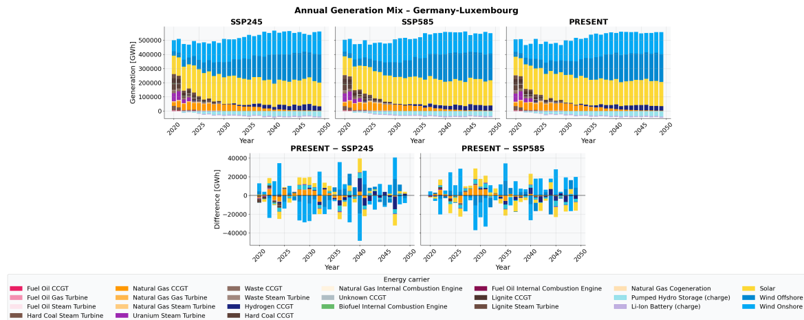
Figure 4.35.: Annual generation mix for Germany-Luxembourg (2020–2049). The transition away from coal and lignite towards wind and solar is clearly visible. Difference plots show high inter-annual variability driven primarily by wind and solar deviations of up to \pm 40\,000 GWh.
