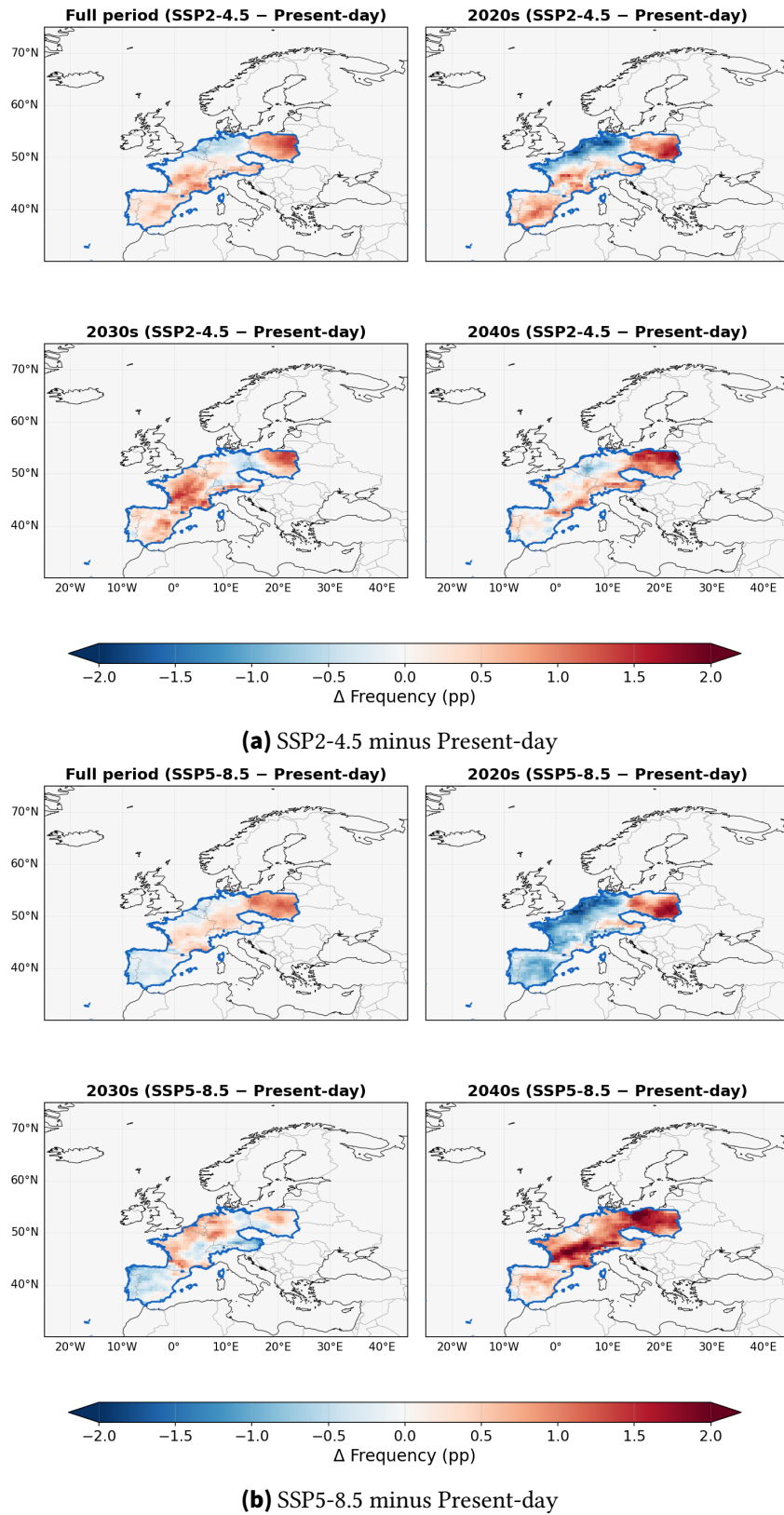
Figure 4.16.: Frequency difference of dark doldrum conditions between future scenarios and Present-day, by decade. Blue outlines determine analysis region boundaries.
