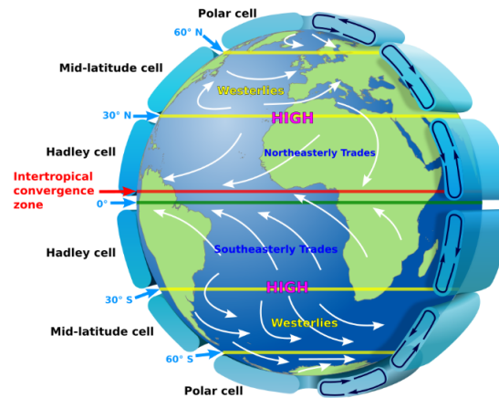
Figure 2.3.: Idealised graphic of the Earth's large-scale winds and atmospheric circulation. Graphic from Atmospheric circulation (2026).
