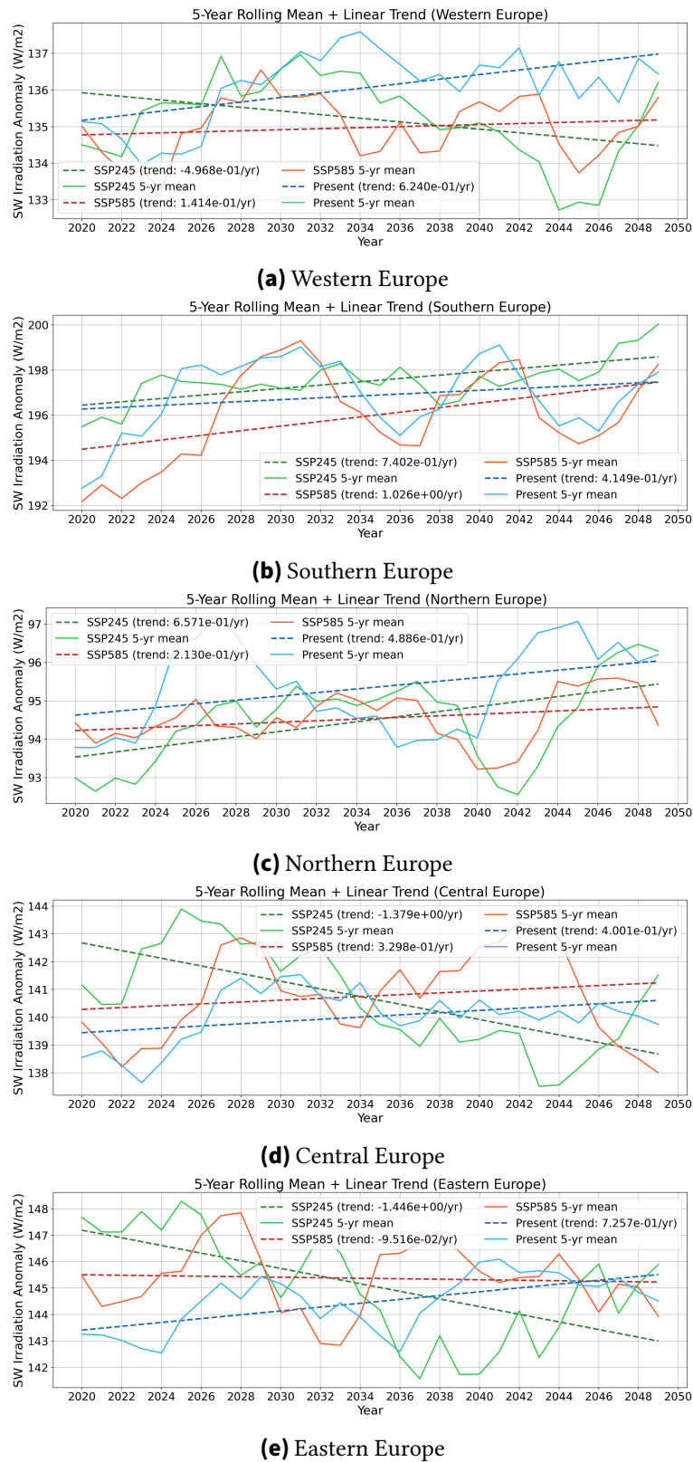
Figure A.4.: Five-year rolling mean of shortwave irradiance ( \text{W m}^{-2} ) with linear trend in different climate zones, 2020–2049.
