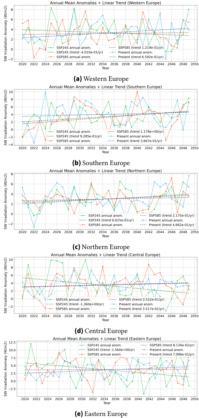
Figure A.3.: Annual mean anomalies and linear trends of shortwave irradiance ( \text{W m}^{-2} ) in different climate zones, 2020–2049.
