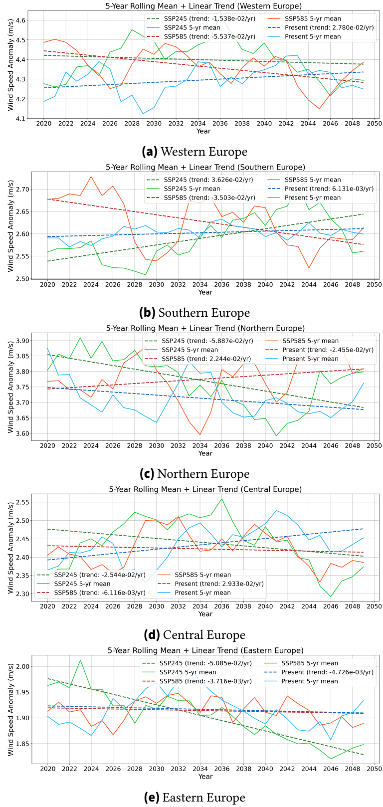
Figure A.2.: Five-year rolling mean of 10 m wind speed ( \text{m s}^{-1} ) with linear trend in different climate zones, 2020–2049.
