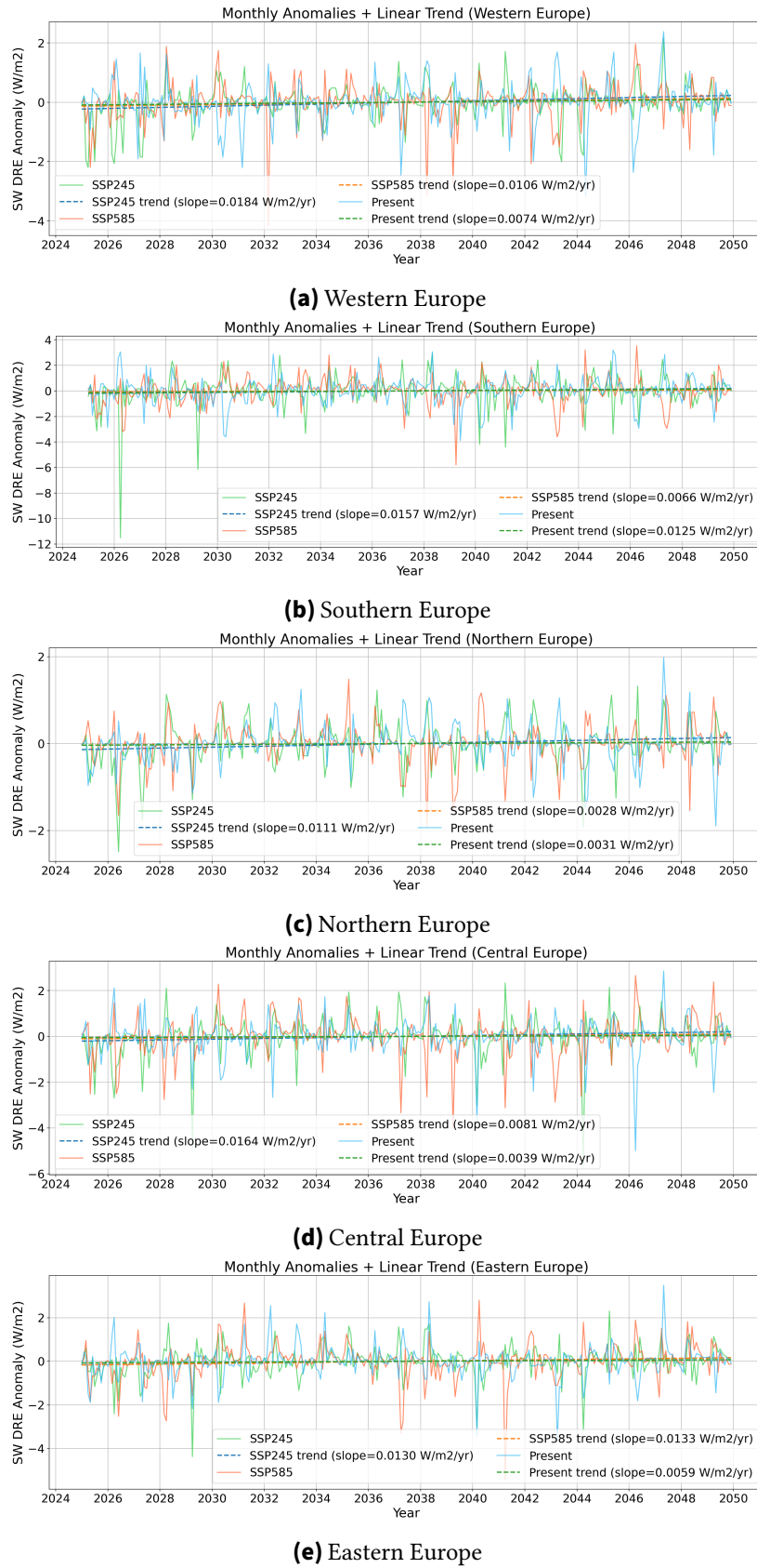
Figure 4.11.: Monthly SW DRE anomalies ( \text{W m}^{-2} ) and OLS linear trends, sub-period 2025–2050 (model spin-up excluded). Dashed lines indicate OLS trends per scenario.
