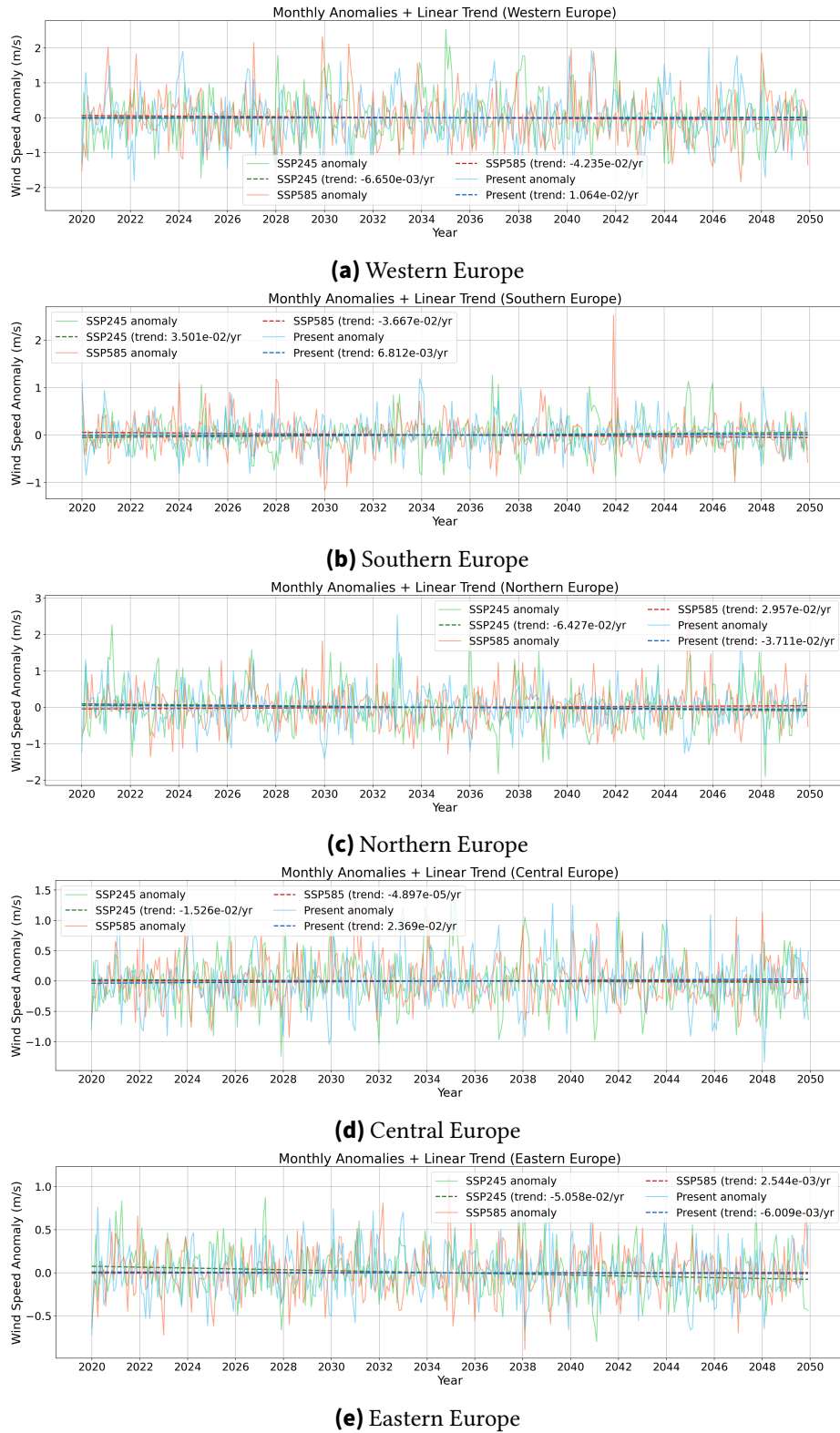
Figure 4.4.: Monthly anomalies and linear trends of 10 m wind speed ( \text{m s}^{-1} ) in different climate zones, 2020–2050.
