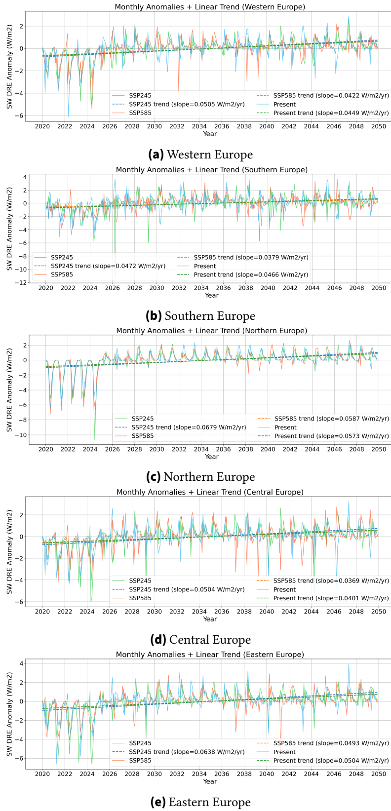
Figure 4.10.: Monthly SW DRE anomalies (W m -2 ) and OLS linear trends, full period 2020–2050. All three scenarios are shown; dashed lines indicate OLS trends.
