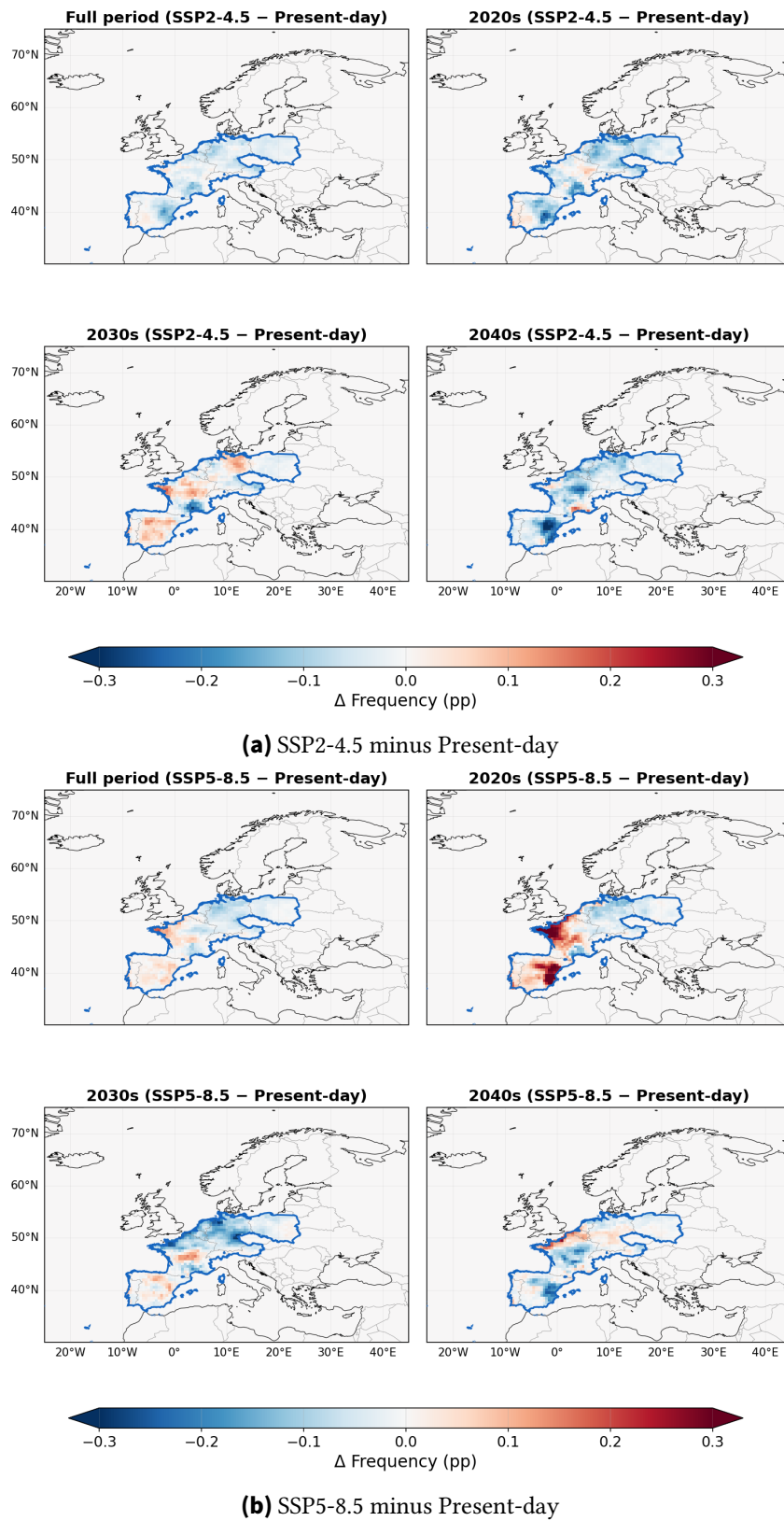
Figure 4.21.: Frequency difference of light breeze conditions between future scenarios and Present-day, by decade. Blue outlines determine analysis region boundaries.
