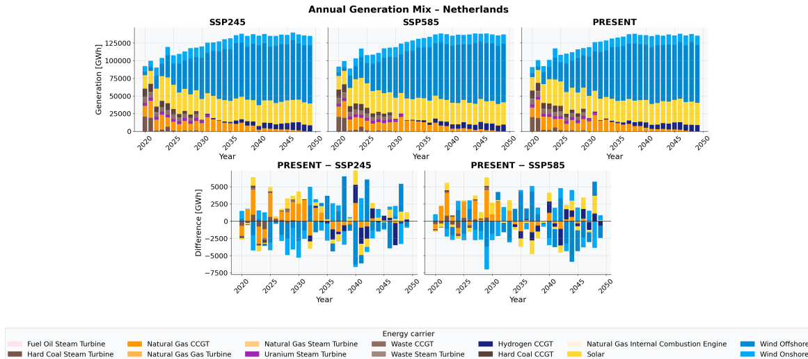
Figure 4.37.: Annual generation mix for the Netherlands (2020–2049). Natural gas is progressively replaced by offshore wind and solar PV. Hydrogen CCGT emerges as a dispatchable backup technology from the mid-2030s onwards.
