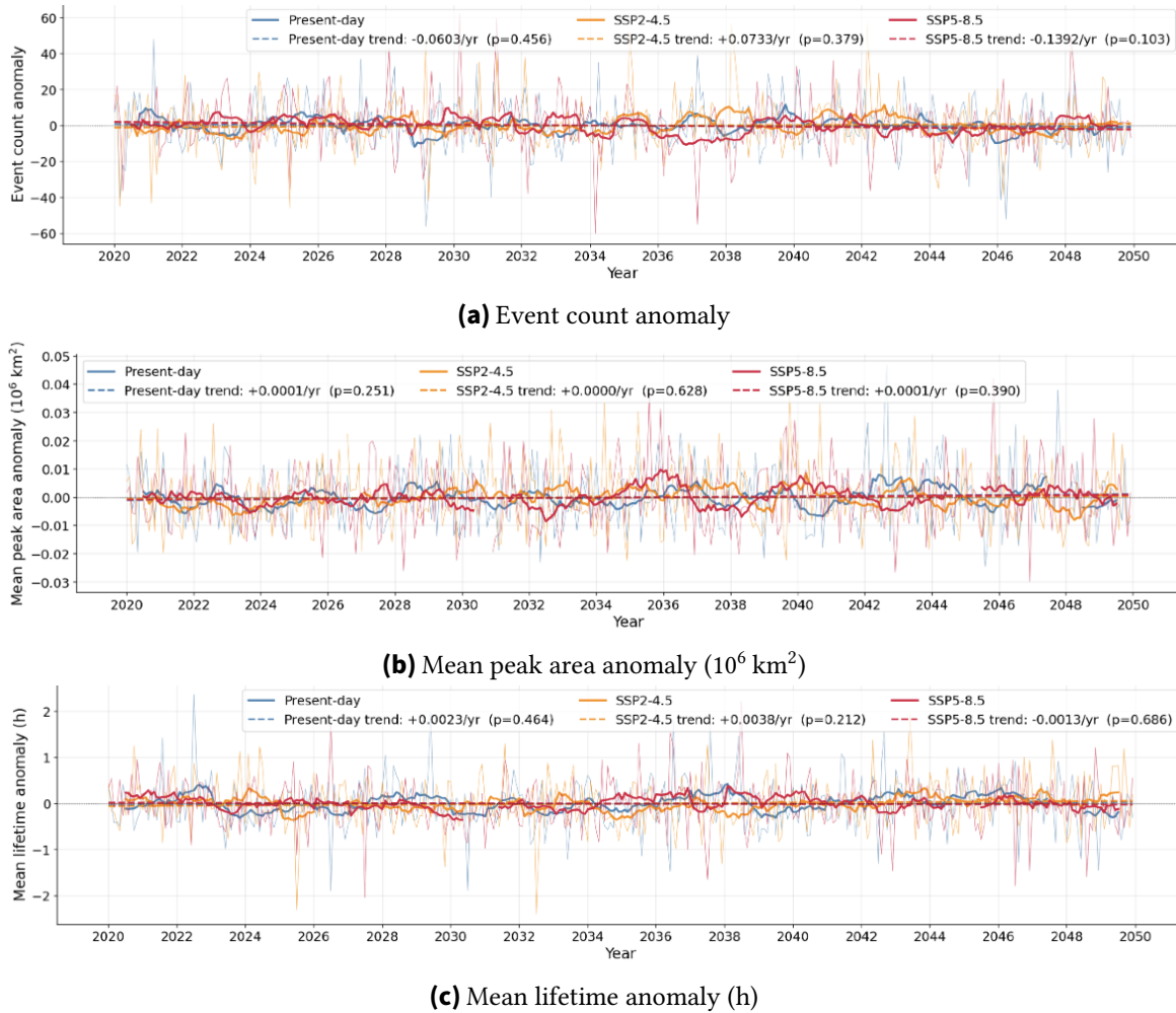
Figure 4.18.: Monthly de-seasoned anomalies and linear trends for light breeze events, 2020–2050.
