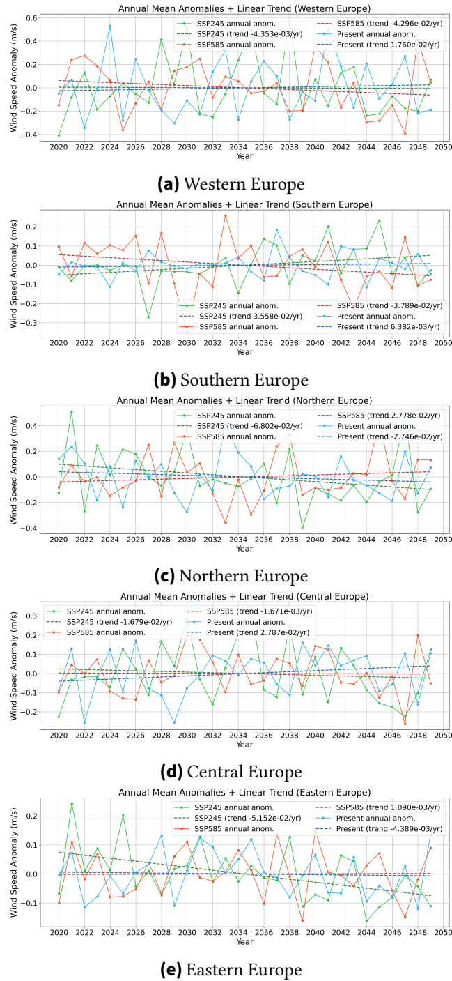
Figure A.1.: Annual mean anomalies and linear trends of 10 m wind speed ( \text{m s}^{-1} ) in different climate zones, 2020–2049.
