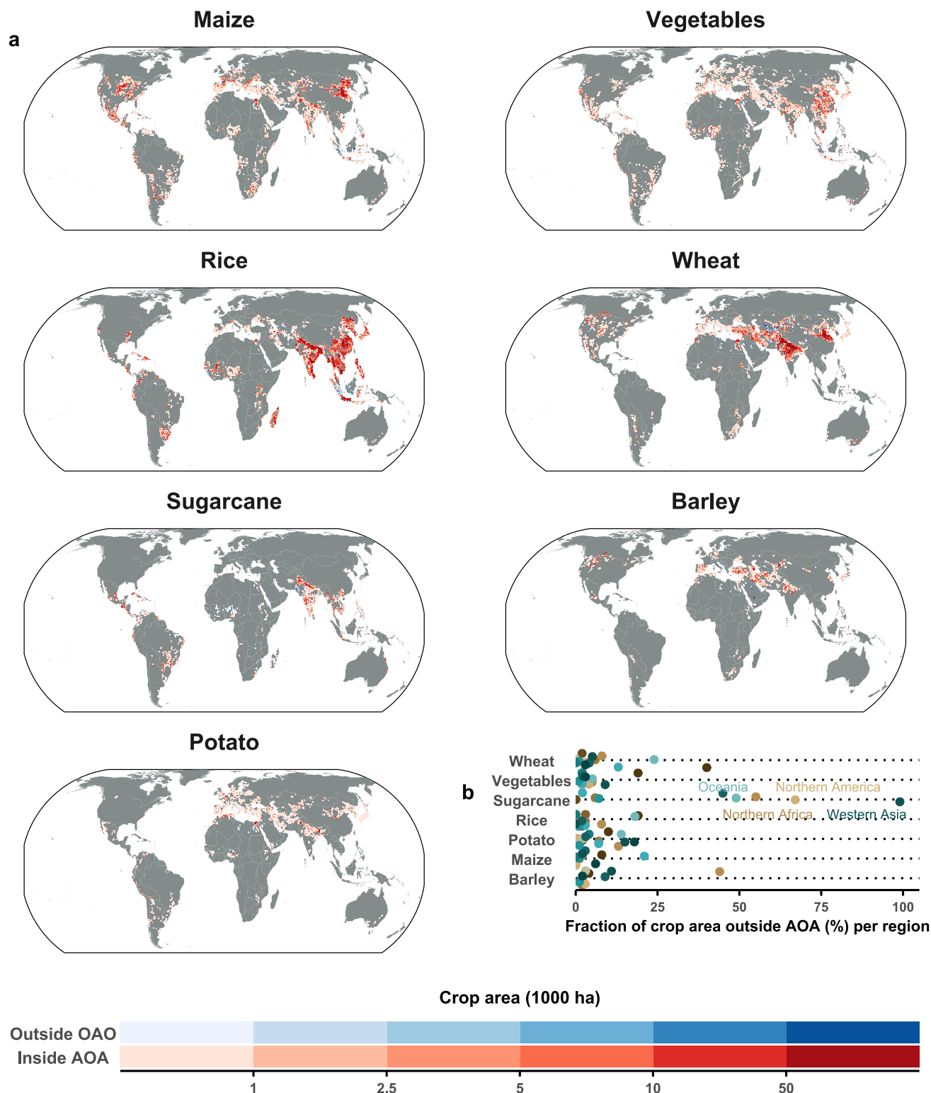
Extended Data Fig. 3 | Area of applicability of the gridded Nlrrig predictions.
