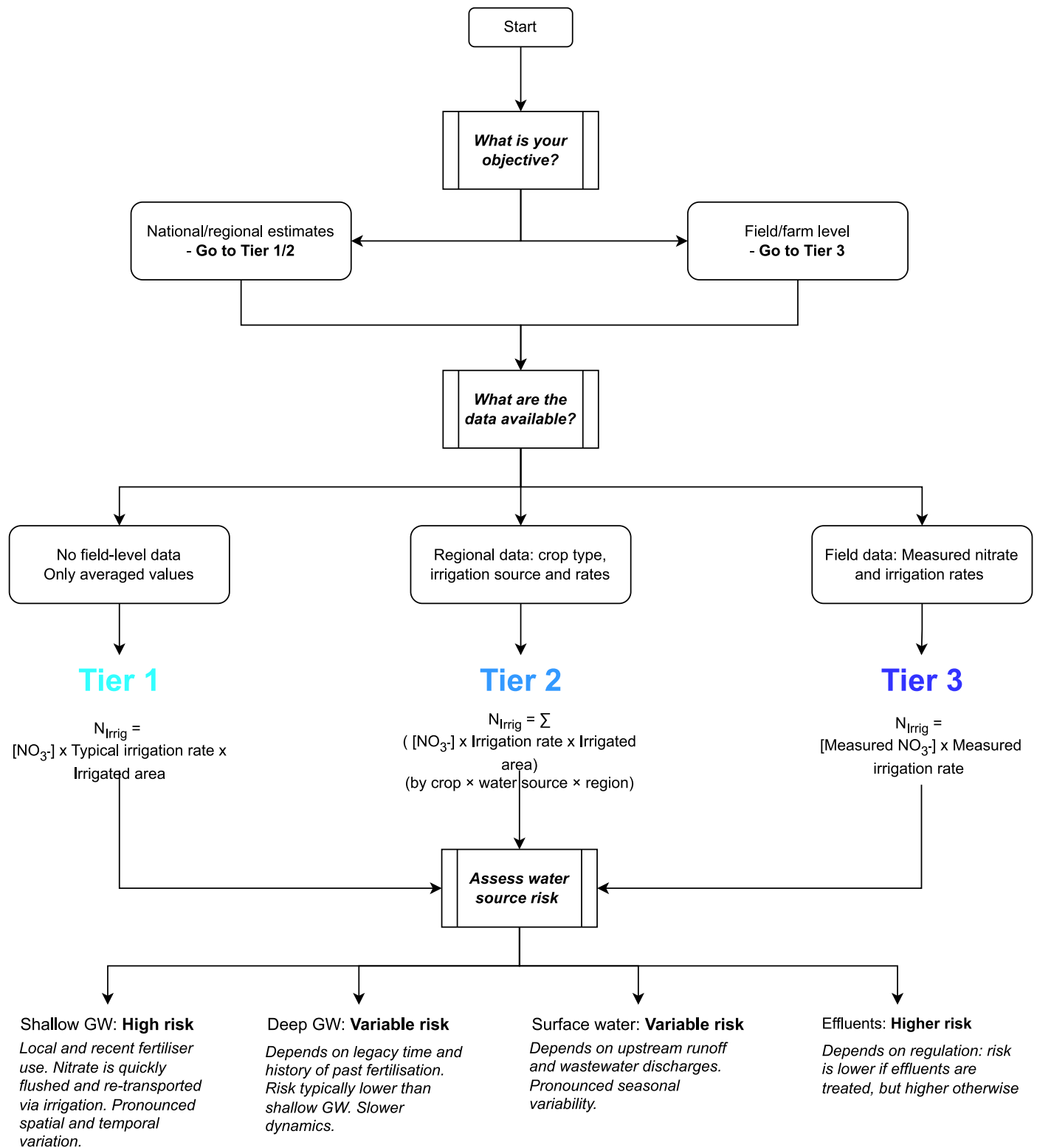
Extended Data Fig. 7 | Decision tree to estimate the nitrogen input via irrigation water using a tiered approach. Additional information for the estimations of Tier 1 and 2 (for example, data sources) are provided in Data Availability.
