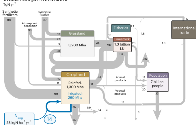
Fig. 4 | Irrigation water represents a considerable nitrogen flow in the global agrofood system. Global representation of the agrofood system (GRAFS) in 2013, expressed in N flows between main system compartments. LU, livestock unit.
