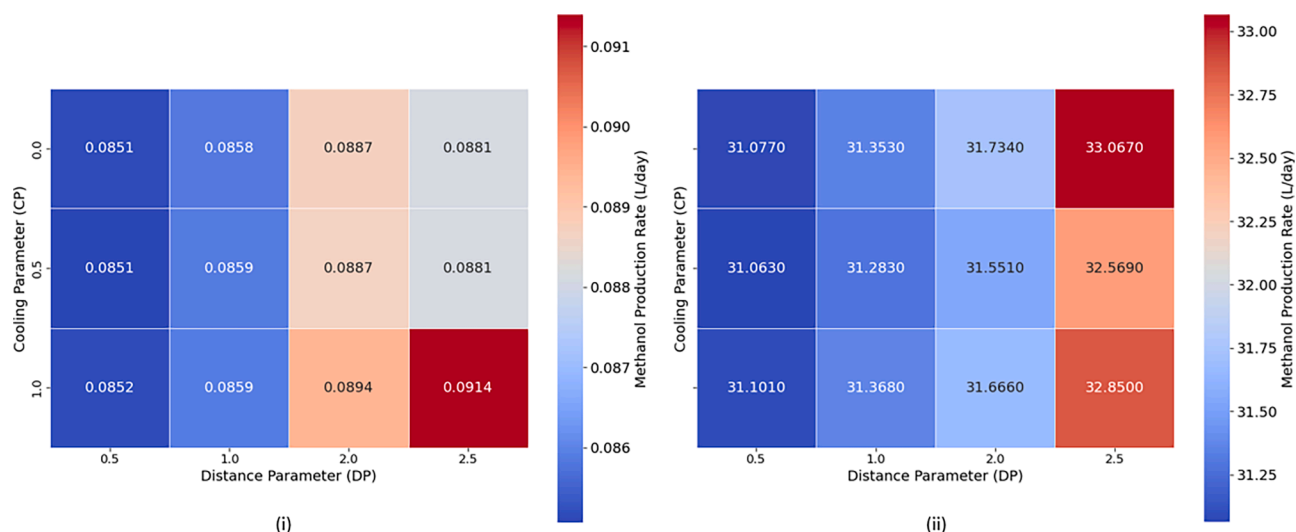
Fig. 9. Effect of cooling and distance parameters on methanol production rate at (i) lab and (ii) container scale, showing how the influence of both parameters changes with reactor scale.
