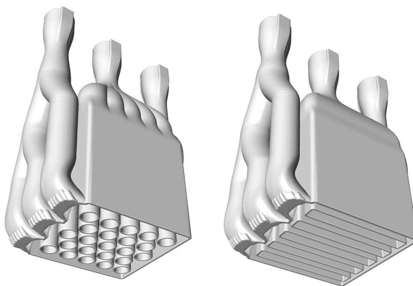
Fig. 10. CAD renderings of two reactor designs with different internal channel geometries generated by the design automation tool: (i) circular and (ii) parallel rectangular channel configurations, demonstrating that different channel concepts can be produced without manual CAD remodeling.
