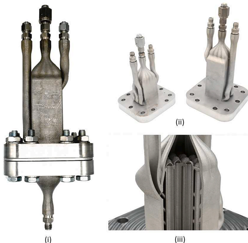
Fig. 6. Additive manufactured reactor components for experimental tests: (i) Assembled configuration, (ii) manufactured reactor prototypes, and (iii) internal design of the reactor with permeable catalyst holder.
