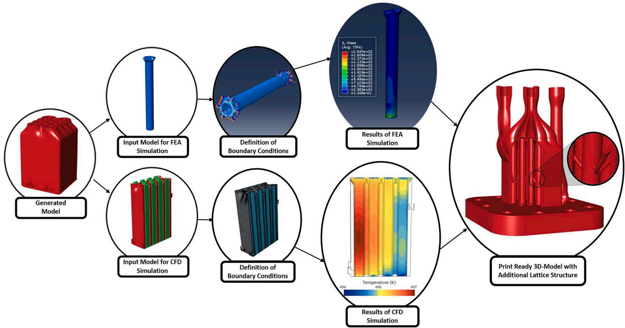
Fig. 4. Illustration of a single CFD or FEA simulation workflow and the generation of a print-ready 3D-Model with additional lattice structure (adapted from [44]).
