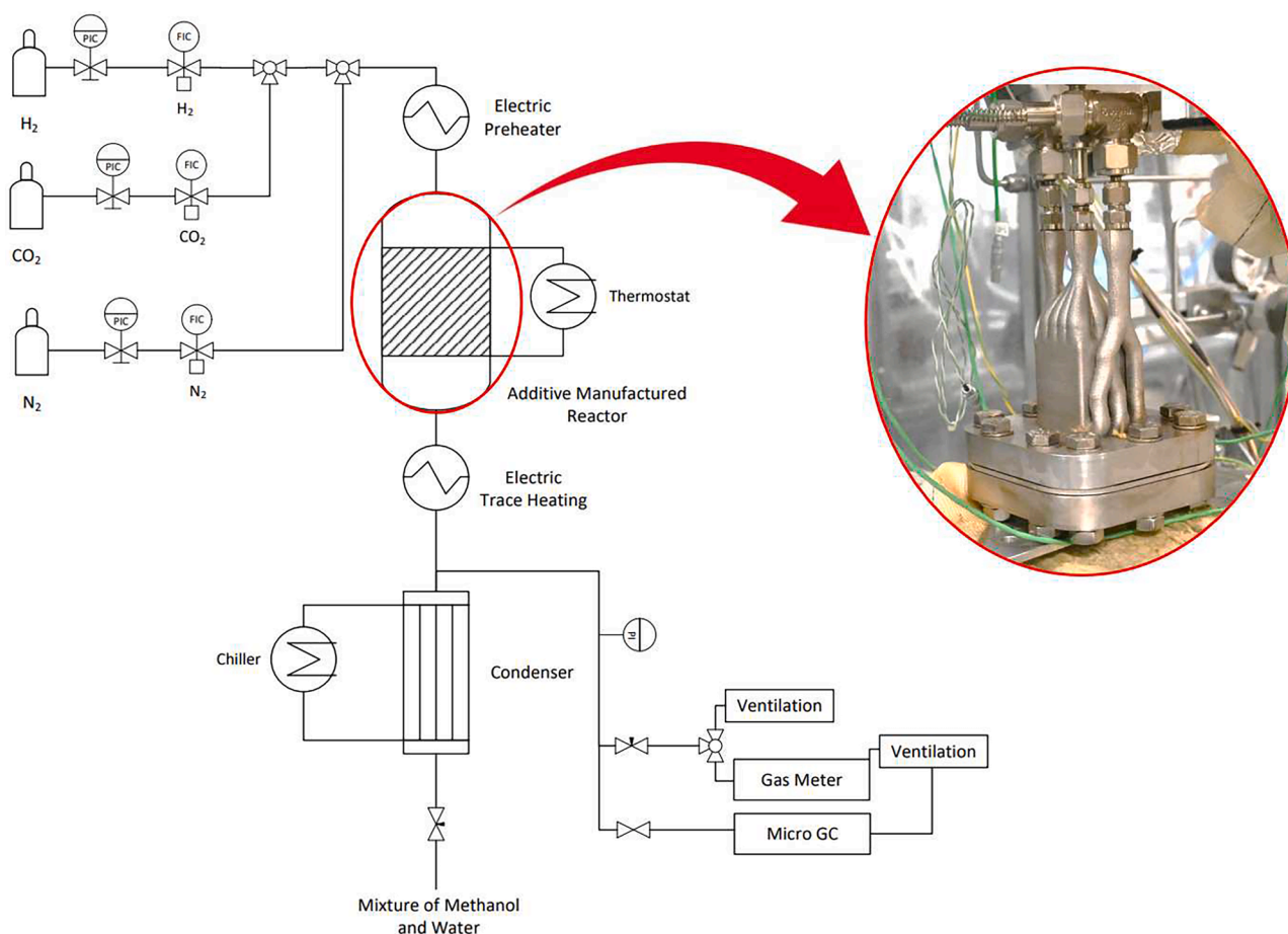
Fig. 7. Schematic of the experimental setup for methanol synthesis, highlighting the integration of the additively manufactured reactor. The detailed view shows the assembled reactor installed within the test bench.
