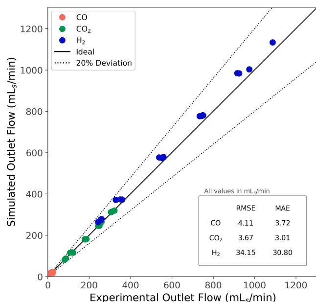
Fig. 8. Parity plot of simulated and experimental outlet volume flows of CO, CO 2 , and H 2 for all tested reactor configurations and inlet flow rates; full test data are available in the supplementary information.
