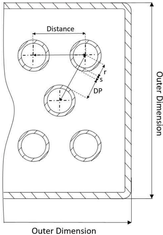
Fig. 5. Geometrical definition of the channel arrangement within the reactor cross-section, relating the distance parameter (DP), wall thickness (s), and channel radius (r) to the resulting number of channels (N) at constant catalyst volume.
