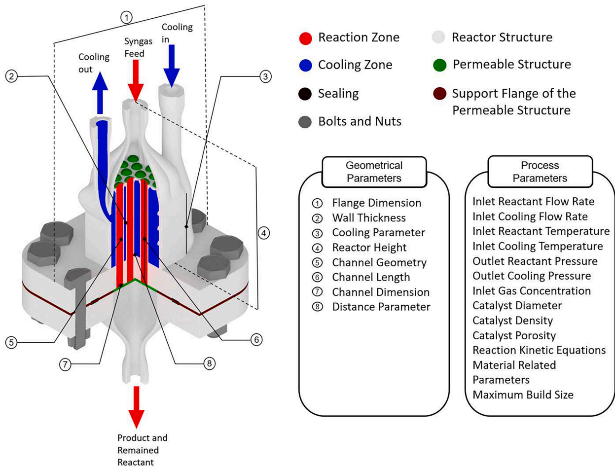
Fig. 2. Schematic representation of the 3D-printed methanol synthesis reactor, illustrating key functional zones, structural components, and the associated geometrical and process parameters used in the design automation tool.
