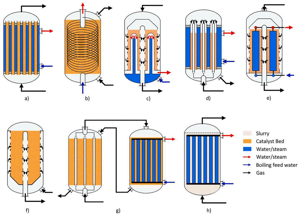
Fig. 1. Simplified schematic representations of established industrial methanol synthesis reactors, illustrating the range of heat-removal strategies that motivate the AM-based reactor concept adopted in this work: (a) the Lurgi tubular reactor, (b) the Linde Variobar system, (c) the Toyo MRF reactor, (d) the Mitsubishi Superconverter, (e) the Methanol Casale IMC reactor, (f) the Haldor Topsøe adiabatic reactor, (g) the Lurgi MegaMethanol process, and (h) the Air Products LPMEOH reactor [5].
