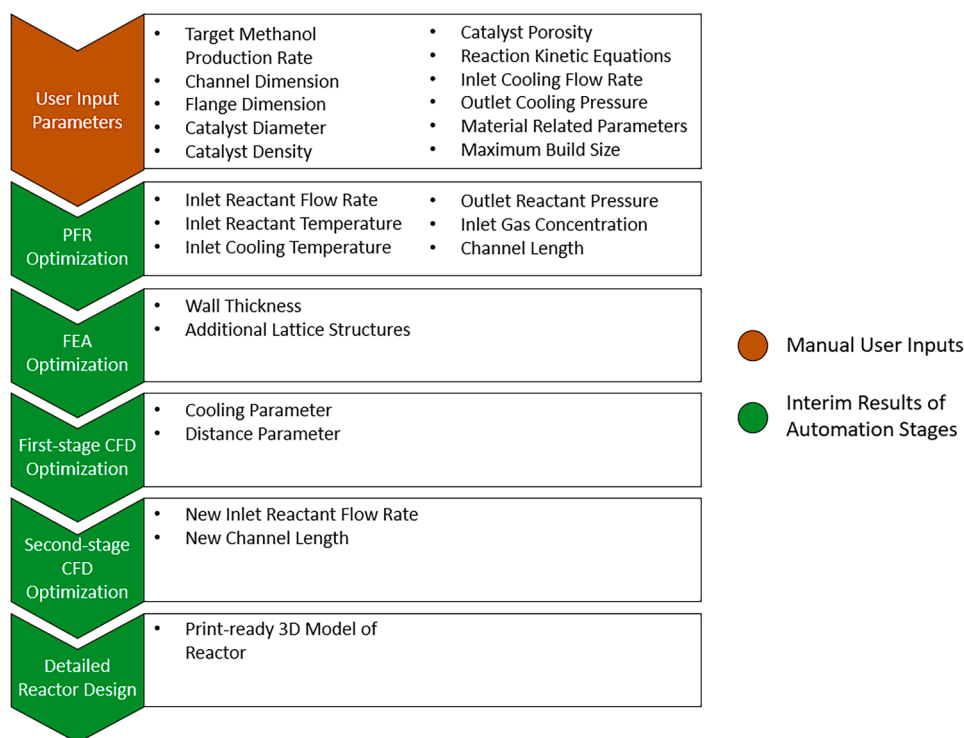
Fig. 3. Workflow of the automated reactor design process in the proposed tool, illustrating the sequential optimization steps, from user input parameters through PFR, FEA, and CFD optimizations, to the generation of a print-ready 3D reactor model.
