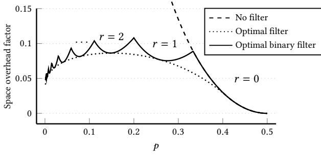
Figure 4: Idealised space overhead of filter-based WRM for keys with weight p \in [0, \frac{1}{2}] . Optimal filter shows the overhead (\text{space}(p, r_{\mathbb{R}_{\geq 0}}^*(p)) - H(p))/H(p) when using a weighted filter that supports real-valued weights. The maximum is \approx 0.086 at p \approx 0.15 . Optimal binary filter shows the overhead (\text{space}(p, r_{\mathbb{N}_0}^*(p)) - H(p))/H(p) when using a weighted filter that supports integer weights only. The maximum is \approx 0.108 at p = 0.2 .
