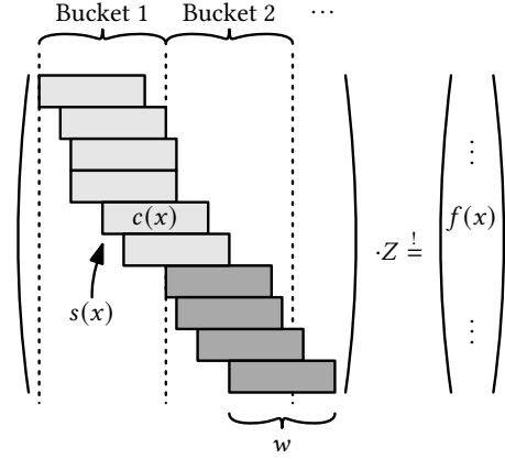
Figure 2: Structure of the BuRR equation system [26].
