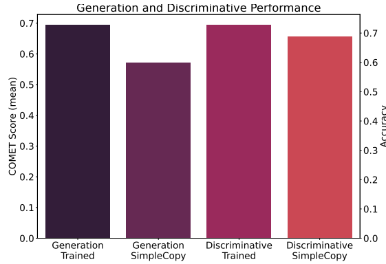
Figure 7. Average generation and discriminative performance for trained and transformed LoRA adapters using SimpleCopy . Discriminative tasks transfer more robustly than generative tasks. SimpleCopy LoRA adapters retain most of the performance of natively trained adapters on discriminative tasks, whereas generative performance degrades substantially, supporting the claim that discriminative capabilities require less task-specific adaptation.
