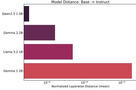
Figure 3. Distance between the pre-trained and instruction-tuned models.
