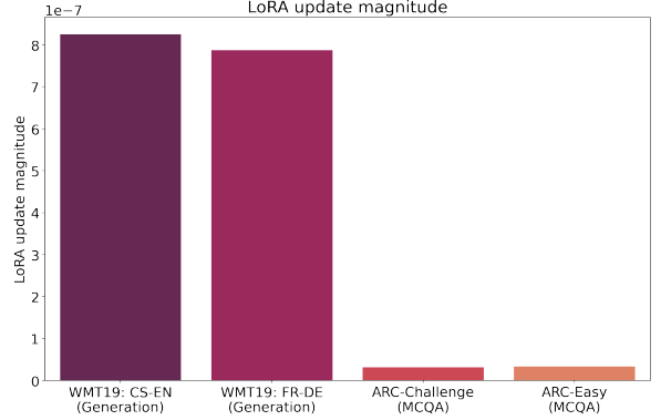
Figure 5. Training on ARC-C and ARC-E yields only marginal adjustments to the base model, whereas translation tasks necessitate substantially larger LoRA adaptation.
