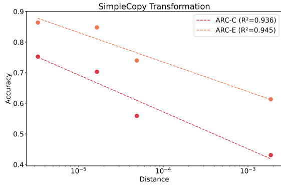
Figure 4. Inverse relationship between the efficacy of SimpleCopy and the source-target model distance on ARC-E and ARC-C. The dashed lines indicate a least-squares linear fit in log-distance space.
