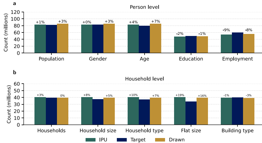
Fig. B.8. Comparison of aggregated target and synthetic population counts for Germany. Counts obtained from the Iterative Proportional Updating (IPU) weights and after household sampling (Drawn) are compared with the target counts from the marginal distributions (Target). The comparison is shown for person-level totals, including the total population and the aggregated counts for age, gender, education, and employment status (a), and for household-level totals, including the total number of households and the aggregated counts for household size, household type, living area, and building type (b). Relative deviations above the bars indicate the percentage difference between the IPU or Drawn counts and the corresponding target counts.
