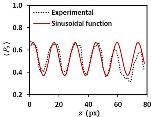
Fig. 3. Evolution of the experimental \langle P_2 \rangle values along the z -axis for the centrifuged sample extracted from Fig. 2b. The experimental profile (dotted line) is fitted by a sinusoidal function (red line). (For interpretation of the references to colour in this figure legend, the reader is referred to the web version of this article.)
