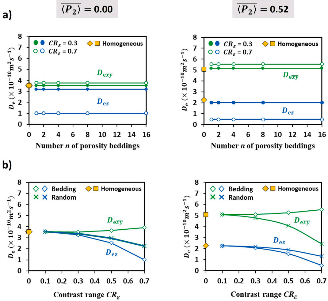
Fig. 5. Influence of the porosity microstructure on the calculated water effective diffusion coefficient ( D_e ) for \langle P_2 \rangle = 0.00 (left) and \langle P_2 \rangle = 0.52 (right). (a) Evolution of the D_e values with the number n of beddings for two contrast ranges, i.e., CR_\varepsilon = 0.3 (solid circles) and CR_\varepsilon = 0.7 (open circles). (b) Evolution of D_e values with the contrast range CR_\varepsilon for bedding ( n = 5.5 ; open diamonds) and random microstructures (crosses; see section 3.3.2 for details). In (a) and (b), the homogeneous microstructure is shown as orange square and diamond for D_{e\bar{x}\bar{y}} and D_{ez} , respectively.
