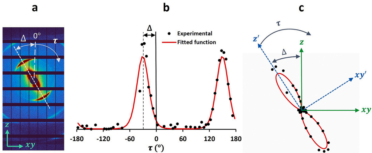
Fig. 1. Extraction of clay particle orientation from 2D-μXRD technique. (a) Individual 2D-μXRD pattern showing the intensity distribution I(\tau) on the (001) diffraction ring (dark red areas) for the centrifuged IDP sample. The azimuthal angle \tau and the detector reference are also shown. (b) Comparison between the experimental I(\tau) data (solid circle) and the fitted function (solid red line) to determine the deviation angle \Delta of the orientation tensor and the degree of particles orientation ( \langle P_2 \rangle ). (c) Orientation tensor of particles derived from the 2D-μXRD pattern in polar coordinates and its relation with xyz detector reference. (For interpretation of the references to colour in this figure legend, the reader is referred to the web version of this article.)
