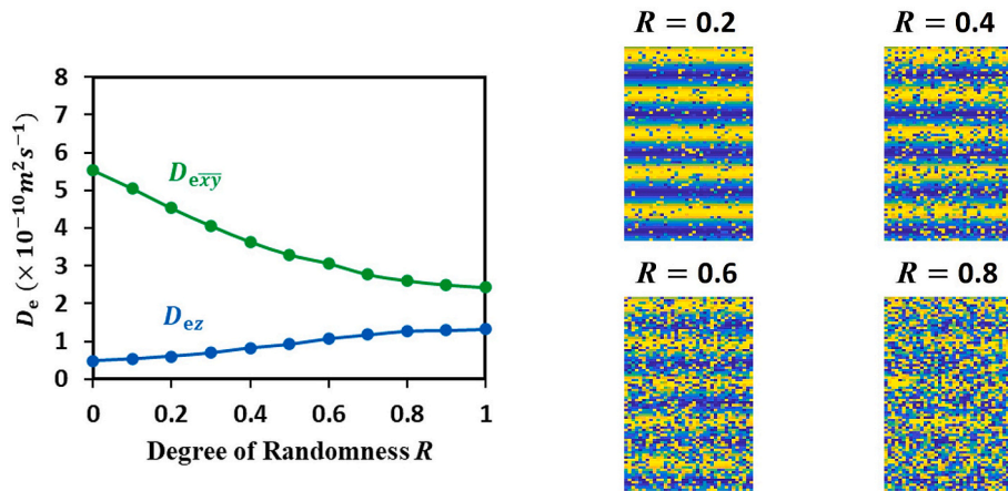
Fig. 6. Evolution of the water effective diffusion coefficient D_e in both the \bar{x}\bar{y} - and z -directions as a function of randomness degree R , starting from the bedding pattern with \bar{\varepsilon} = 0.38 , \langle P_2 \rangle = 0.52 , and CR_\varepsilon = 0.7 (Fig. 5b). Four selected maps are shown in the right part of the figure with R = 0.2, 0.4, 0.6, and 0.8 .
