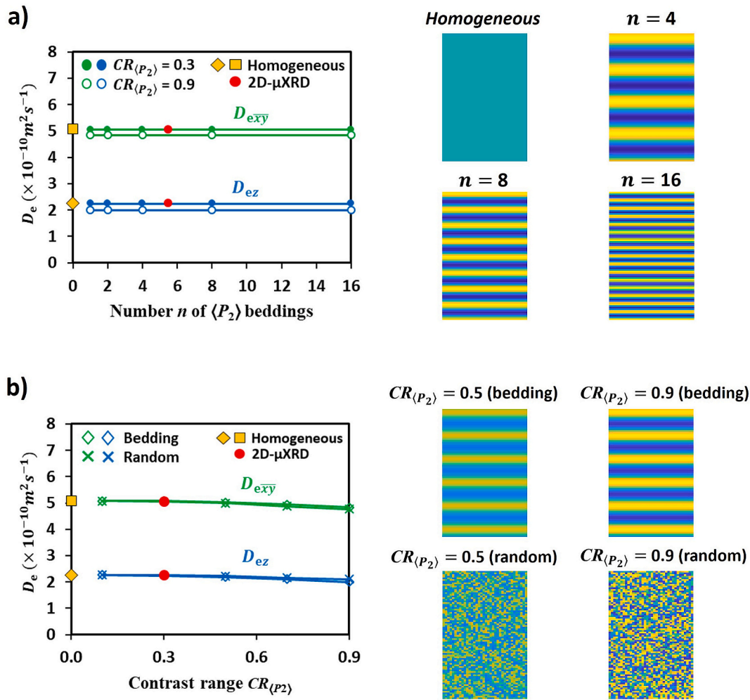
Fig. 4. Influence of the microstructure in preferred orientation of clay particles (parameter \langle P_2 \rangle ) on the calculated water effective diffusion coefficient ( D_e ) for a mean porosity \bar{\epsilon} = 0.38 and a mean \overline{\langle P_2 \rangle} value of 0.52. (a) Evolution of D_e values with the number n_{\langle P_2 \rangle} of beddings for two contrast ranges, i.e., CR_{\langle P_2 \rangle} = 0.3 (solid circles) and CR_{\langle P_2 \rangle} = 0.9 (open circles). (b) Evolution of D_e values with the contrast range CR_{\langle P_2 \rangle} for bedding ( n_{\langle P_2 \rangle} = 5.5 ; open diamonds) and random microstructures (crosses; see section 3.3.1 for details). In (a) and (b), the homogeneous microstructure is shown as orange square and diamond for D_{e\bar{x}\bar{y}} and D_{ez} , respectively. The simulated D_e values using the maps obtained from 2D- \mu XRD for the centrifuged IDP sample (Table 1) are also indicated in red solid circles. Four selected maps are shown on the right part of the figure in (a) and (b). In (a), the homogeneous organization is compared to the bedding microstructure with CR_{\langle P_2 \rangle} = 0.3 and n_{\langle P_2 \rangle} = 4, 8 , and 16. In (b), the bedding microstructure at two CR_{\langle P_2 \rangle} values (top) are compared to its corresponding random organization (bottom). (For interpretation of the references to colour in this figure legend, the reader is referred to the web version of this article.)
