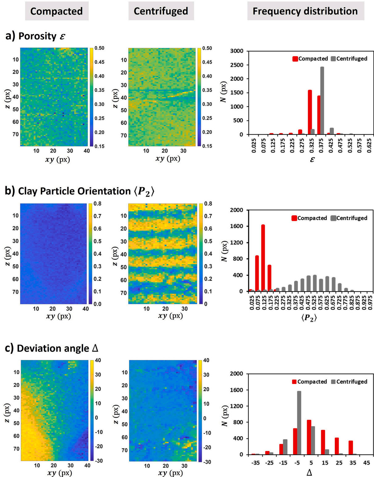
Fig. 2. Colour-code mapping (left and center) and frequency distribution (right) of different parameters, including (a) porosity ( \varepsilon ), (b) preferred orientation of clay particle ( P_2 ) parameter, and (c) deviation angle of the particle orientation tensor ( \Delta ) for both compacted and centrifuged IDP samples based on synchrotron depth-averaged 2D- \mu XRD analyses. The map pixel size is 76.85 \mu\text{m} .
