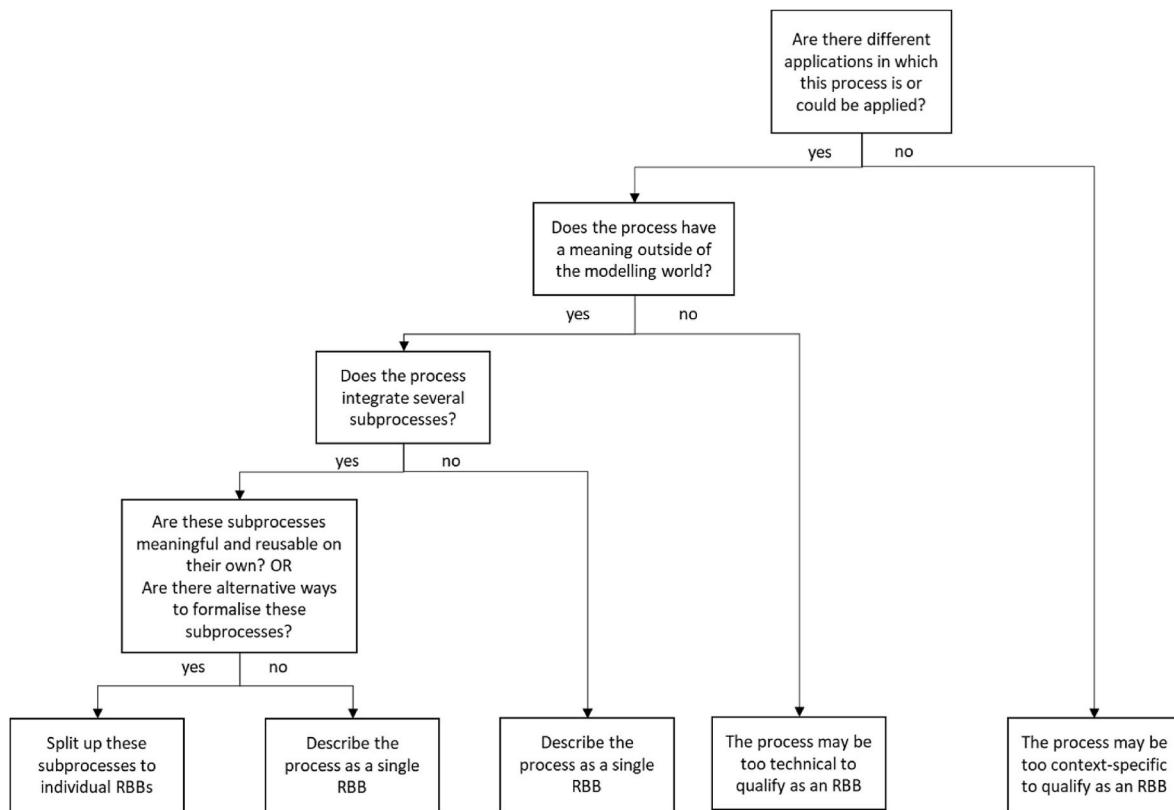
Fig. 4. Decision tree for identifying and scoping RBBs. It guides contributors in assessing whether a mechanism qualifies as a RBB and whether it should be represented as a single RBB or decomposed into multiple building blocks. Boundary examples this tree emerged from, and which can be used to demonstrate how to apply this decision tree, are presented in the Supplementary Material S.3 .
