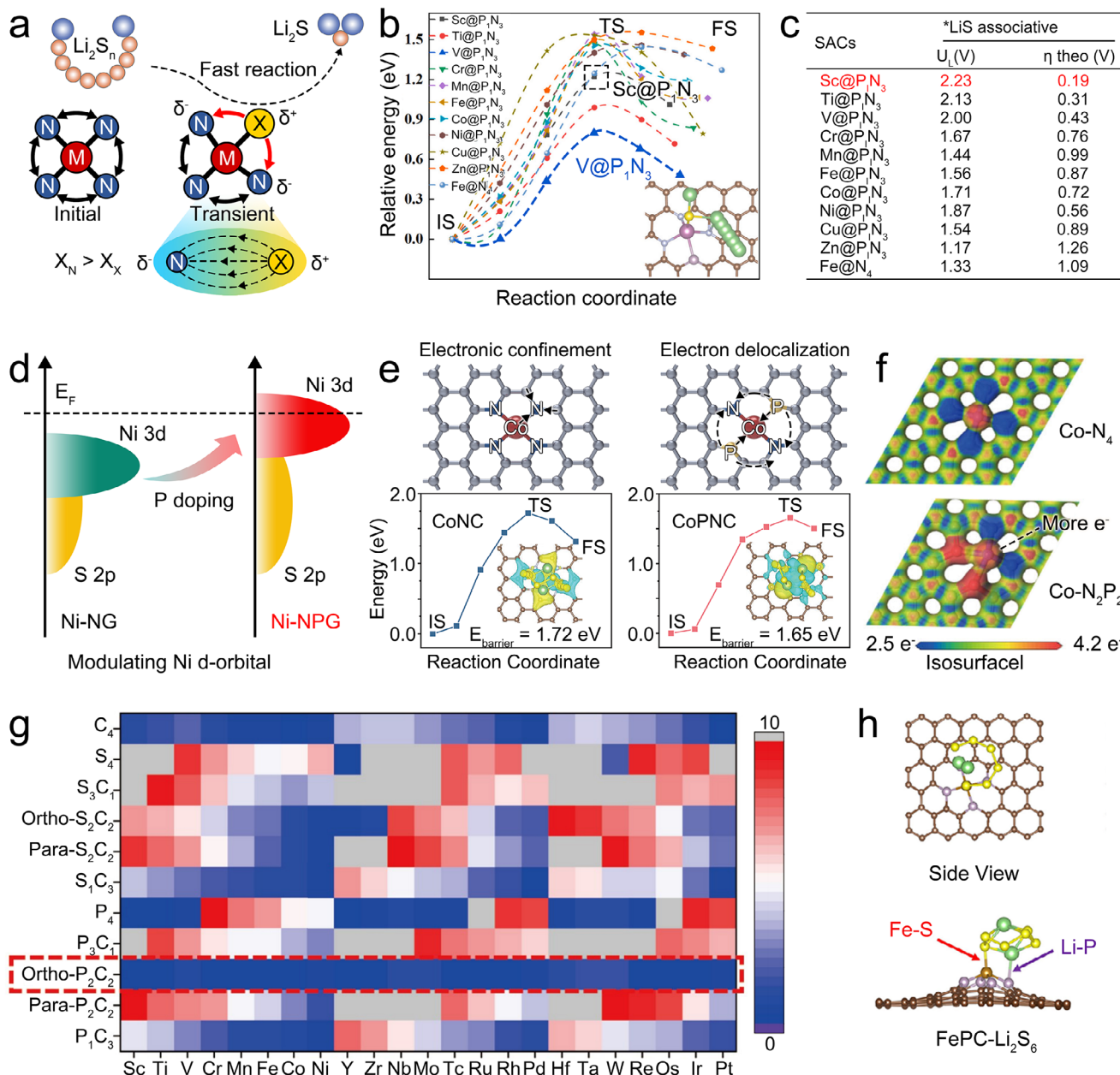
FIGURE 4 | (a) Mechanism diagram for accelerated sulfur redox by weakly electronegative coordination atoms. (b) Relative energy of \text{Li}_2\text{S} conversion on the \text{TM@N}_3\text{P}_1 . (c) Theoretical overpotentials and ultimate potential values of \text{TM@N}_3\text{P}_1 applied in \text{Li}_2\text{S}_2 reduction. Reproduced with permission [78]. Copyright 2024, Elsevier B.V. (d) Schematic of the Ni d-orbitals near the Fermi level and the S p-orbitals structure. Reproduced with permission [81]. Copyright 2025, Wiley-VCH GmbH. (e) Decomposition energy barrier of \text{Li}_2\text{S} conversion on the \text{Co-N}_4 and \text{Co-N}_2\text{P}_2 . Reproduced with permission [86]. Copyright 2024, Wiley-VCH GmbH. (f) Differential electron density images. Reproduced with permission [88]. Copyright 2025, Springer Nature. (g) Overpotential of SACs covering 3d, 4d, and 5d transition metals with different coordination structure. Reproduced with permission [82]. Copyright 2024, Springer Nature. (h) Schematic diagram of \text{Li}_2\text{S}_6\text{-Fe-P}_4 . Reproduced with permission [93]. Copyright 2025, Wiley-VCH GmbH.
