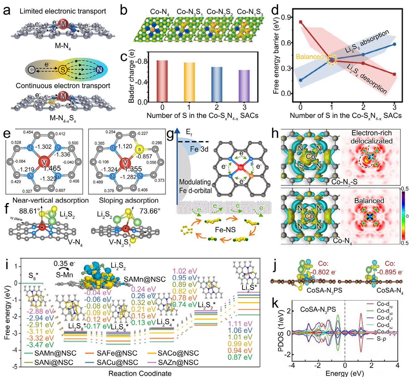
FIGURE 5 | (a) Schematic mechanism of local charge redistribution induced by substituting N with weakly electronegative S heteroatom. (b) Differential electron density image of Co–N 4-x S x . (c) Bader charge of Co in Co–N 4-x S x . (d) Free energy barrier of Li 2 S n absorption/desorption on Co–N 4-x S x . Reproduced with permission [95]. Copyright 2025, Elsevier B.V. (e) Bader charge numbers of atoms in V–N 4 and V–N 3 S 1 . (f) The adsorption optimized structure of Li 2 S 2 on the V–N 4 and V–N 3 S 1 . Reproduced with permission [96]. Copyright 2024, Wiley-VCH GmbH. (g) Schematic illustration of the working mechanism of FeSAC-NS. Reproduced with permission [98]. Copyright 2025, Elsevier B.V. (h) Differential charge density of Co–N 4 and Co–N 3 S. Reproduced with permission [100]. Copyright 2025, American Chemical Society. (i) Gibbs free energy diagrams of sulfur species reduction. Reproduced with permission [101]. Copyright 2024, Elsevier B.V. (j) Differential charge density and (k) PDOS of Co-d orbitals and S-p orbitals. Reproduced with permission [102]. Copyright 2024, Wiley-VCH GmbH.
