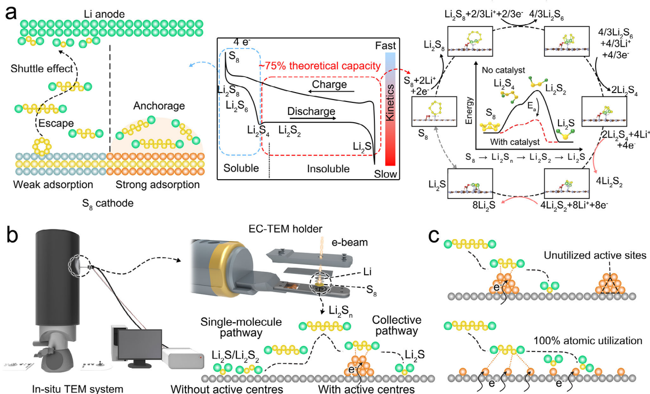
FIGURE 1 | (a) Schematic illustration of LiPSs conversion mechanisms with/without electrocatalysts. (b) Schematic diagram for LiPSs conversion within/without the electrocatalysts. (c) Schematic illustration comparing the low active site utilization of nanoparticle catalysts and nearly full atomic utilization of SACs.
