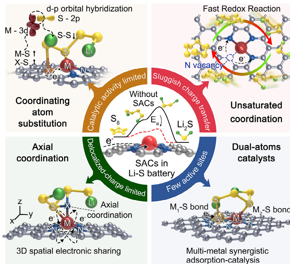
FIGURE 11 | Design logic of metastable SACs coordination.
