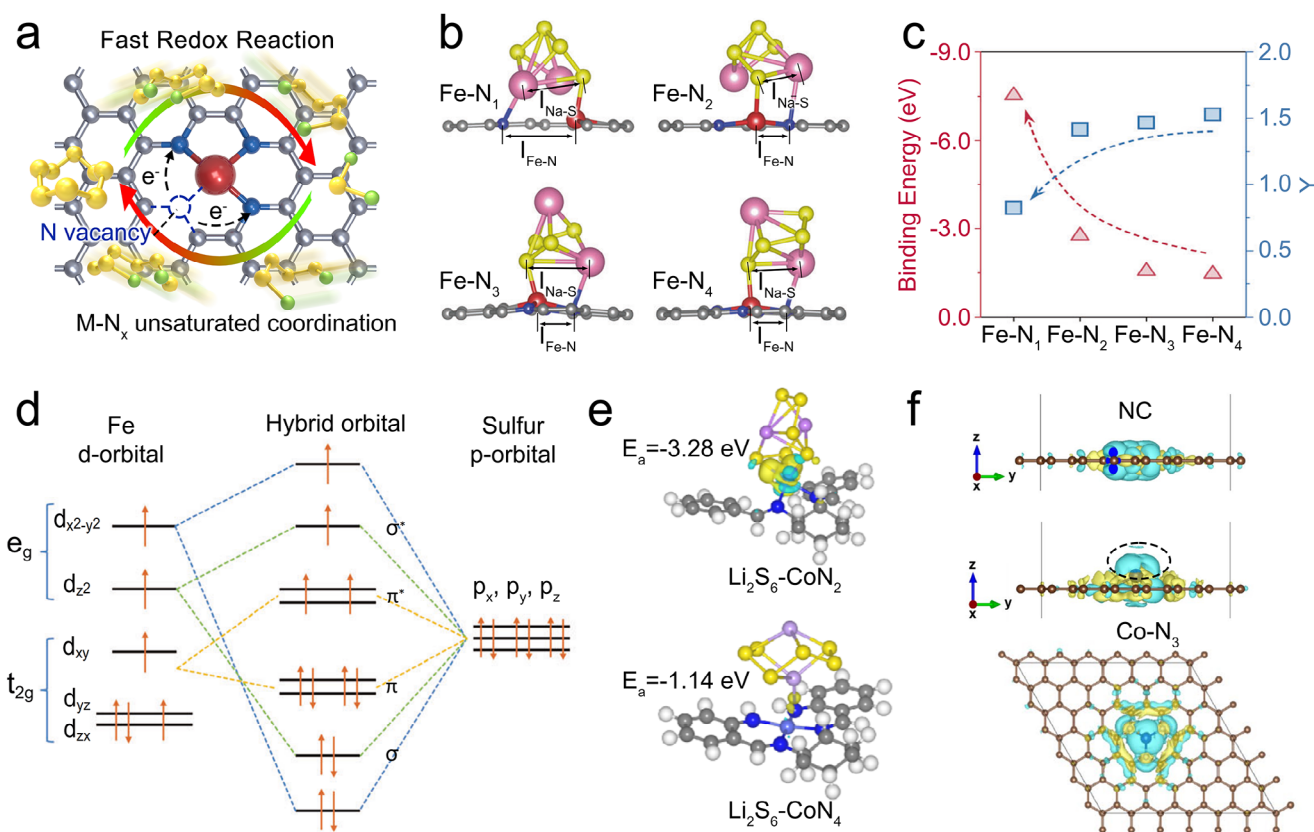
FIGURE 6 | (a) Schematic diagram for boosted LiPSs redox via unsaturated M-N x coordination. (b) Configurations of Na 2 S 4 adsorbed on Fe-N x . (c) relationships among unsaturation degrees of Fe-N x , binding energies, and geometric structure descriptors. (d) Schematic for the d-p orbital hybridization between Fe-N x and sulfur species. Reproduced with permission [110]. Copyright 2025, Springer Nature. (e) Adsorption of Li 2 S 6 -CoN 2 and CoN 4 . Reproduced with permission [55]. Copyright 2025, American Chemical Society. (f) Differential charge density of Co-N 3 . Reproduced with permission [111]. Copyright 2025, Springer Nature.
