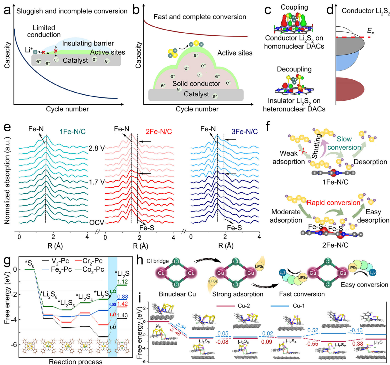
FIGURE 8 | (a) Problems and (b) potential solution for solid-phase conversion reactions. (c) Comparison of the coupling of the homo- and heteronuclear DACs. (d) Influence of orbital hybridization between conductor \text{Li}_2\text{S}_2 and DACs. Reproduced with permission [124]. Copyright 2026, Springer Nature. (e) Operando FTEXAFS spectra of the Fe K-edge recorded. (f) Schematic of the SRR process on Fe-based catalysts. Reproduced with permission [123]. Copyright 2024, American Chemical Society. (g) Calculated free energy diagram. Reproduced with permission [125]. Copyright 2025, Elsevier B.V. (h) LiPSs conversions catalyzed by Cu-1 and Cu-2. (i) Calculated free energy diagram. Reproduced with permission [127]. Copyright 2024, Springer Nature.
