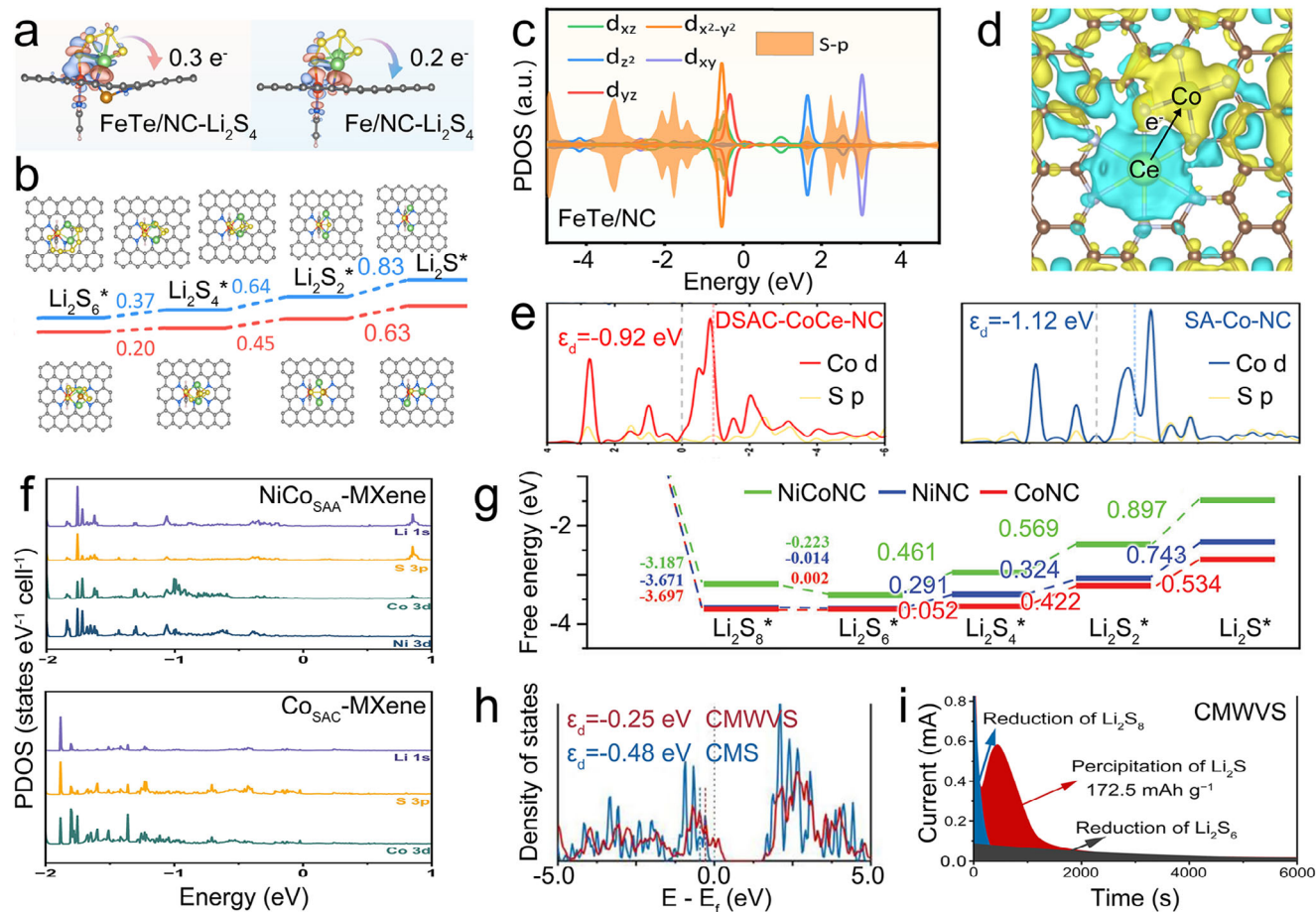
FIGURE 10 | (a) Charge density difference of \text{Li}_2\text{S}_4 -FeTe/NC and \text{Li}_2\text{S}_4 -Fe/NC. (b) Free energy profiles for the conversion of LiPSs. (c) PDOS of \text{Li}_2\text{S}_4 -FeTe/NC. Reproduced with permission [149]. Copyright 2025, Springer Nature. (d) Charge density difference and (e) PDOS of Ce-Co DACs. Reproduced with permission [152]. Copyright 2025, American Chemical Society. (f) PDOS of Ni-Co DACs and Co SACs. Reproduced with permission [154]. Copyright 2025, Tsinghua University Press. (g) Free energy profiles for the conversion of LiPSs. Reproduced with permission [156]. Copyright 2024, Wiley-VCH GmbH. (h) PDOS of CMWVS and CMS. (i) \text{Li}_2\text{S} nucleation experiment. Reproduced with permission [157]. Copyright 2026, Springer Nature.
