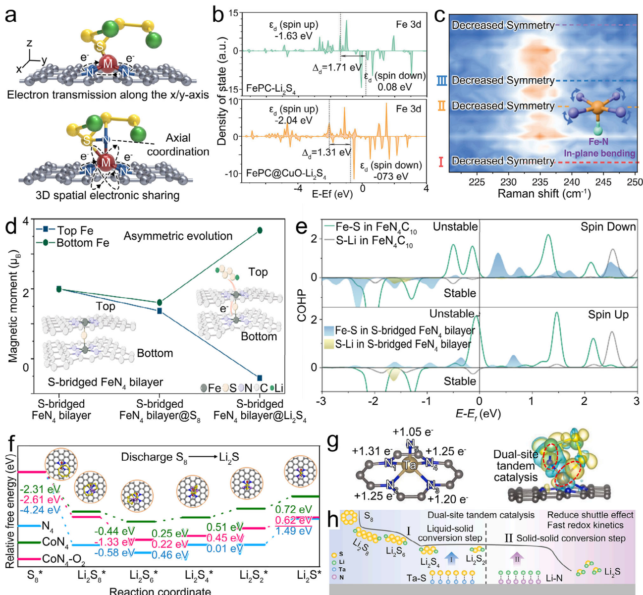
FIGURE 7 | (a) Schematic illustration of axial coordination atoms inducing local electron redistribution. (b) Density of state. (c) In-situ Raman. Reproduced with permission [114]. Copyright 2024, Wiley-VCH GmbH. (d) Comparison of magnetic moments of the top and bottom Fe atoms under different conditions. (e) COHP analysis of Fe-S and Li-S bonds in the S-bridged FeN 4 bilayer and FeN 4 C 10 structures. Reproduced with permission [116]. Copyright 2025, American Chemical Society. (f) Calculated free energy diagram. Reproduced with permission [117]. Copyright 2025, American Chemical Society. (g) Bader charge numbers of coordination atoms of Ta-N 5 . (h) Schematic illustration of the mechanism of dual-site Ta-N 5 catalysis. Reproduced with permission [119]. Copyright 2025, Elsevier B.V.
