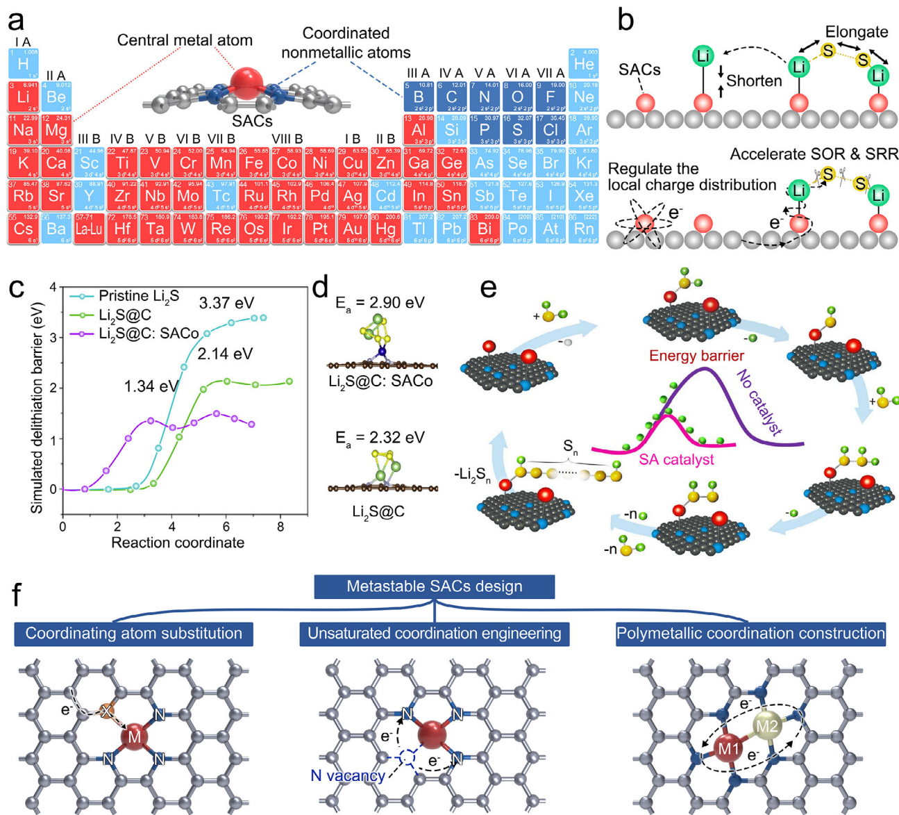
FIGURE 2 | (a) Schematic diagram for atomic screening of SACs. (b) Schematic diagram for accelerated LiPSs redox on the SACs. (c) Comparison of simulated delithiation energy barrier of \text{Li}_2\text{S} . (d) Adsorption energy of \text{Li}_2\text{S}_4 on NC with/without Co SACs. Reproduced with permission [43]. Copyright 2020, Elsevier B.V. (e) A proposed mechanism for SACs catalyzed \text{Li}_2\text{S} delithiation reaction. Reproduced with permission [44]. Copyright 2019, Elsevier B.V. (f) Design logic of metastable SACs coordination structure.
