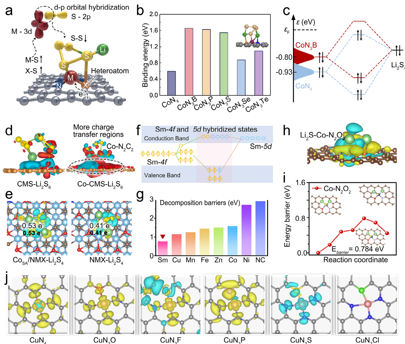
FIGURE 3 | Mechanism diagram for LiPSs redox on the M-N 3 X. (b) Binding energy of Li 2 S 4 -Co-N 3 X. (c) Scenario of d-p orbital hybridization for Li 2 S 4 -Co-N 3 B and Li 2 S 4 -Co-N 4 . Reproduced with permission [65]. Copyright 2024, Elsevier B.V. (d) Electron density difference of Li 2 S 6 -CMS with/without Co-N 2 C 2 . Reproduced with permission [69]. Copyright 2025, Elsevier B.V. (e) Electron density difference. Reproduced with permission [71]. Copyright 2025, Wiley-VCH GmbH. (f) Schematic diagram of mott transition of electrons from 4f to 5d-orbitals. (g) Decomposition energy barriers of Li 2 S on SACs. Reproduced with permission [72]. Copyright 2024, Wiley-VCH GmbH. (h) Electron density difference of Li 2 S-Co-N 2 O 2 . (i) Decomposition energy barriers of Li 2 S on Co-N 2 O 2 . Reproduced with permission [73]. Copyright 2024, Elsevier B.V. (j) Electron density difference of M-N 3 X. Reproduced with permission [75]. Copyright 2025, American Chemical Society.
