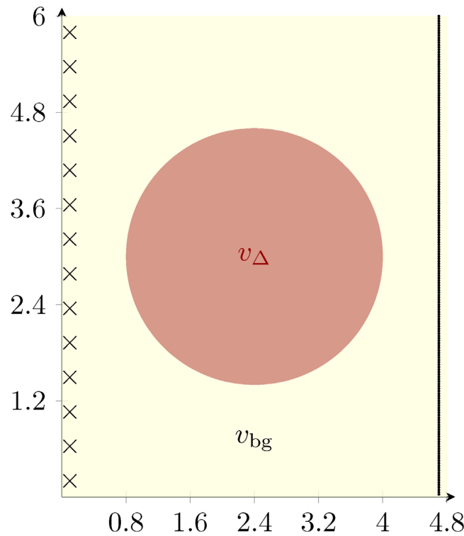
FIGURE 1 | Geometry of the Camembert model: sources (marked by \times ), inclusion (colored red), and the receivers on the line at the right. [Colour figure can be viewed at wileyonlinelibrary.com ]
