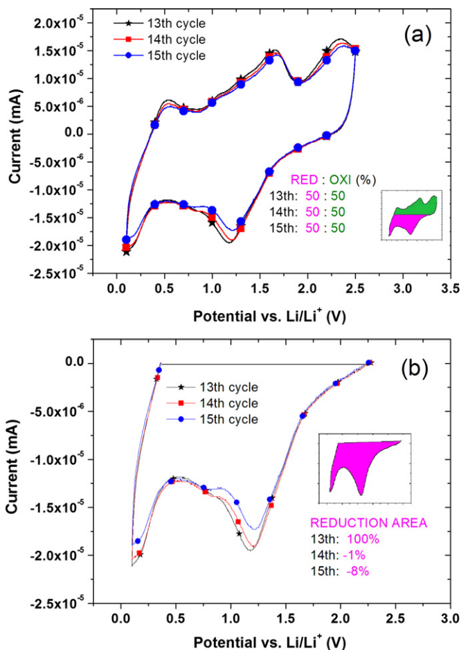
Fig. 6. (a): Three whole cycles by cyclic voltammetry after CE = 100% at a voltage rate of 0.1 \text{ V s}^{-1} and the ratio of the integrated reduction area to the oxidation area. The measured current resolution and accuracy is about \pm 0.2\% , so that the error bar is smaller than the line symbols used. Therefore, the uncertainty of the integrated areas is almost negligible. (b): Three discharge cycles and their reduction areas. Symbols are representing only a few of the measured data points to distinguish between the cycles.
