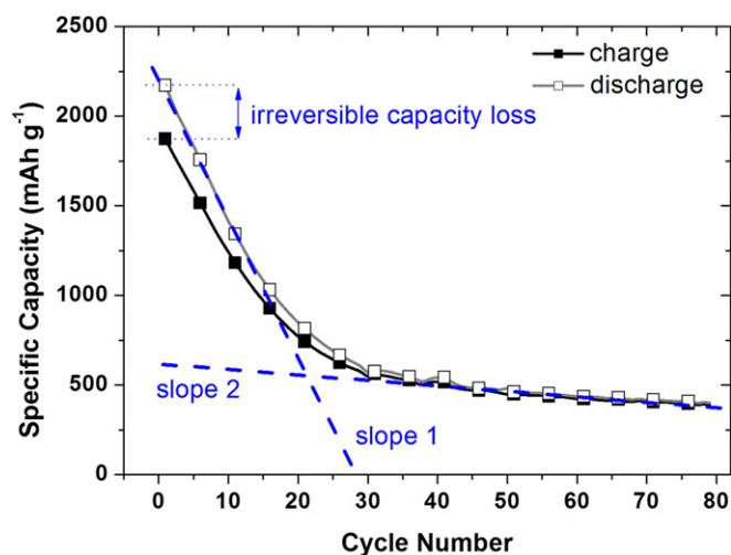
Fig. 1. Typical charge and discharge capacities of a SnO 2 nanoparticle layer electrode. For the first cycles an irreversible capacity loss can be observed. In parallel, a steep slope (1) can be observed until CE reaches 100% and a shallow slope (2) describes the cycling behavior after CE reaches 100%.
