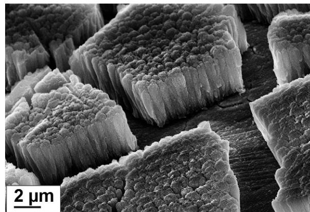
Fig. 4. Ex-situ SEM image of a \text{SnO}_2 -nanoparticle electrode after the first cycle. The building of new, fresh surface area, due to the large volumetric changes accompanied by film break off, is evident from this image.
