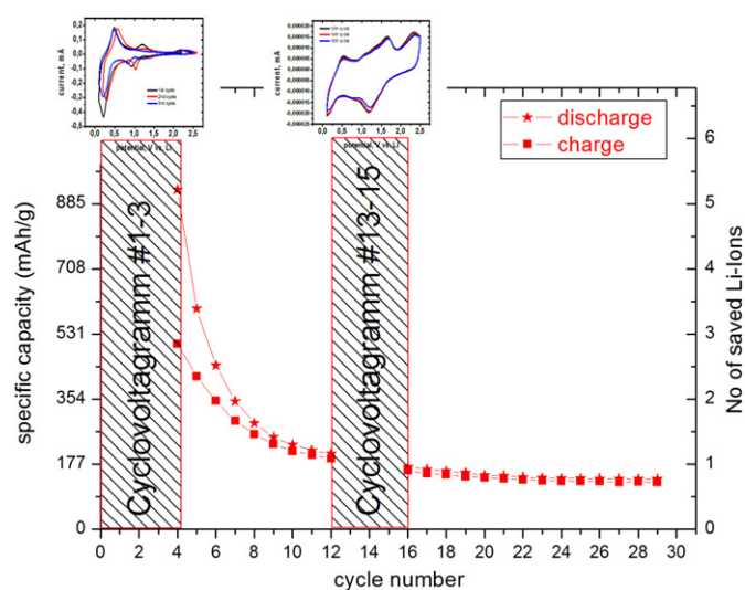
Fig. 5. Result of the cycling treatment: first three cycles with cyclic voltammetry at a voltage rate of 0.1 \text{ mV s}^{-1} , subsequent long term cycling measurements until a CE of about 100% is reached, using a constant current density of 40 \text{ mA g}^{-1} and, finally, again three cycles with cyclic voltammetry and final long term cycling measurements until the 30th cycle is reached.
