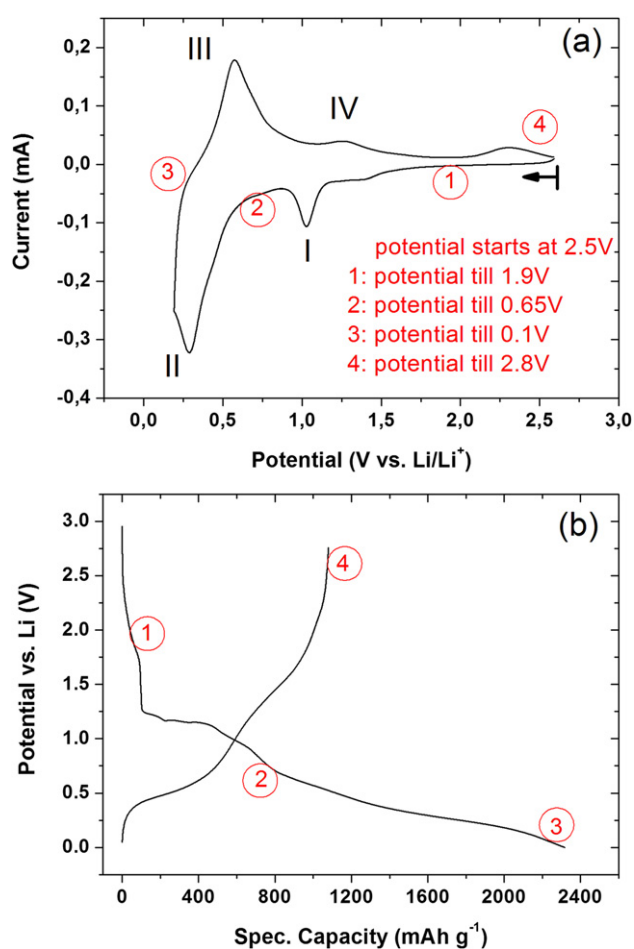
Fig. 2. Typical cyclic voltammogram (a) and voltage profile (b), showing the relevant reactions (I–IV) during cycling and the potential, where ex-situ XPS samples were taken (samples 1–4).
