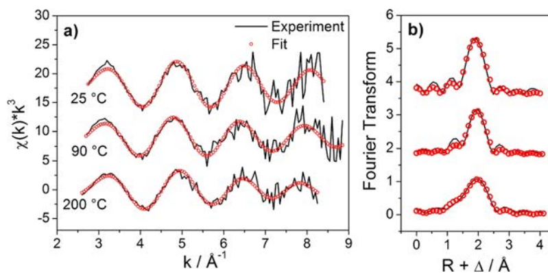
Figure 9. k^3 weighted Am L III edge EXAFS spectra (a) and related Fourier transforms (b) at T = 25, 90, and 200 °C.
