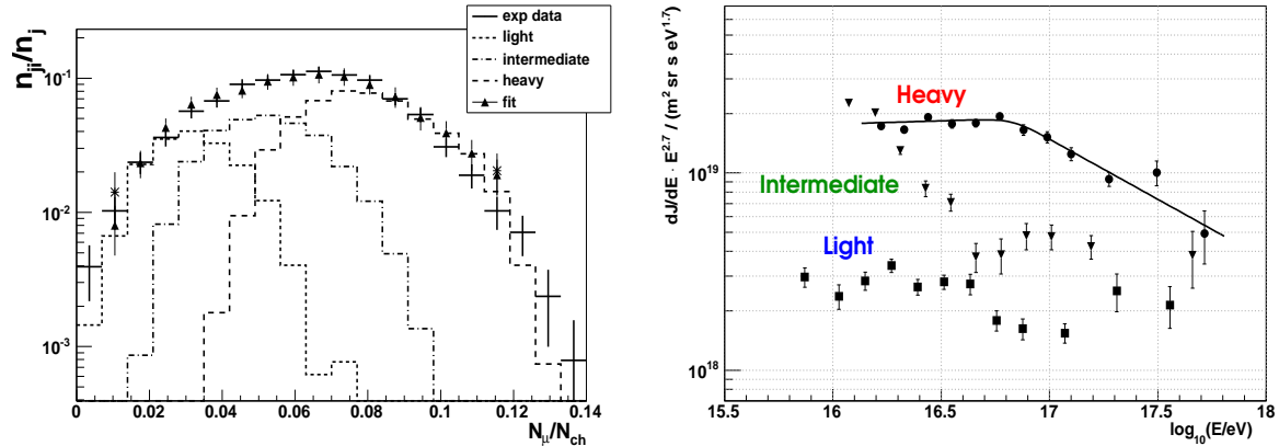
Figure 7: Left panel: An example of an experimental N_{\mu}/N_{ch} distribution (solid line) for the interval 7.15 \leq \log_{10} N_{ch} < 7.24 (data has been normalized dividing by the total number of events in the histogram). The result of the fit (triangles) with the simulated distributions (based on CORSIKA/QGSJET II-03 [29]) for the light (thin-dashed line), intermediate (dot-dashed line) and heavy (thick-dashed line) mass groups is shown. Right panel: Energy spectra for the light, intermediate and heavy mass groups derived from experimental data using the technique described in section 4.2.3 [30]. Data was interpreted using QGSJET II-03.
