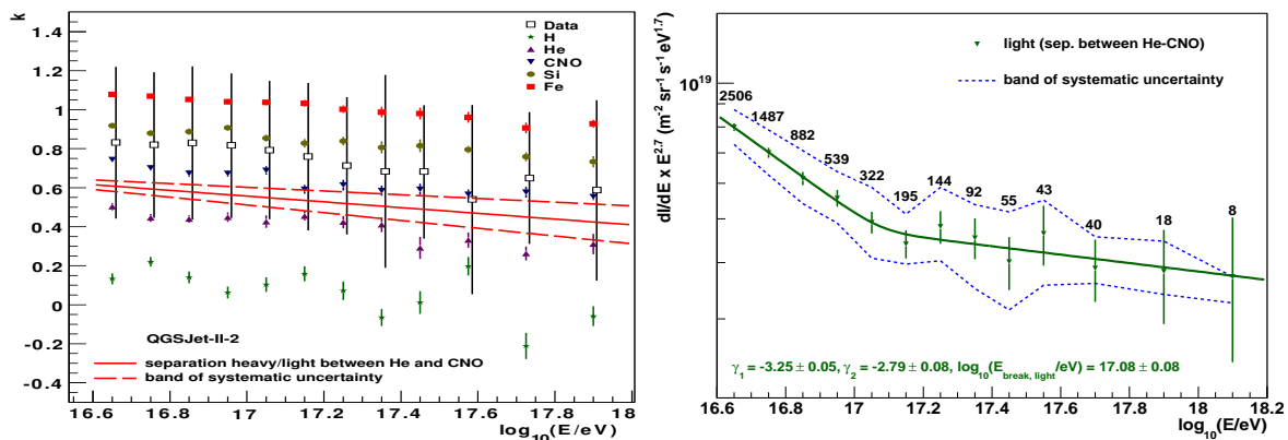
Figure 5: Left panel : Mean k parameter vs reconstructed energy for different primaries according to MC simulations (CORSIKA/QGSJET II) for the analysis of [21]. The thick line represents the frontier line used for classification of experimental data into different mass groups and the thin lines, the corresponding uncertainties on the definitions. Statistical and reconstruction uncertainties of k are shown as error bars. Right panel : Experimental energy spectrum for light primaries according to the analysis of [21] based on the k technique. Error bands are obtained by considering the changes in the spectra introduced by varying the frontier lines inside their respective interval of uncertainties. Statistical uncertainties appear as error bars.
