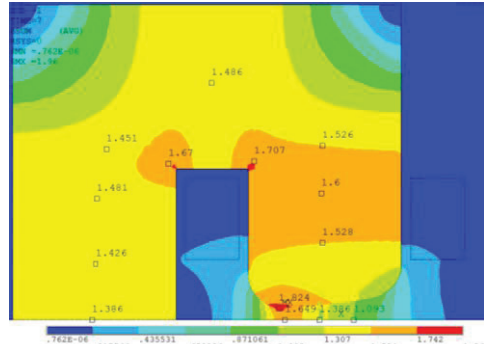
Figure 9: Field map of gradient bending magnet.
