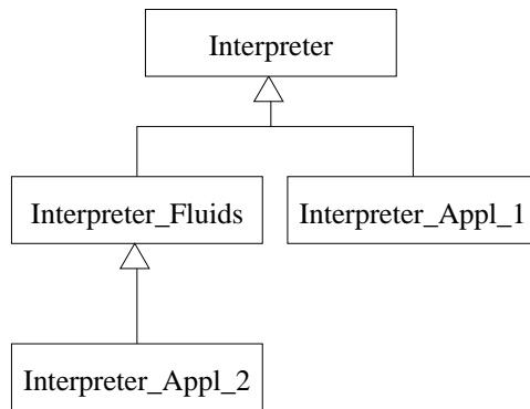
Figure 5: Interpreter usage
