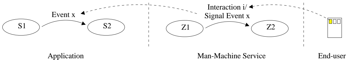
Figure 3: User interaction
