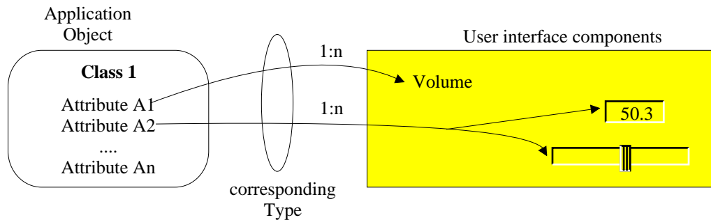
Figure 2: Visualization of application objects
