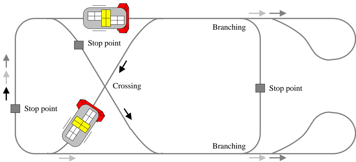
Figure 6: Simulator for a driverless transport system
