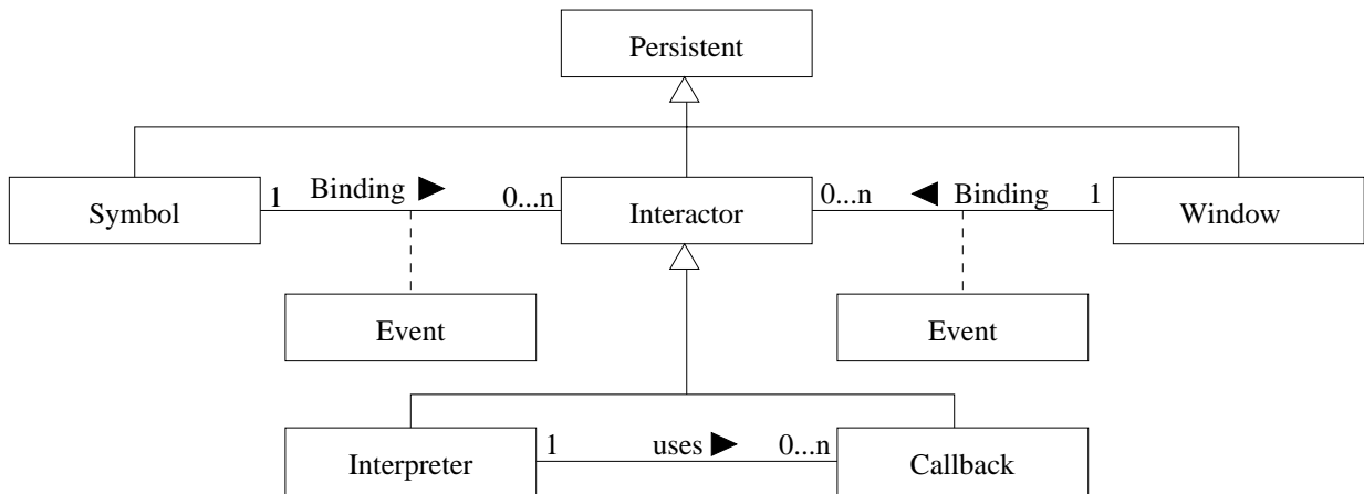
Figure 4: Behavior model
