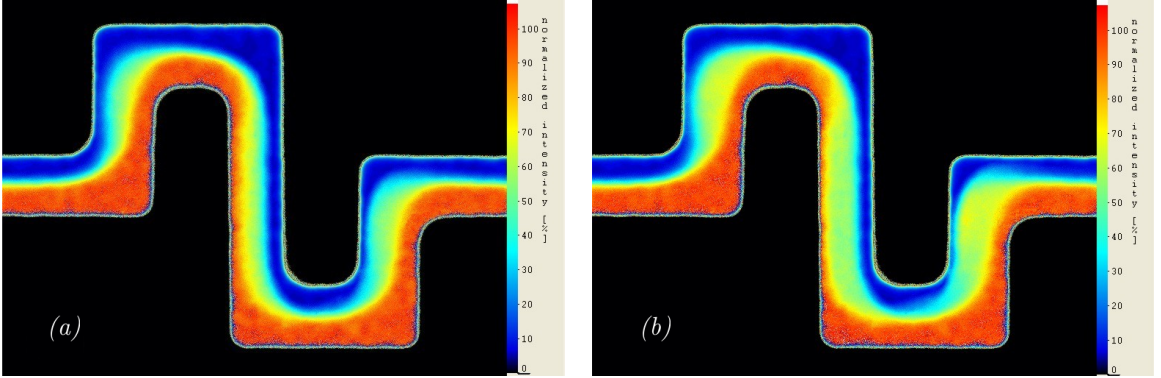
Figure 5.1: Concentration fields of flows at (a) Re=27 and (b) Re=42 within the meander part of the micromixer.
