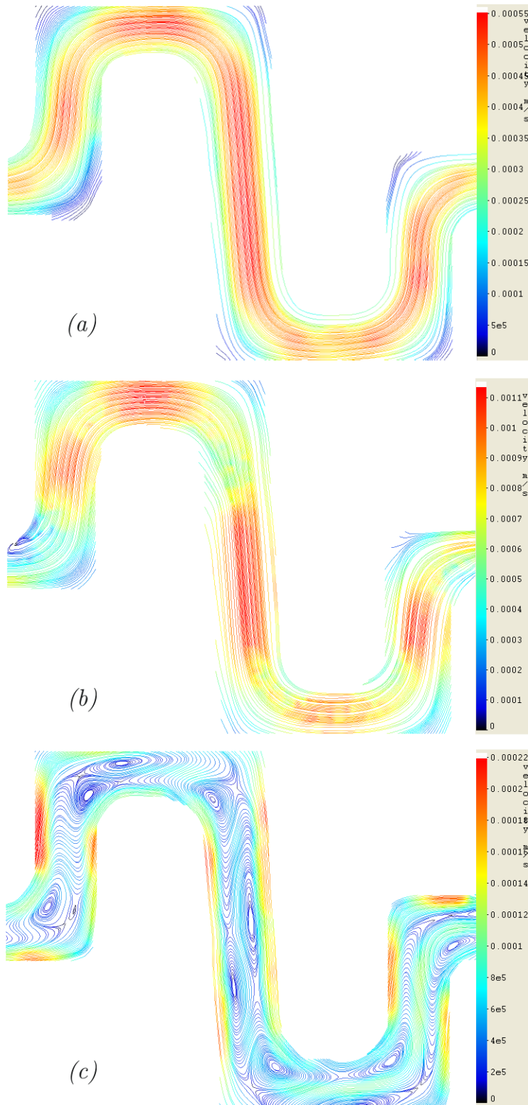
Figure 5.14: Streamlines of (a) a pressure-driven flow for Re=0.07 at level 2z/d = -0.37 . (b) and (c) are obtained with an additional electrical field of amplitude 14.5 V/mm. The electrical field is either (b) in the direction of the pressure-driven flow or (c) against the direction of the pressure-driven flow.
