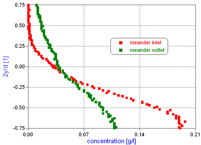
Figure 5.20: Concentration profiles at the meander inlet (line i , red) and the meander outlet (line o , green) for a gravity-driven flow at Re=0.1 .
