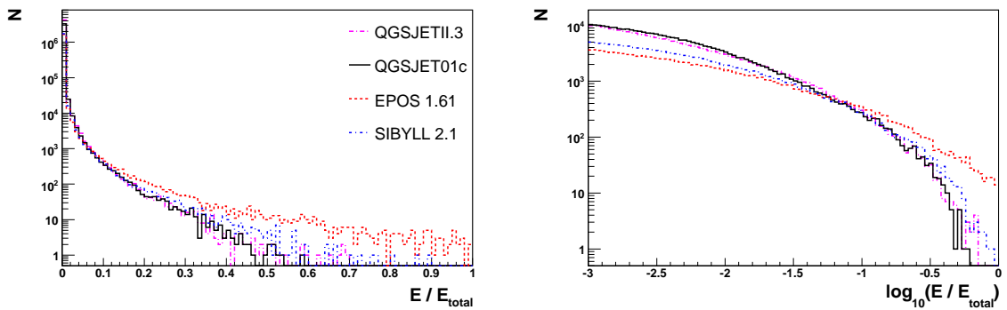
(b) electromagnetic secondaries ( e^\pm , \gamma and \pi^0 )
