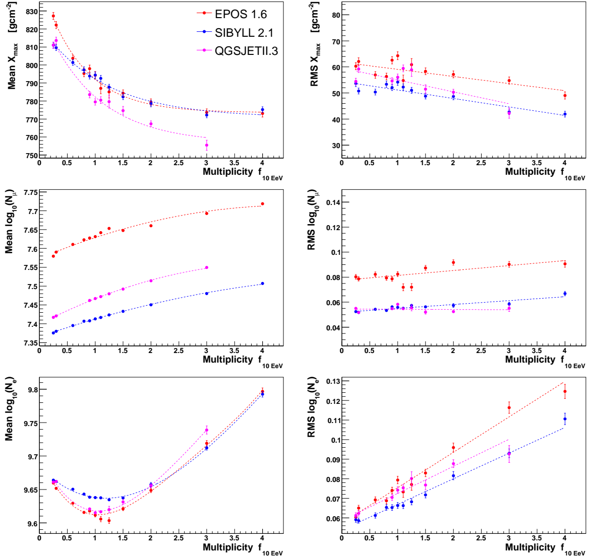
Figure 4.3: Impact of a modified secondary multiplicity on the mean and RMS of the observables X_{\max} , N_e(X_{\text{obs}} = 1000 \text{ gcm}^{-2}) and N_{\mu}(X_{\text{obs}} = 1000 \text{ gcm}^{-2}) for proton initiated air showers at 10 EeV. The dashed lines are just to guide the eye.
