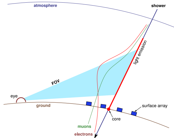
Figure 3.17: The hybrid detector simulation needs to calculate light emission, propagation in a curved atmosphere and the telescope response as well as the signal and timing induced by the air shower in the surface detectors. Detector simulations are based on generated longitudinal profiles of \frac{dE}{dX} , electron and muons.
