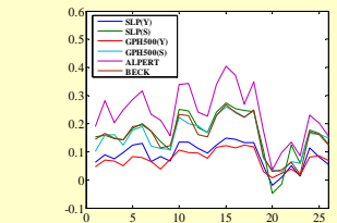
Figure 2: Skill score for rainfall modelling of the 26 observation stations in the Jordan region (see Fig. 1 for the location of the stations).
