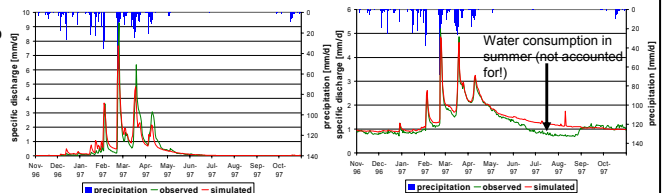
Simulated and observed discharge at the gauges Saar (left) and Yoseph Bridge (right)
