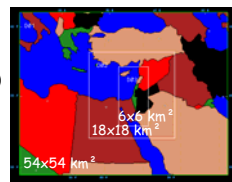
Domain Setup of MM5
