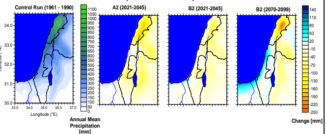
Mean annual temperature (above) and mean annual precipitation (below) for the control run and changes in the future for the scenarios A2 and B2 in different time slices (results of domain2)
