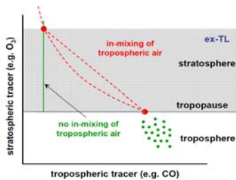
Fig. 1: Schematic view of a typical tracer correlation around the extratr. tropopause
