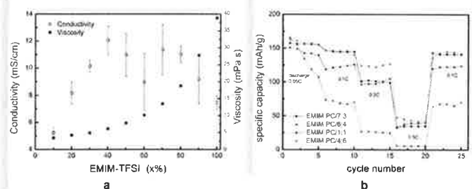
(a) ionic conductivity (at room temperature) and viscosity (at 20 °C) of EMIM-TFSI mixed with PC; (b) specific capacity of electrolytes with different PC content at room temperature in swagelok cells using NMC/Li + as electrodes, discharged at variable C-rates between 3.0 and 4.3 V.
