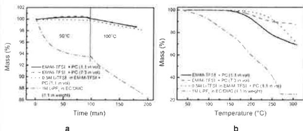
Thermogravimetric Analysis (TGA) of electrolyte mixtures (a) isothermal mass change at 50 °C and 100 °C. Exposition time : 90 min. (b) mass change between room temperature and 300 °C, heating :10 K/min.
