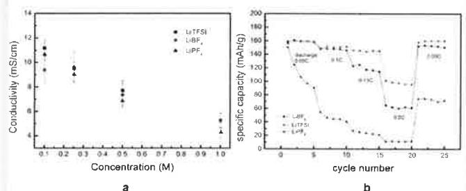
(a) ionic conductivity of mixture EMIM-TFSI+PC (7:3 in vol.) with different lithium salts at room temperature; (b) specific capacity of electrolyte with different lithium salts at room temperature in swagelok cells using NMC/Li + as electrodes, discharged at variable C-rate between 3.0 and 4.3 V
