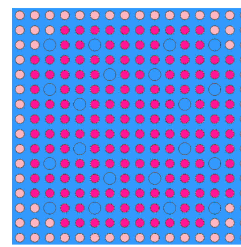
Composition of a 18x18-24 MOX Fuel Assembly
