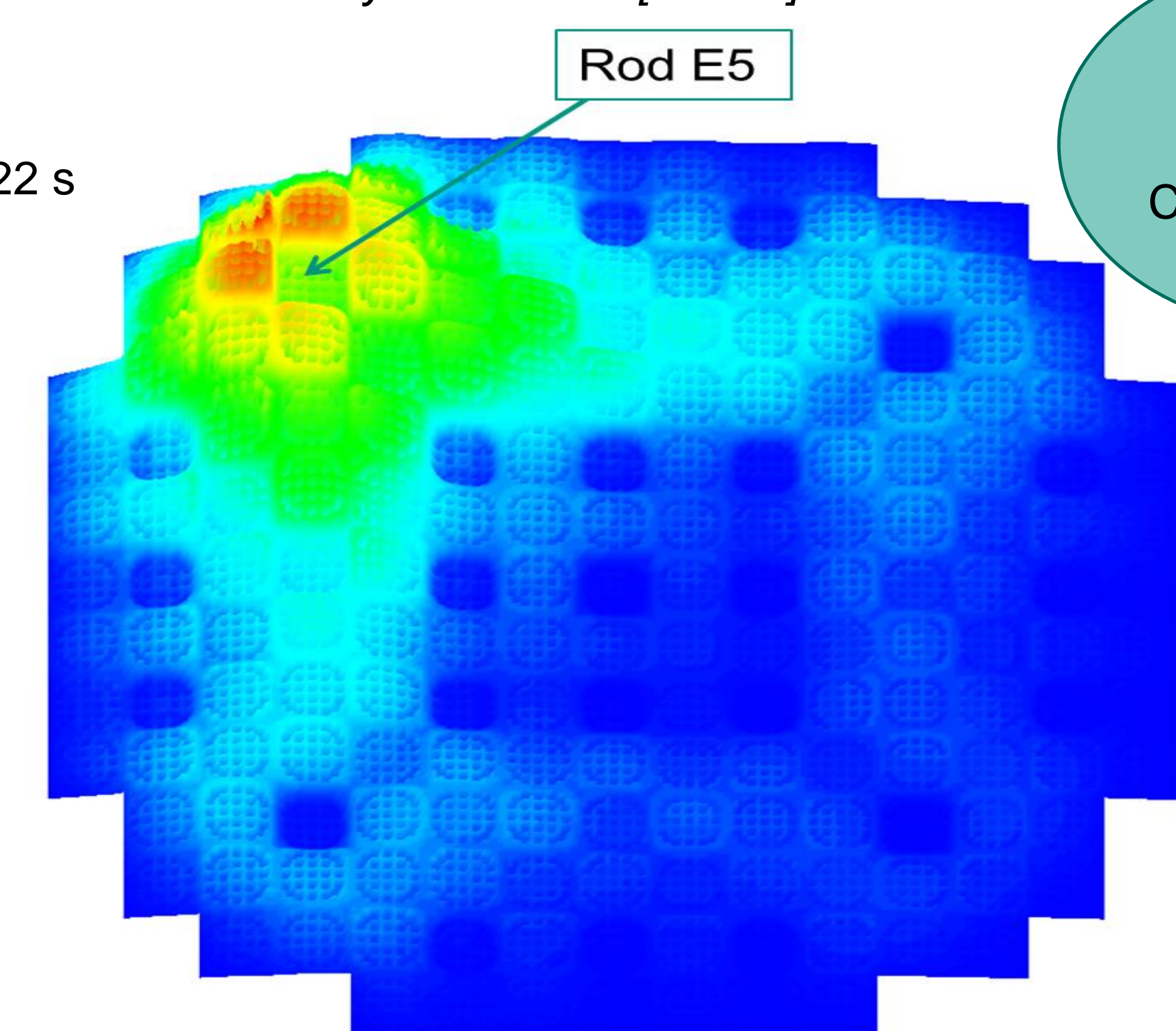
HZP rod ejection accident (REA): axially cumulated power density distribution [W/cm 3 ] at 0.22s
