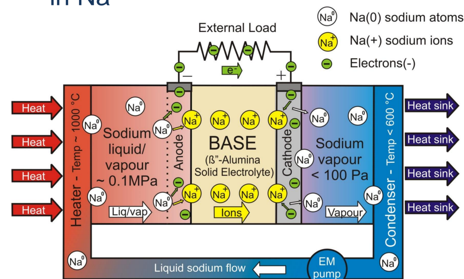
Operation principle of AMTEC
