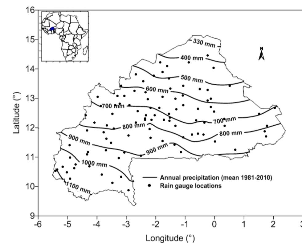
Fig. 1: Annual rainfall distribution and rain gauges locations in Burkina Faso
