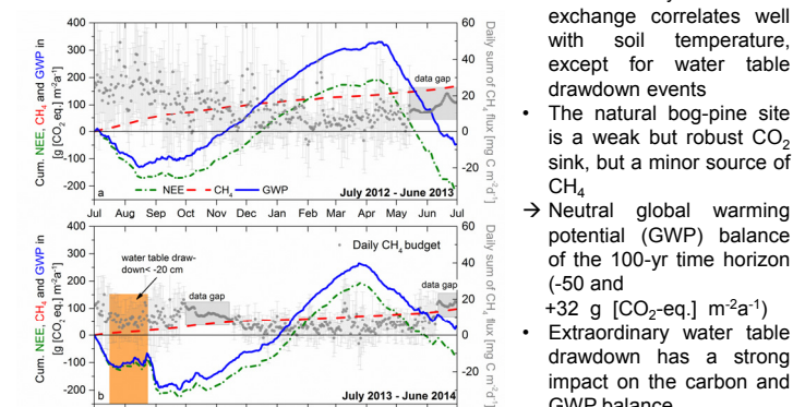
Fig. 5 Annual cumulative NEE, CH 4 and GWP exchange and the daily sum of methane exchange from July 2012-June 2014.
