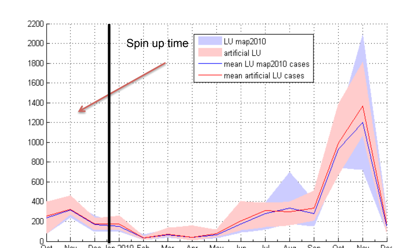
Fig.4a Precipitation of 15 perturbation runs with LU map 2010 (blue) and artificial LU (red) at Da Nang station
