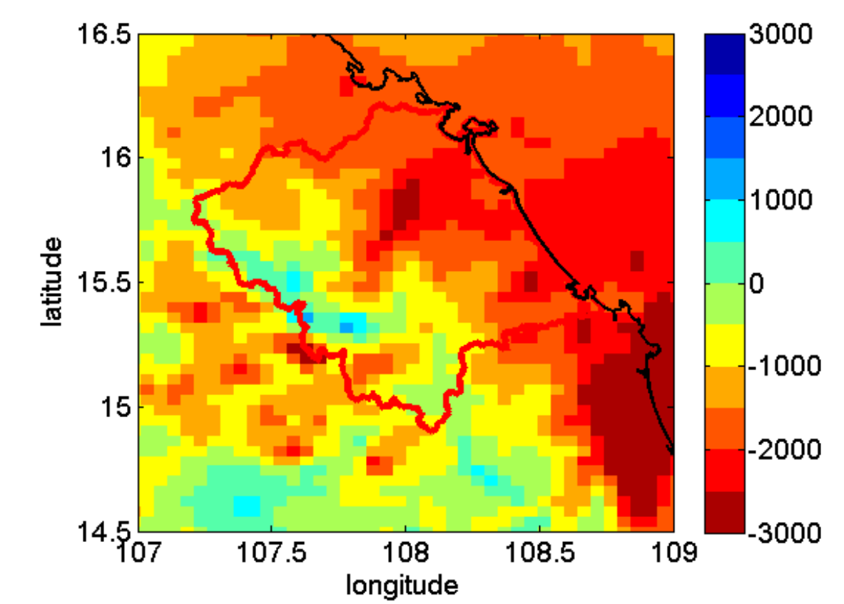
Fig.5b Difference of mean precipitation values of 15 perturbation runs with LU default and artificial LU (LUC minus default)
