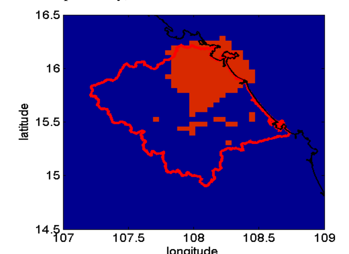
Fig.3d t-test for temperature based on 15 perturbation runs (h=1: reject, h=0: failure to reject)
