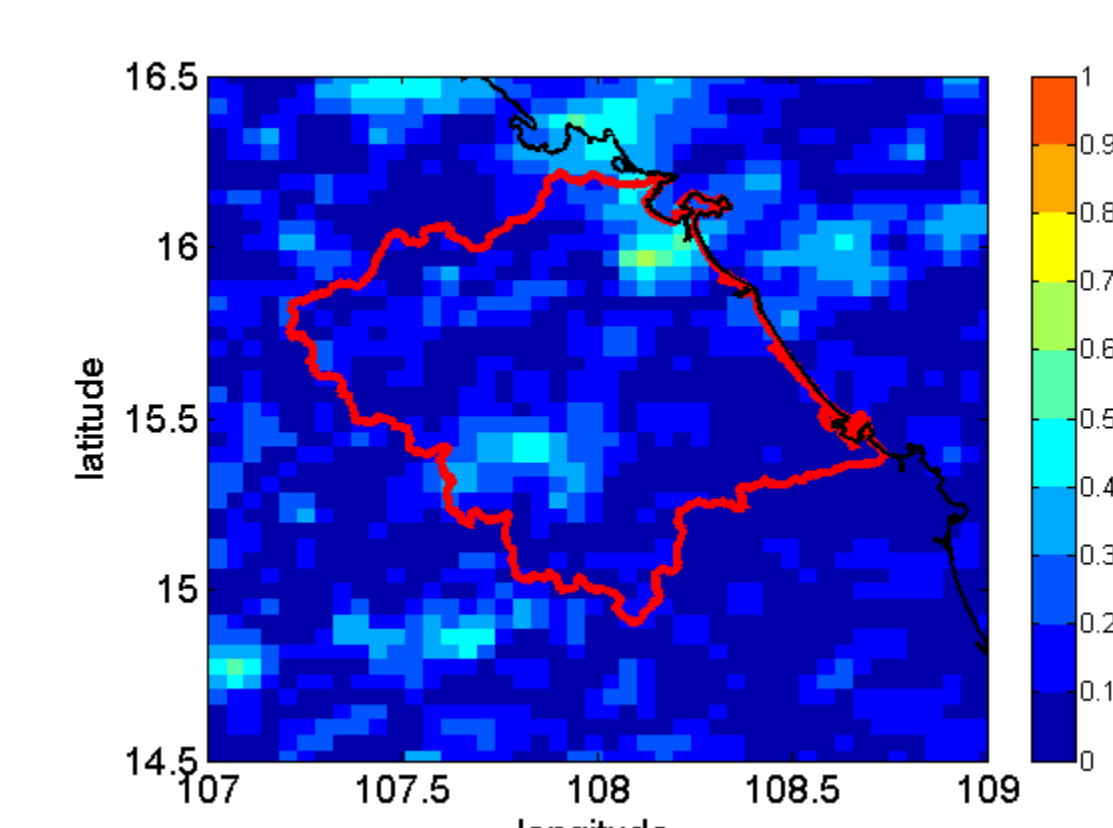
Fig.4b Signal-to-noise ratio for precipitation based on 15 perturbation runs
