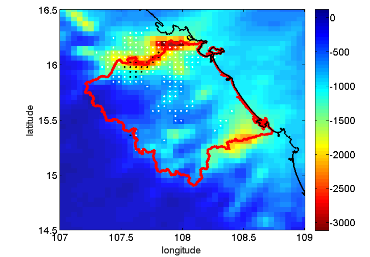
Fig.5d Difference of mean precipitation values of 15 perturbation runs with LU default and artificial LU in November 2001 (LUC minus default). Dots indicate a significant (alpha = 90 (black) and alpha = 80 (white)) signal-to-noise ratios based on bootstrapping test
