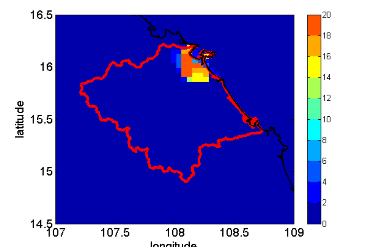
Fig.3c Signal-to-noise ratio for surface temperature based on 15 perturbation runs
