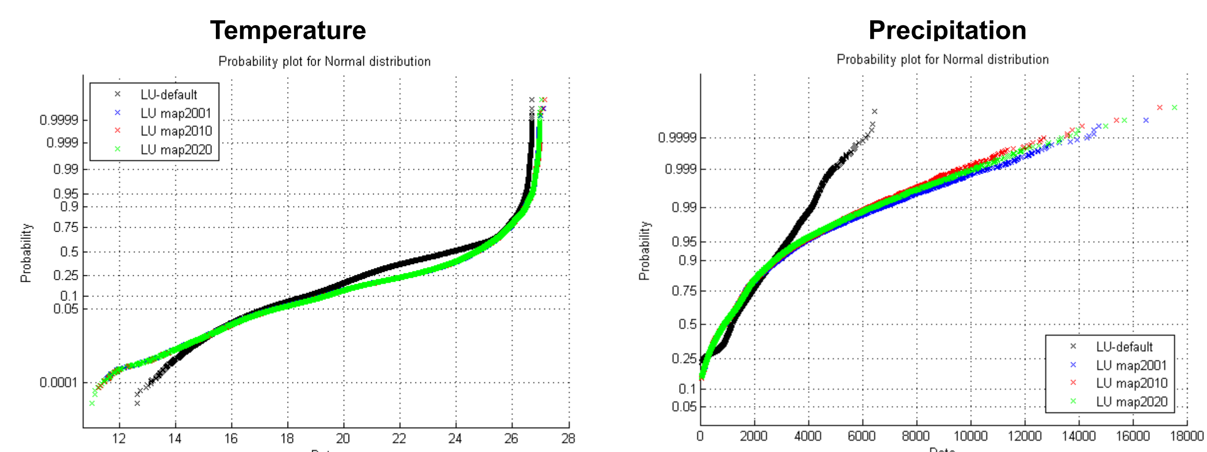
Fig.6 Probability of surface temperature (left) and precipitation (right) for domain 3 for the period 2011 to 2020 with WRF default LU map, observed maps 2001 and 2010, and projected map 2020
