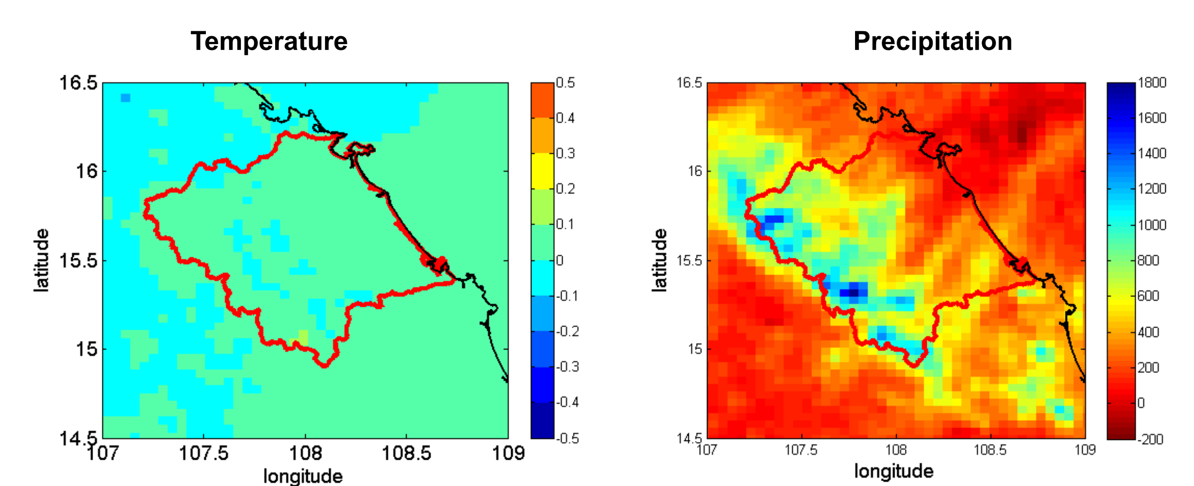
Fig.7 Difference of mean annual surface temperature (left) and mean annual precipitation (right) using observed LU map 2001 between the period 2001-2010 and period 2011-2020 (2011-2020 minus 2001-2010)
