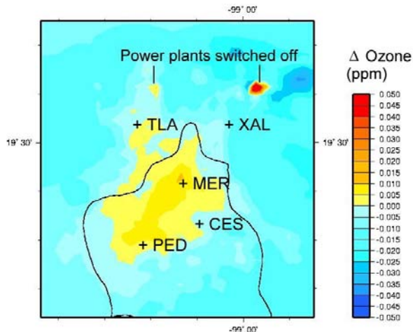
Szenario- simulation (MCCM)
