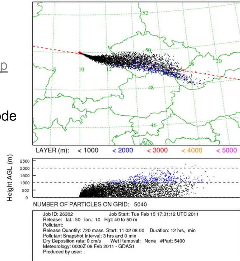
NOAA HYSPLIT MODEL PARTICLE CROSS-SECTIONS PARTICLE POSITIONS AT 12 UTC 08 Feb 11
