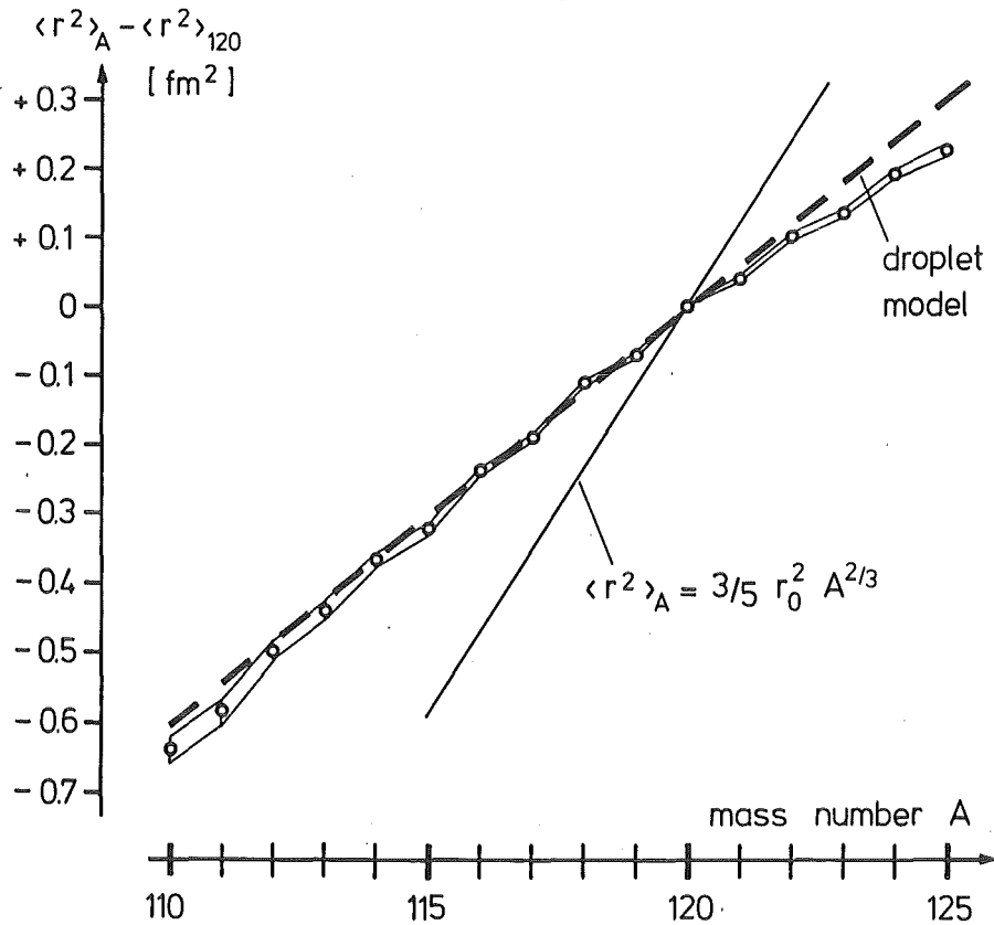
FIG. 3. The variation of the mean square charge radii of Sn nuclei with the mass number A as compared to the droplet model prediction. The systematic uncertainty arising from the calibration of the experimental data is indicated by an "error band" enclosing the data points.
