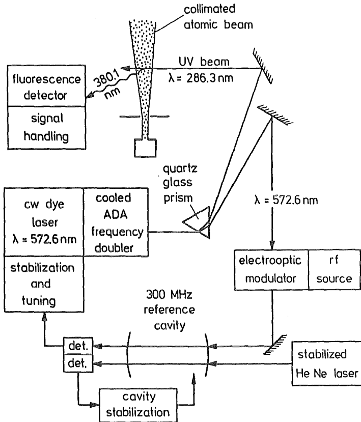
FIG. 1. Schematic diagram of the experimental arrangement.
