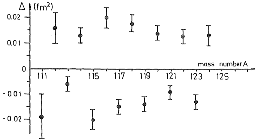
FIG. 5. The odd-even staggering of the mean square charge radii of Sn nuclei as represented by the quantity \Delta as defined by equation (5).
