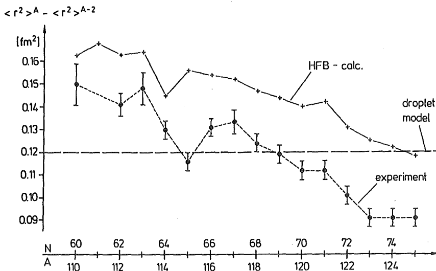
FIG. 4. The differential change \delta \langle r^2 \rangle_{A, A-2} of the mean square charge radii of Sn compared with theoretical results on the basis of the HFB theory. 11 The data for N=60 ( ^{108, 110}\text{Sn} ) were taken from Ref. 20.
