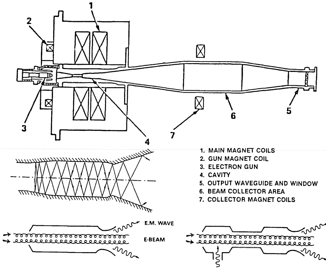
Fig. 1: Schematic of VARIAN CW gyrotron oscillator [4] and scheme of irregular waveguide cavities of gyromonotron oscillator (left) and gyrokylystron amplifier [24].
