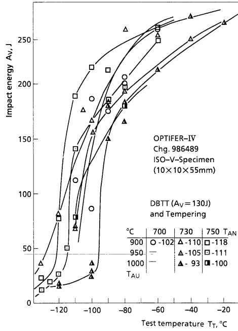
Figure 3: Impact energy of the steel OPTIFER-IV with different thermal treatments in dependence of the test temperature. The best DBTT is -118°C
