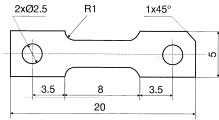
Tensile Test Specimen (0.3 mm thick)
