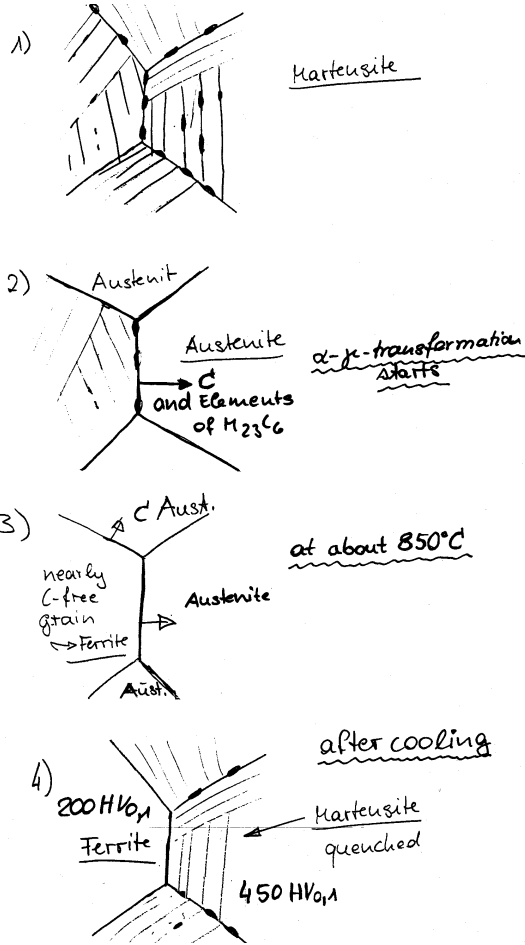
Figure 5: Schematic formation of Ferrite.
