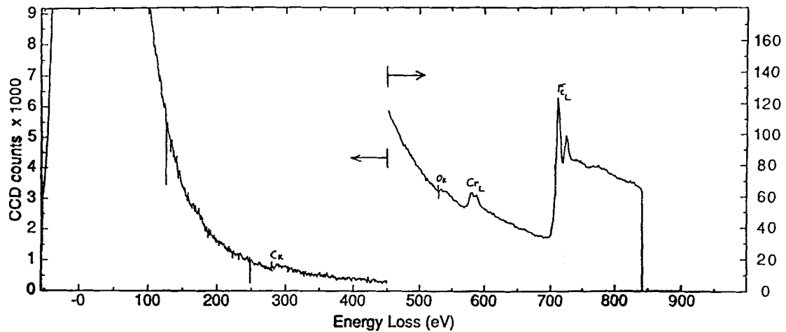
EELS of F82H-mod.
