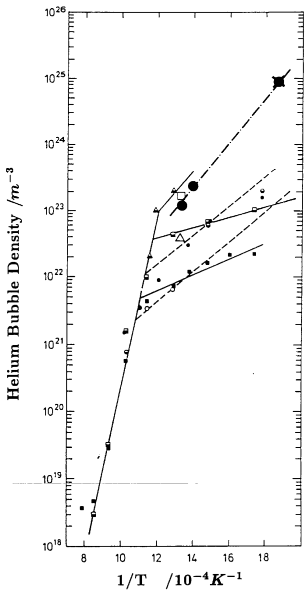
Figure 1: Helium bubble density as a function of reciprocal temperature for different ferritic steels implanted with helium. We show the data compilation by Singh and Trinkaus [1], Dauben et. al [2, 3] and Farrell and Lee [4] together with the present results on the F82H-mod. alloy. It turns out that the helium bubble density is significantly different from one alloy to the another one. ( - . - present results)
