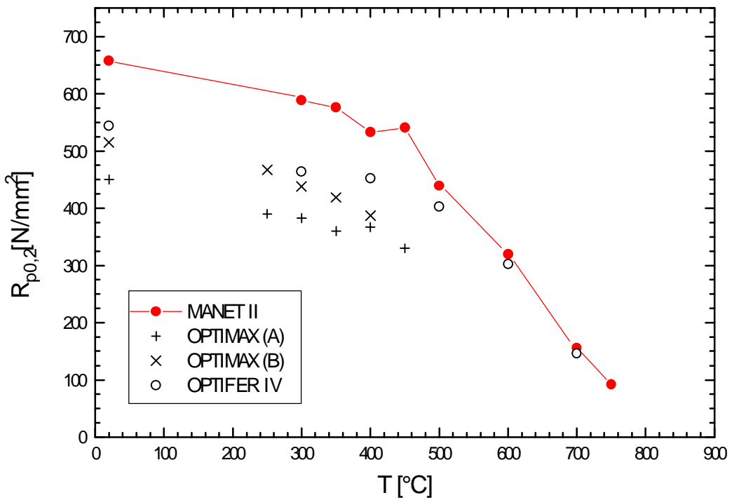
Figure 13: Comparison of the 0.2 % yield strength
