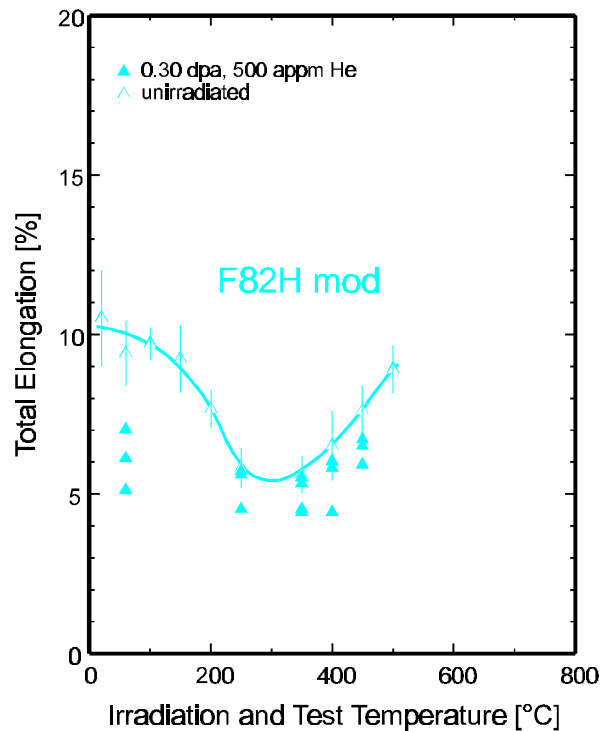
Fig. 4: Total elongation of F82H-mod. specimens after implantation
