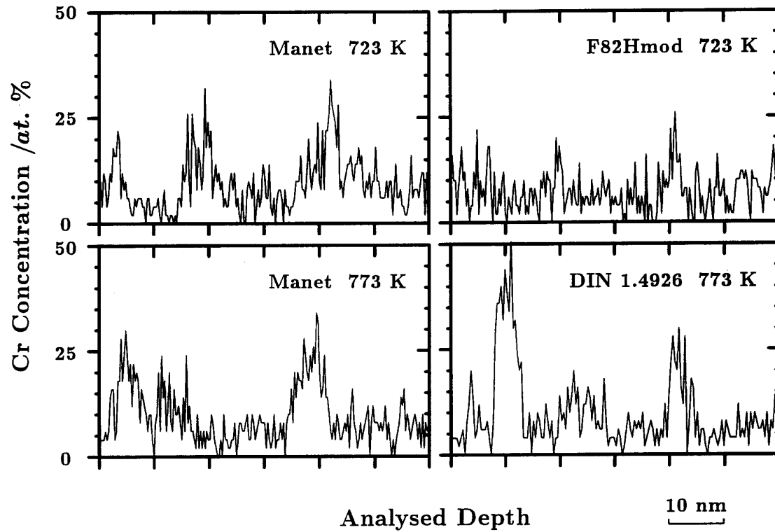
Figure 2: Chromium concentration depth profiles performed by means of atom probing after 300 keV Fe + ion irradiation at a flux of 10 -2 dpa/s to a fluence of 50 dpa and simultaneous implantation of 15 keV He + ions at a rate of 2 appm/s. The nominal chromium concentration varies between 8 and 12 wt.%. All profiles reveal clearly a segregation of chromium.
