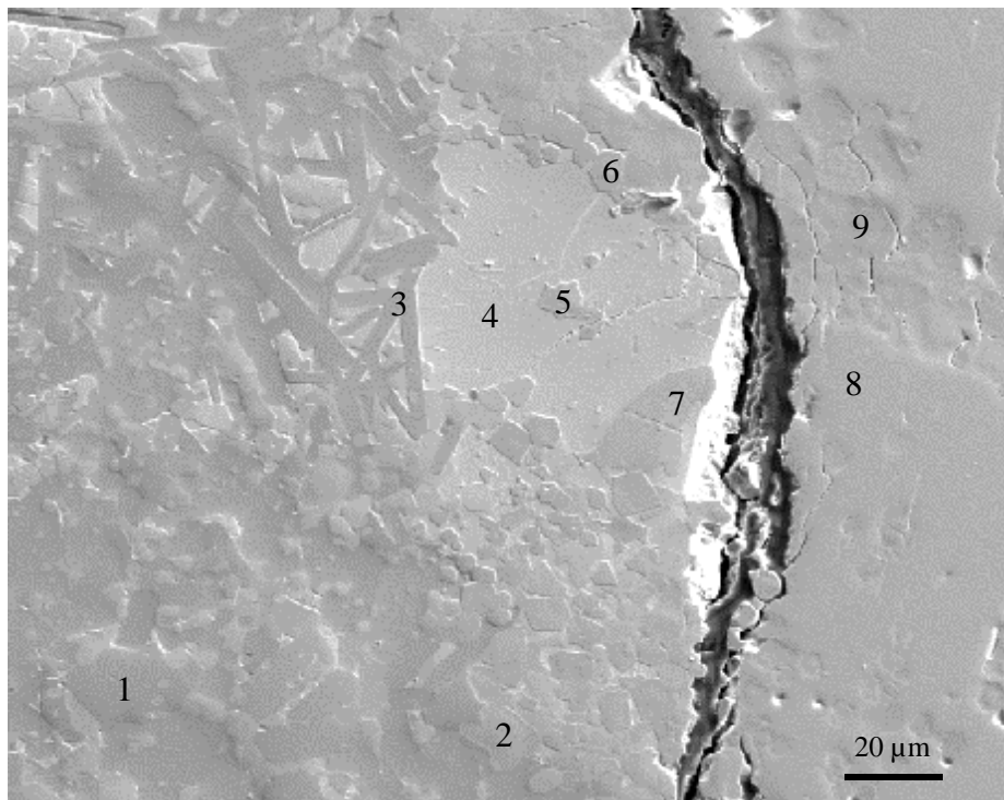
Fig. 4: SEM image of the range near the boundary SS/Zry with Auger measuring points
