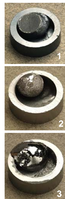
Figure 26: Pre-tests for preparation of absorber melts using stacks of thin slices of the starting materials. Good results were obtained at 1800 and 1900 °C.
