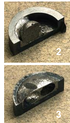
Figure 25: Pre-tests for preparation of absorber melts using powder mixtures. The specimens were either incompletely molten or had large voids.
