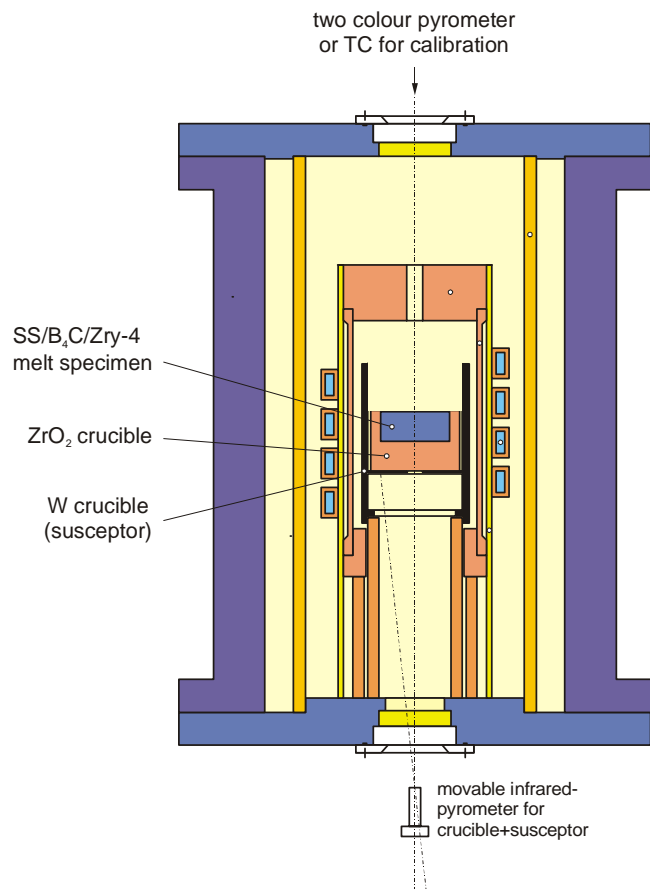
Figure 4: LAVA apparatus for the preparation of absorber melts
