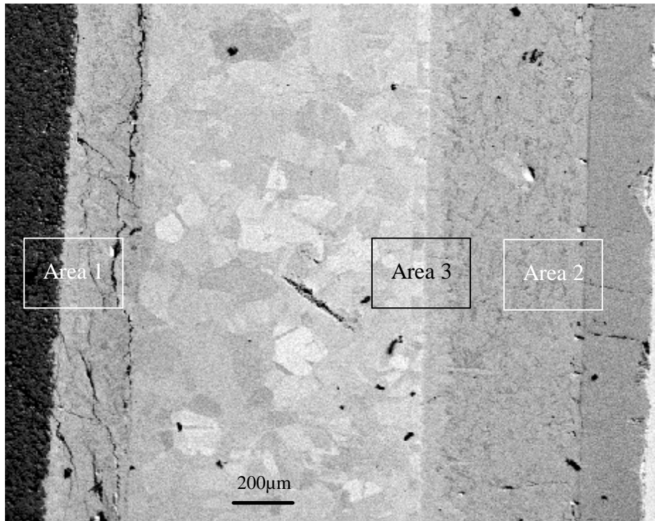
Fig. 1: Cross section through a CR segment after test at 1200 °C, left: B 4 C, right: ZrO 2 with indicated areas for detailed Auger analyses
