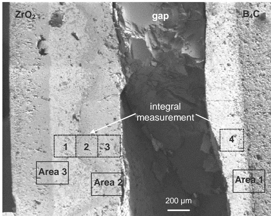
Fig. 1: Cross section through a CR segment after 1 h isothermal test at 1400 °C in argon/steam atmosphere; left: ZrO 2 scale, right: B 4 C pellet; areas for detailed analyses are indicated in black; areas for integral analyses of the melt in white
