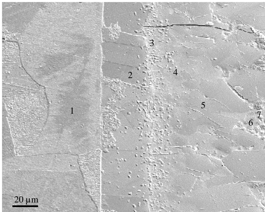
Fig. 6: SEM image of an area at the boundary SS/Zry-4 with Auger measuring points
