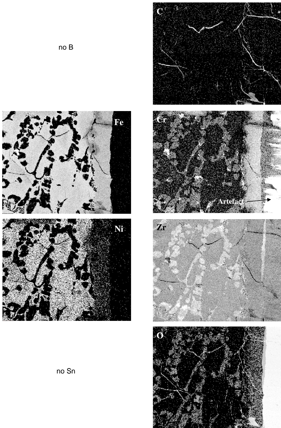
Fig. 5 a-h: Element mapping near outer ZrO 2 scale (see Fig. 4)
