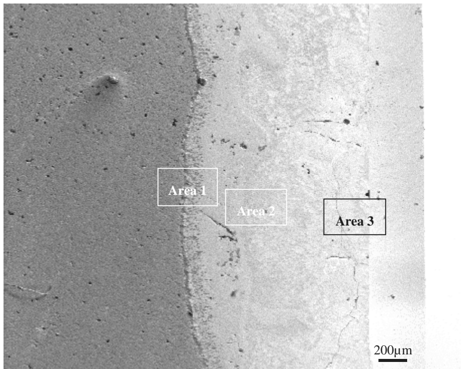
Fig1: Cross section through a CR segment after test at 1400 °C, left: B_4C , right: ZrO_2 with indicated areas for detailed Auger elemental analyses
