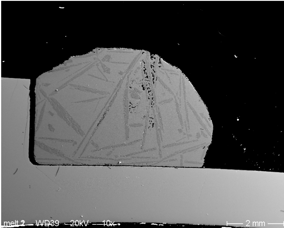
Melt 2: 95 % SS, 5 % B4C after preparation
