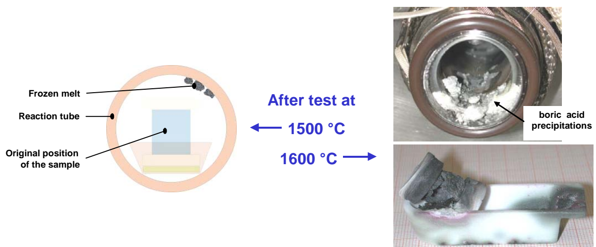
Figure 16: Post-test appearance of furnace and specimens after failure of the control rod segments during tests at high temperatures, showing results of rapid reactions with melt splashing in the reaction tube, relocation of the specimen during the test, and huge precipitations of boric acids at the outlet of the reaction tube flange.
