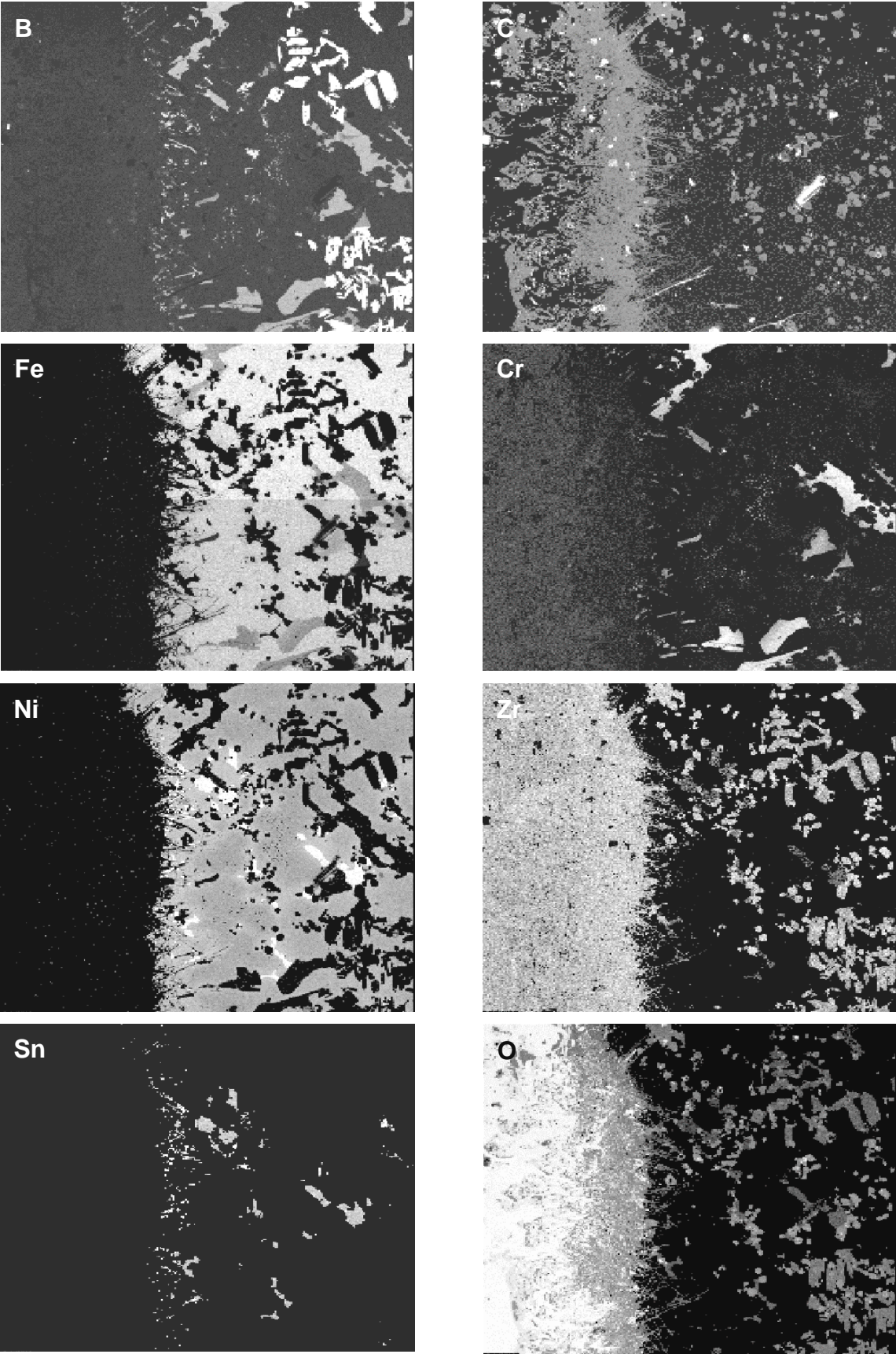
Fig. 8: Auger element mapping of the area near the external ZrO 2 scale (see Fig. 7)
