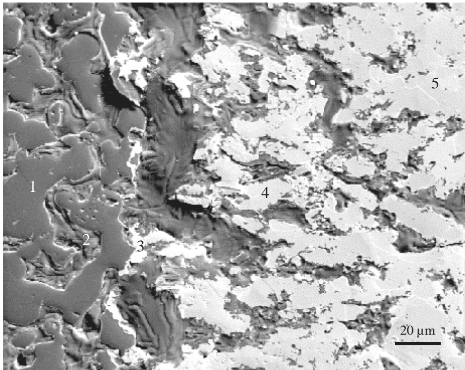
Fig. 2 : SEM image of the range near B 4 C with Auger measuring points
