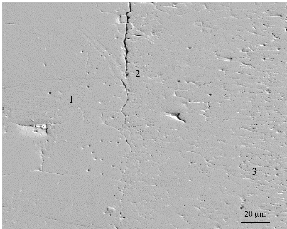
Fig. 6: SEM image of the range near the outer ZrO 2 scale with Auger measuring points
