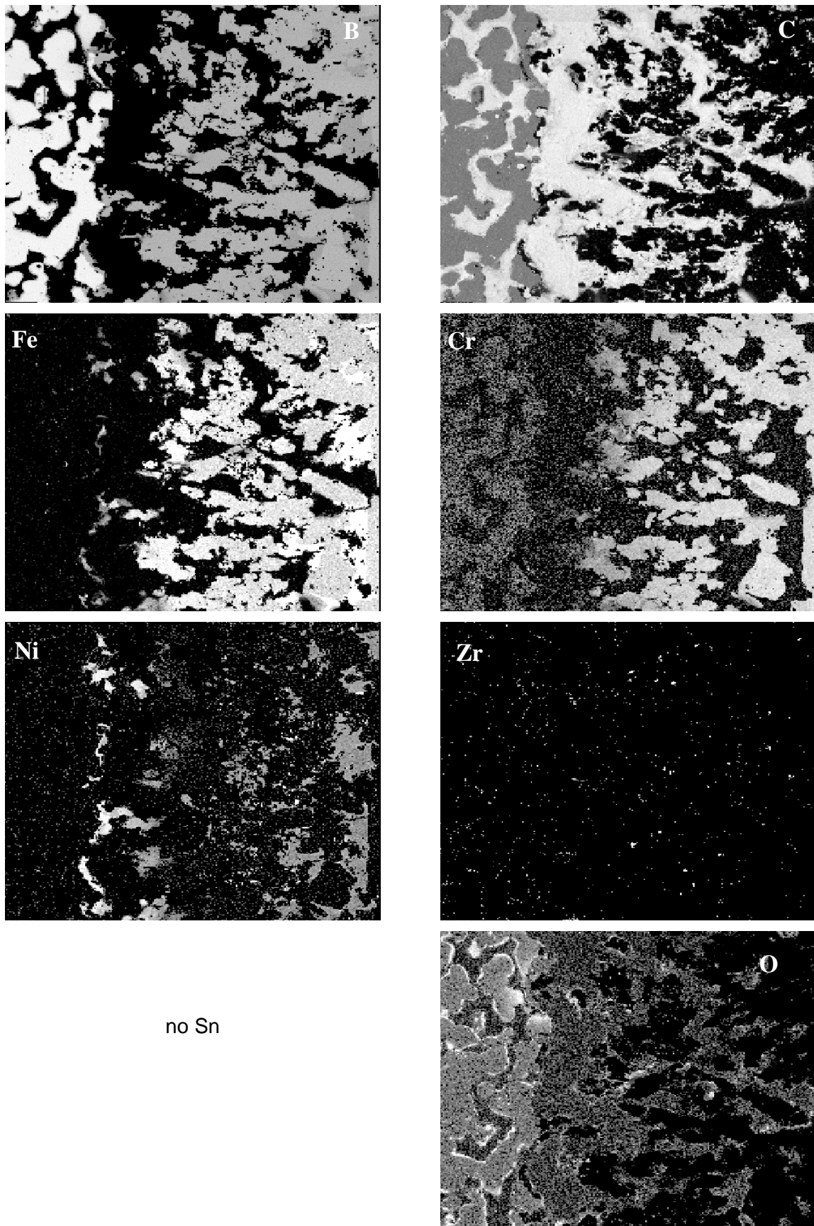
Fig. 3 a-h: Element mapping near B 4 C (see Fig. 2)
