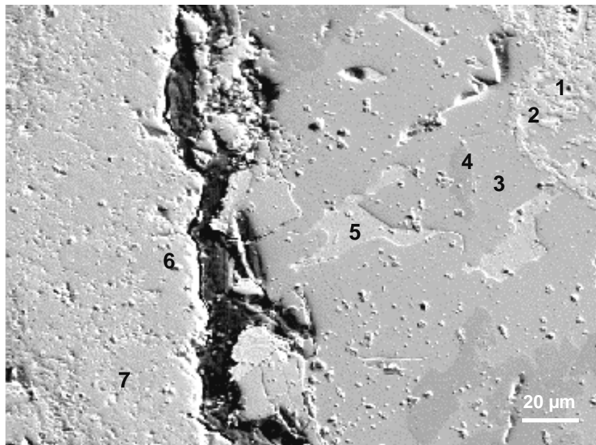
Fig. 6: SEM Image of the area near ZrO_2 scale with Auger measuring points
