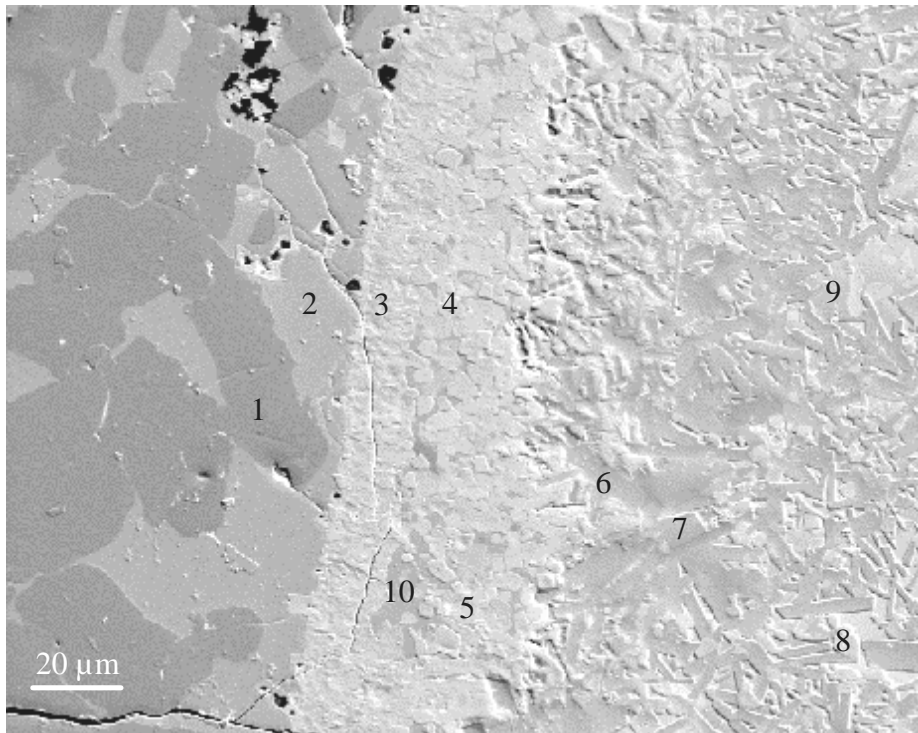
Fig. 4 : SEM image of the molten SS/Zry range with Auger measuring points
