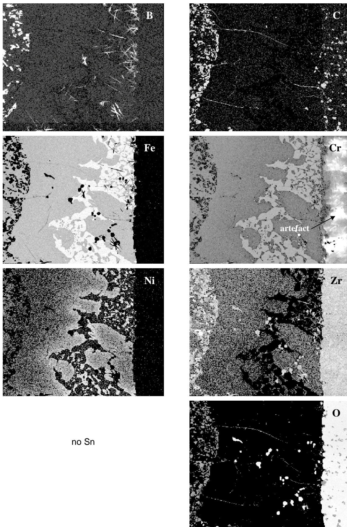
Fig. 7 a-h: Element mapping near outer ZrO_2 scale (see Fig. 6)
