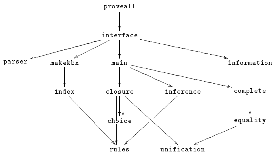
Figure 4.1: Dependency graph for the modules of \mathcal{Z}TP 's core.
