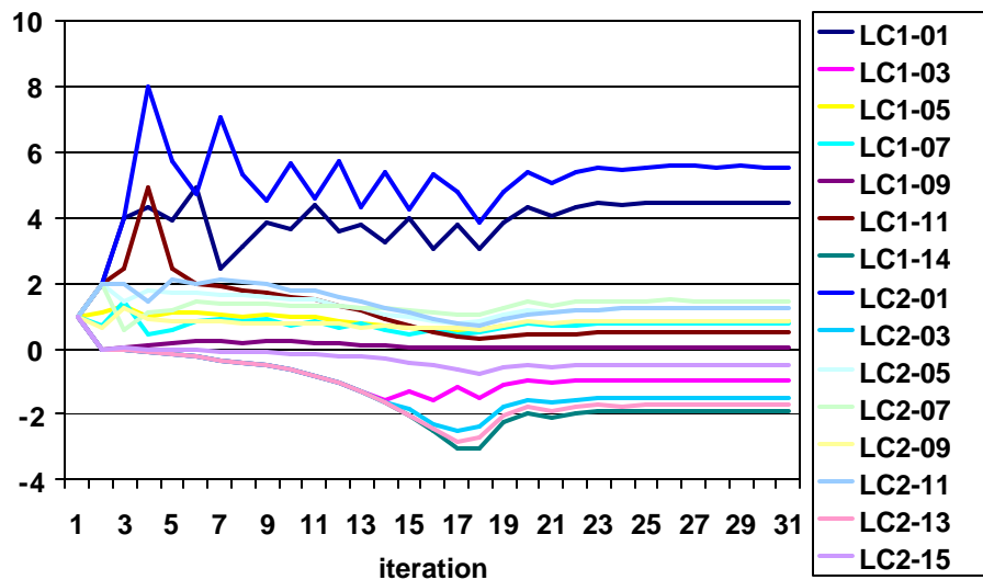
Figure 19: Examples of the design variable histories for the optimisation
